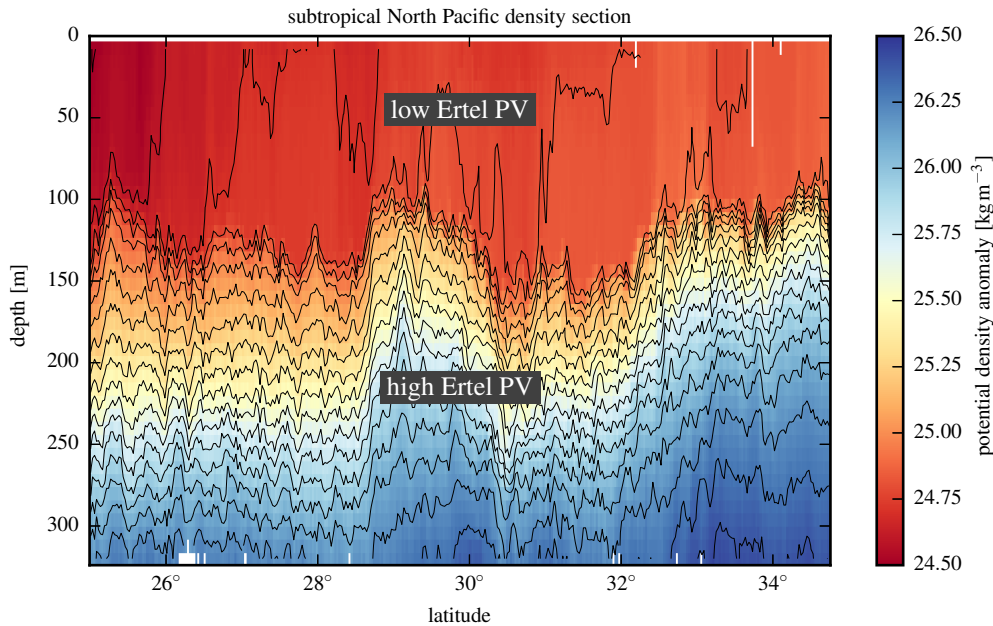
FIGURE 1. Potential density section from the wintertime eastern subtropical North Pacific. The data were obtained using a conductivity–temperature–depth sensor towed on a sawtooth profile along 140^\circ\text{W} as part of the Spice experiment on Jan. 28 to Feb. 2, 1997. For more information on the data, see Ferrari & Rudnick (2000).
