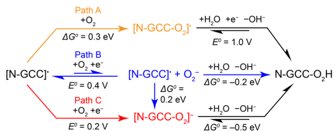
Scheme 2. Computed thermochemistry of various pathways for \text{O}_2 activation by \text{N}^+\text{-GCC} active sites. The putative rate-limiting step(s) in each sequence are denoted with irreversible reaction arrows.
