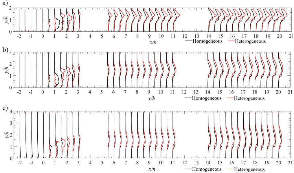
FIGURE 9. Turbulent kinetic energy profiles TKE at (a) H/h = 2 , (b) H/h = 3 , and (c) H/h = 4 . The homogeneous canopy is shown in black and the heterogeneous in red.
