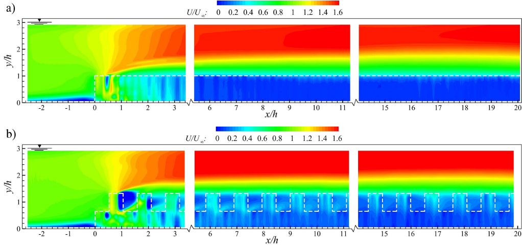
FIGURE 3. Time-averaged streamwise velocity fields U(x,y)/U_\infty at submergence H/h = 3 for the a) homogeneous and b) heterogeneous canopies. White dashed lines indicate the envelope of the canopies, and the symbol at the top left shows the free surface. The three panels correspond to the three fields of view (FOV) for the PIV.
