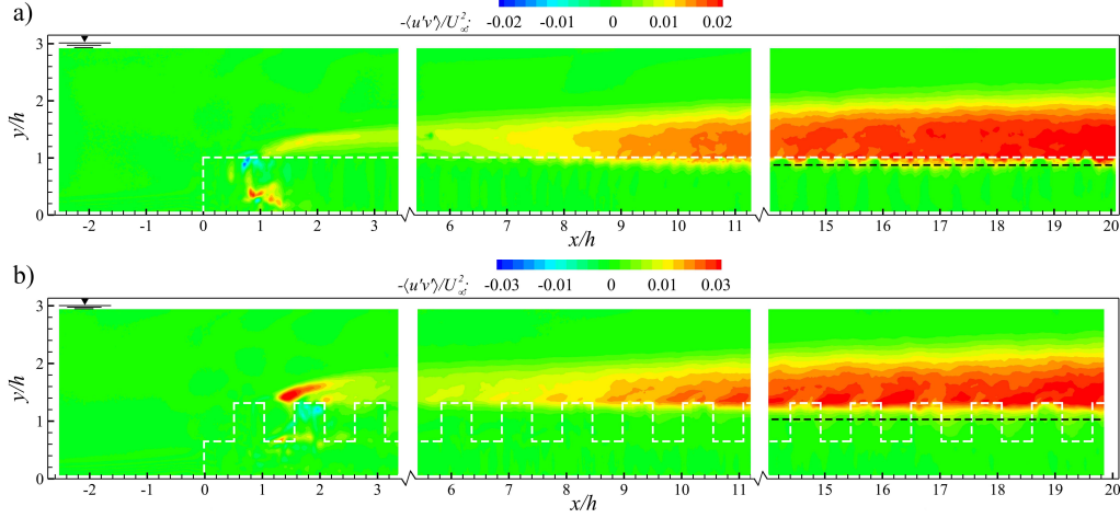
FIGURE 10. Reynolds shear stress fields -\langle u'v' \rangle / U_\infty^2 at submergence H/h = 3 for the a) homogeneous and b) heterogeneous canopies. White dashed lines illustrate the envelope of the canopies, and the symbol at the top left shows the free surface. The black dashed lines indicate the penetration depths \delta_e (equation 3.5).
