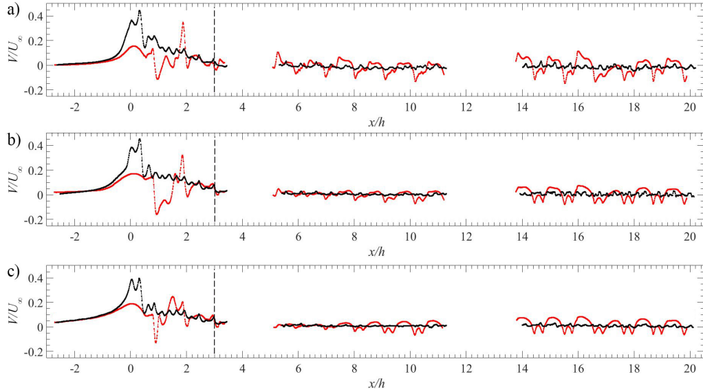
FIGURE 6. Time-averaged vertical velocity profiles V(x, y = h)/U_\infty at various submergences for the homogeneous (black) and heterogeneous (red) canopies. a) H/h = 2 ; b) H/h = 3 ; c) H/h = 4 .
