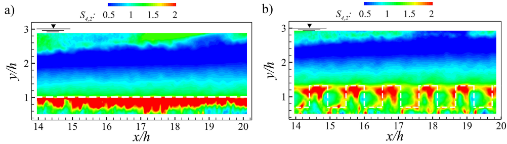
FIGURE 15. The ratio of the total contribution of sweep to ejection events S_{4,2} = \sum u'v'_4 / \sum u'v'_2 at H/h = 3 for the a) homogeneous and b) heterogeneous canopies.
