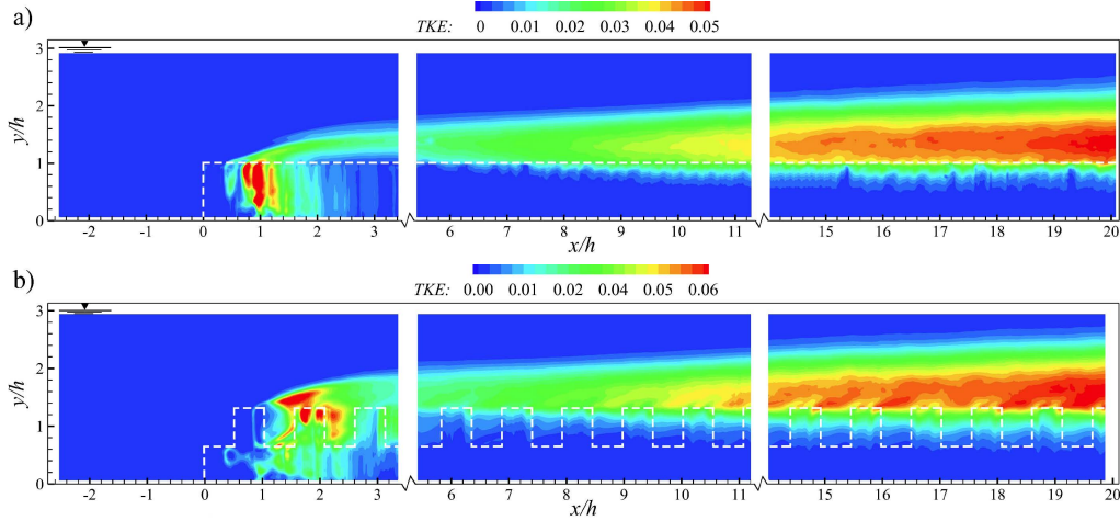
FIGURE 8. Turbulent kinetic energy fields TKE = \langle u'^2 + v'^2 \rangle / 2U_\infty^2 at submergence H/h = 3 for the a) homogeneous and b) heterogeneous canopies. White dashed lines indicate the envelope of the canopies, and the symbol at the top left shows the free surface.
