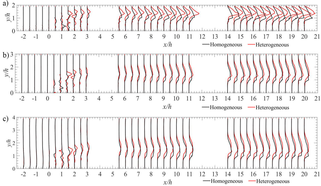
FIGURE 11. Reynolds shear stress profiles -\langle u'v' \rangle / U_\infty^2 at a) H/h = 2 , b) H/h = 3 , and c) H/h = 4 . The homogeneous canopy is shown in black and the heterogeneous in red.
