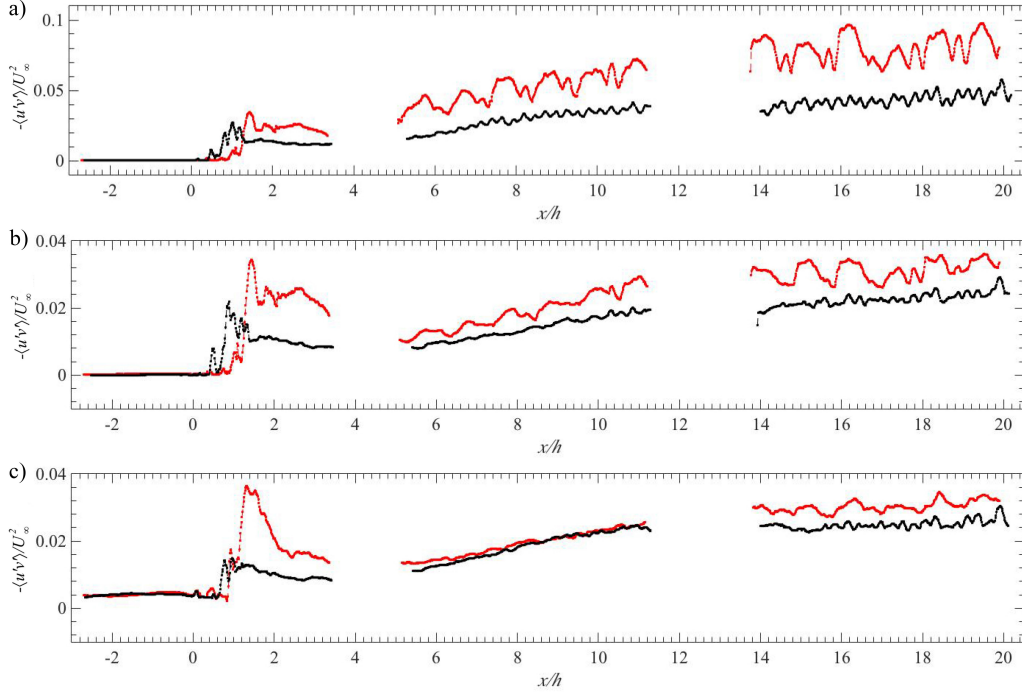
FIGURE 12. Maximum Reynolds shear stress -\langle u'v' \rangle / U_\infty^2 as a function of downstream distance: (a) H/h = 2 , (b) H/h = 3 , (c) H/h = 4 . Homogeneous canopy in black and heterogeneous in red.
