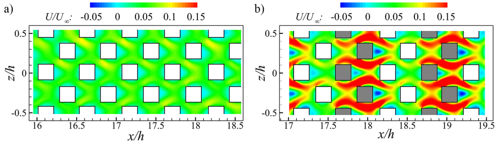
FIGURE 7. Time-averaged streamwise velocity fields U(x, z)/U_\infty at y/h \simeq 0.6 and H/h = 3 for the a) homogeneous and b) heterogeneous canopies, elements of height h_1 are shaded.
