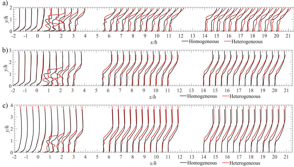
FIGURE 4. Time-averaged streamwise velocity profiles U(y)/U_\infty at various x/h locations and submergences for the homogeneous (black) and heterogeneous (red) canopies. a) H/h = 2 ; b) H/h = 3 ; c) H/h = 4 .
