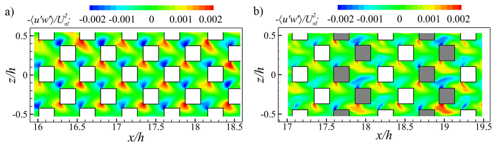
FIGURE 16. Reynolds shear stress -\langle u'w' \rangle / U_\infty^2 at y/h \simeq 0.6 and H/h = 3 for the a) homogeneous and b) heterogeneous canopies, elements of height h_1 are shaded.
