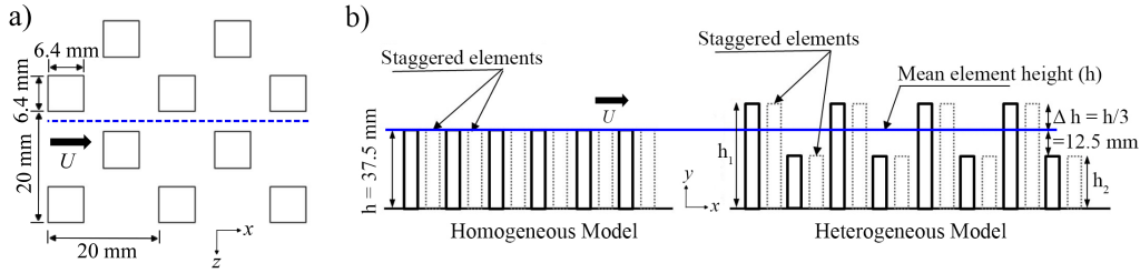
FIGURE 1. Homogeneous and heterogeneous canopy models. (a) plan view of the models with element spacing and geometry, the dashed line marks the location of the streamwise wall-normal ( x - y ) measurement plane. (b) schematic highlighting the elements height for both models ( h = 37.5 mm, h_1 = 50 mm, h_2 = 25 mm).
