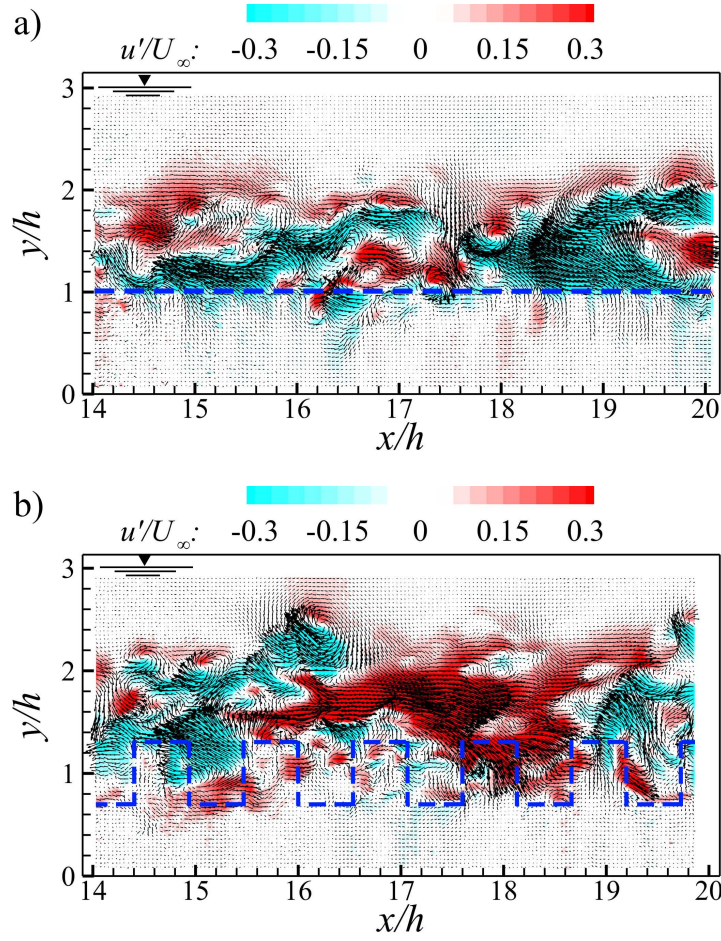
FIGURE 14. An instantaneous velocity fluctuation vector field u'\hat{i} + v'\hat{j} superimposed on the contours of u'/U_\infty at submergence H/h = 3 for the a) homogeneous and b) heterogeneous canopies.
