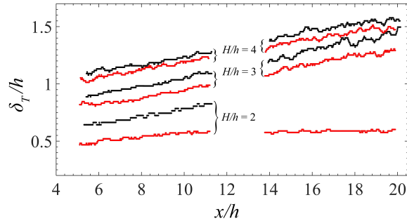
FIGURE 13. Extension of mixing layer \delta_T/h above the homogeneous (black) and heterogeneous (red) canopies at the three submergence depths.
