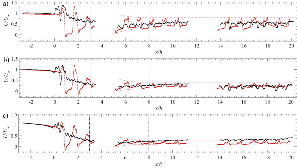
FIGURE 5. Time-averaged streamwise velocity profiles U(x, y = h)/U_\infty at various submergences for the homogeneous (black) and heterogeneous (red) canopies. a) H/h = 2 ; b) H/h = 3 ; c) H/h = 4 .
