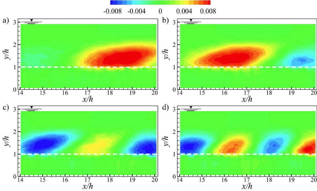
FIGURE 17. POD modes of the streamwise velocity fluctuations \phi_{u'} for the homogeneous canopy at H/h = 3 : a) mode 1, b) mode 2, c) mode 3, d) mode 4.
