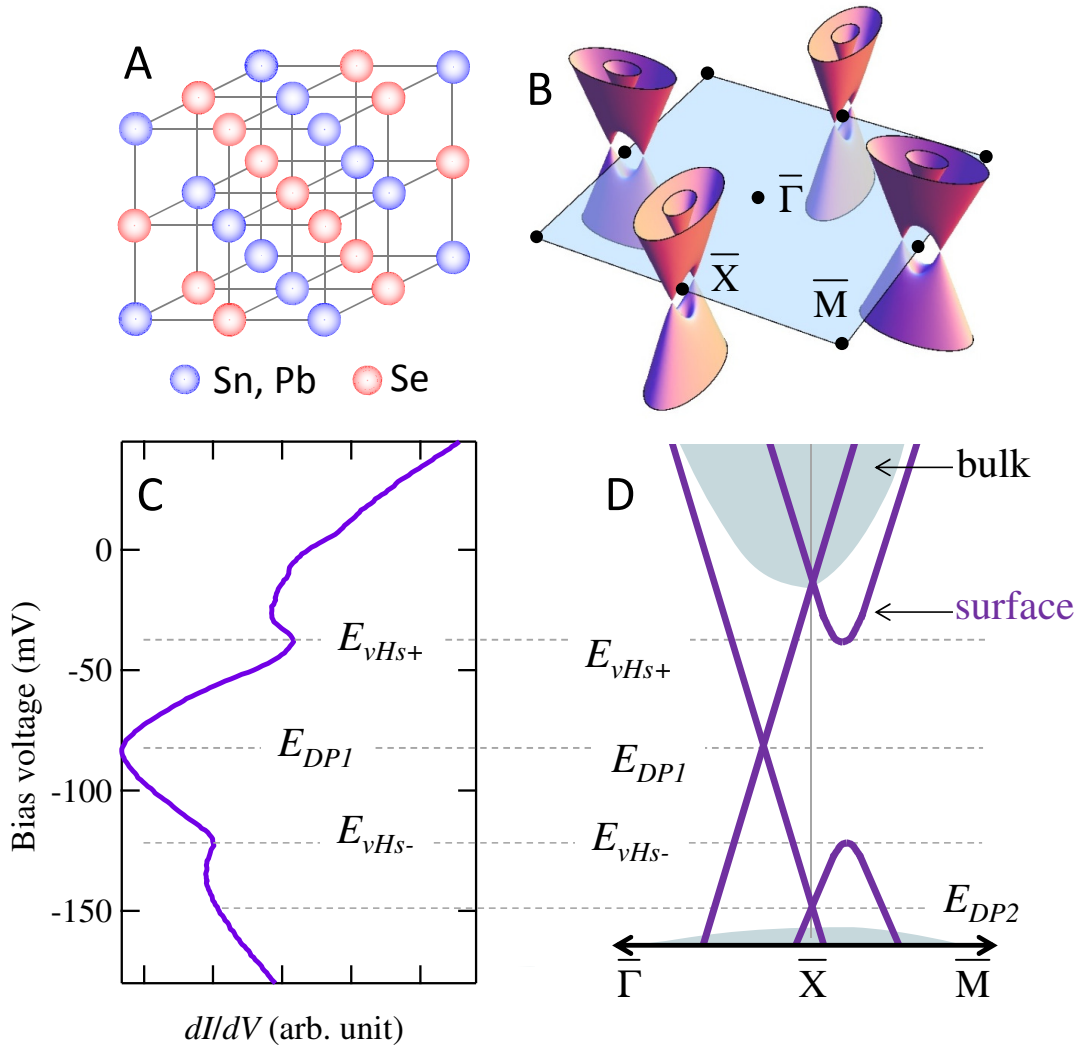
Fig. 1. Crystal structure and schematic band structure of TCIs. (A) Schematic crystal structure of Pb_{1-x}Sn_xSe . The top view reflects the [001] plane, which is the surface seen in STM. The Sn and Pb atoms are expected to be randomly distributed at the blue sites. (B) Schematic band structure of the surface state showing the surface Brillouin zone as a blue plane and the four pairs of Dirac nodes, each centered at the X point in momentum space. (C) Typical average dI/dV spectrum in zero field. (D) Schematic cuts along two high symmetry directions showing the surface state dispersion of one of the Dirac cones as well as the four important energy scales E_{DP1} , E_{vH+} , E_{vHs-} , and E_{DP2} representing the Dirac point associated with the primary Dirac node, the two Van Hove singularities associated with the saddle points in the dispersion, and the Dirac point energy associated with the secondary Dirac node respectively.
