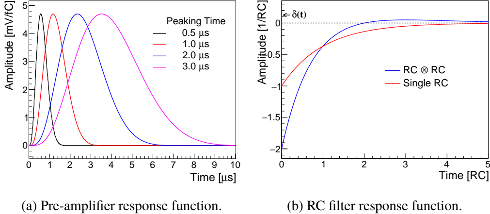
Figure 6: MicroBooNE pre-amplifier electronics impulse response functions are shown for (a) four peaking time settings at 4.7 mV/fC gain and (b) a single RC filter and two independent RC filters ( RC \otimes RC ).
