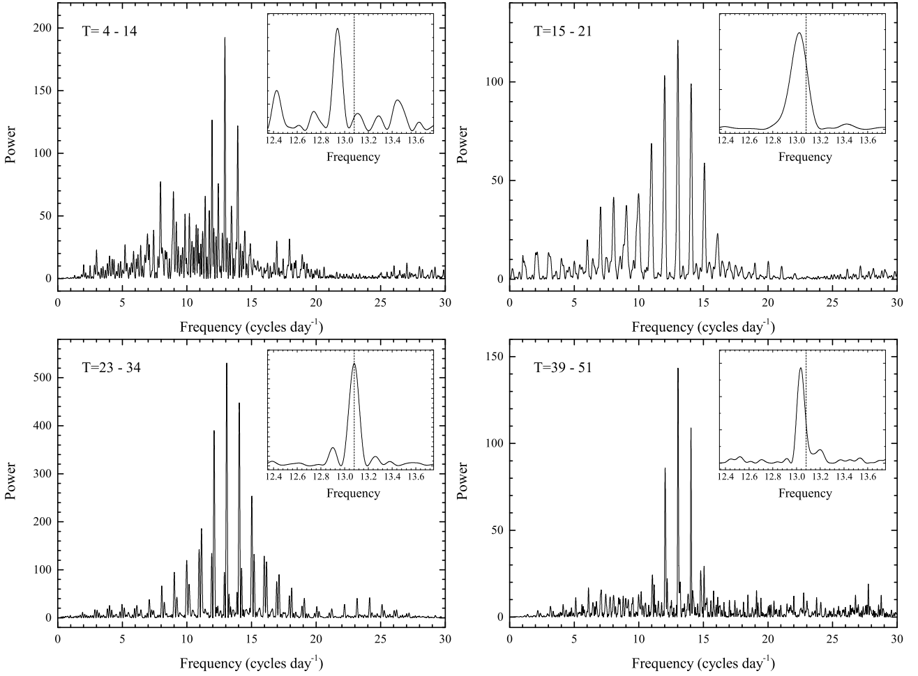
Figure 7. Lomb–Scargle periodograms of the V data combined among T=4-14 , 15-21 , 23-34 and 39-51 . The inset shows the enlarged region around the frequency 13.08 \text{ cycle d}^{-1} – the averaged frequency of superhumps during the superoutburst stage B, marked by the vertical dashed line.
