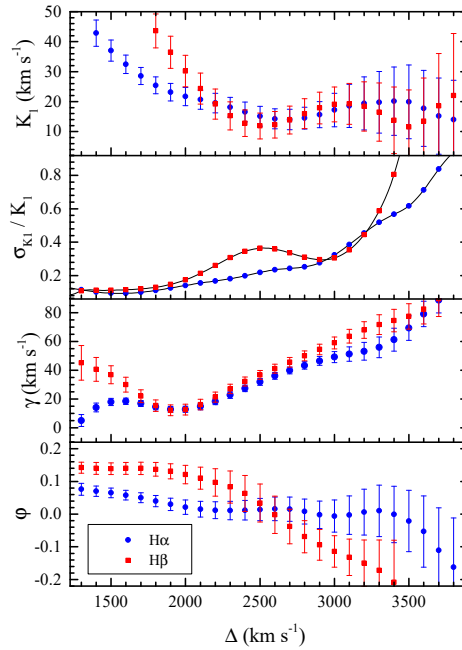
Figure 16. The diagnostic diagram for the H \alpha and H \beta emission lines from the T=72 observations, showing the response of the fitted orbital elements to the choice of the double-Gaussian separation.
