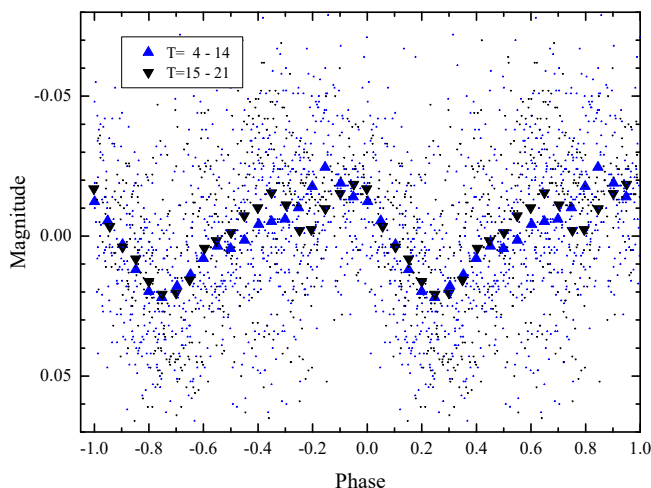
Figure 12. The V light curves from the time intervals T=4-14 and 15-21 folded with the period of 180.48 min and averaged in 20 phase bins. The small and large symbols represent the individual observations and the data averaged in 20 phase bins, respectively. All data are plotted twice for continuity.
