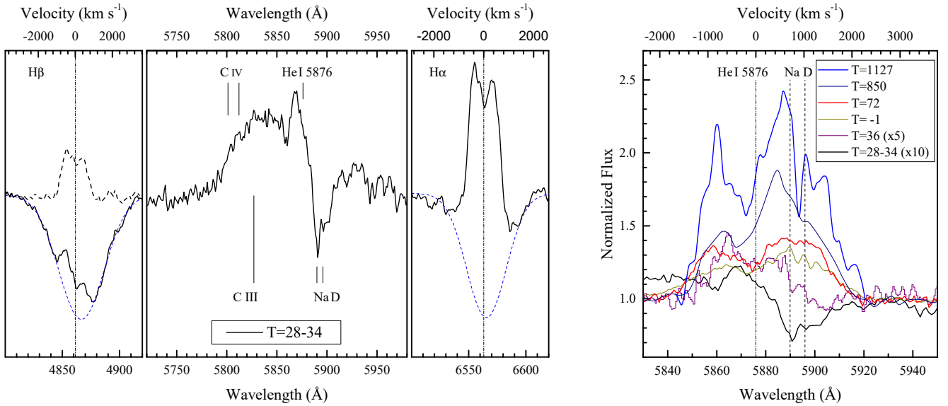
Figure 14. Left: H\alpha and H\beta line profiles and the region around the C\text{ III} / C\text{ IV} / \text{He I } \lambda 5876 / \text{Na D} complex (black solid line) during the plateau stage of the superoutburst (arbitrary scaling). The dashed blue line shows a Gaussian fit to the absorption components of H\alpha and H\beta . The dashed black line shows the profile of H\beta after being corrected for absorption. Right: \text{He I } \lambda 5876 and \text{Na D} line profiles from different data sets, shown in actual scale (for a better comparison, the T=28-34 and 36 profiles have been multiplied by a factor of 10 and 5, respectively).
