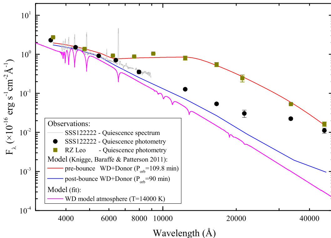
Figure 18. Theoretical SEDs of pre- and post-bounce CVs, based on the models of Knigge, Baraffe, & Patterson (2011) , shown together with the photometric and spectroscopic data of SSS J122222 and RZ Leo in quiescence (see text for details).
