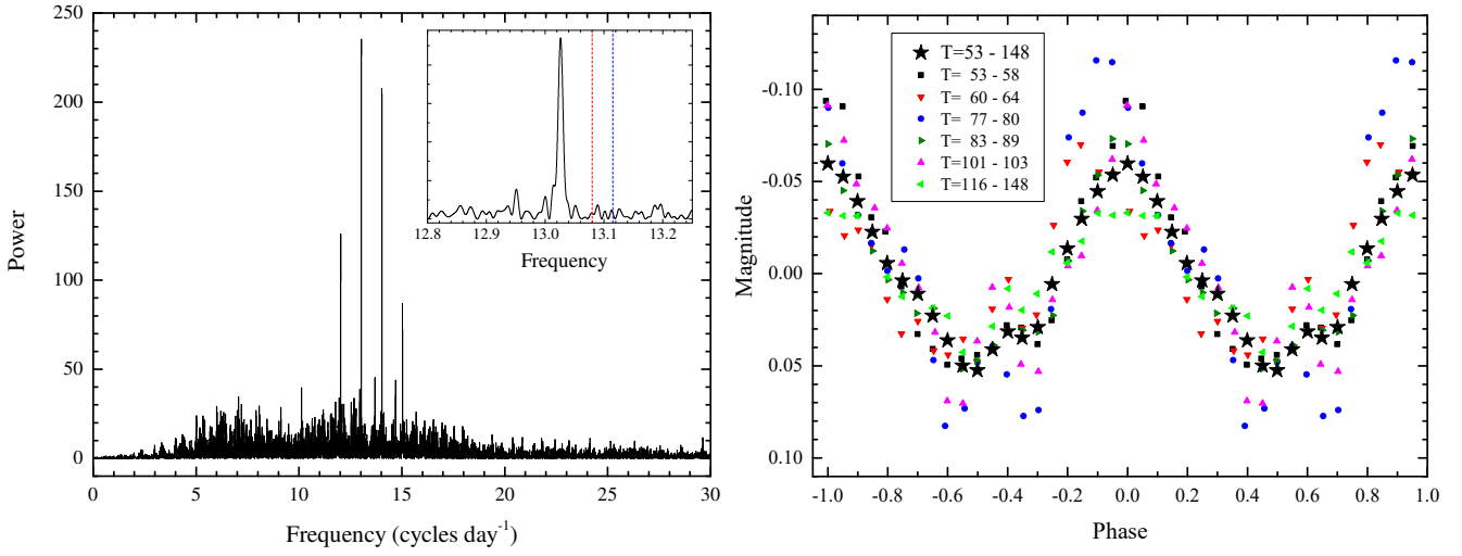
Figure 10. Left: Lomb–Scargle periodogram of the V data combined between T=53 and 148. The inset shows the enlarged region around the frequency 13.026 cycle d^{-1} – the frequency of post-superoutburst modulations observed in 2013. The vertical dashed lines mark the orbital (blue) and stage B superhump (red) frequencies of 13.11 and 13.08 cycle d^{-1} , respectively. Right: the entire set (large stars) and short subsets (small symbols) of the V data between T=53 and 148, folded according to ephemeris HJD_{max} = 245\,6300.0610(3) + 0.07676887(5) \cdot E .
