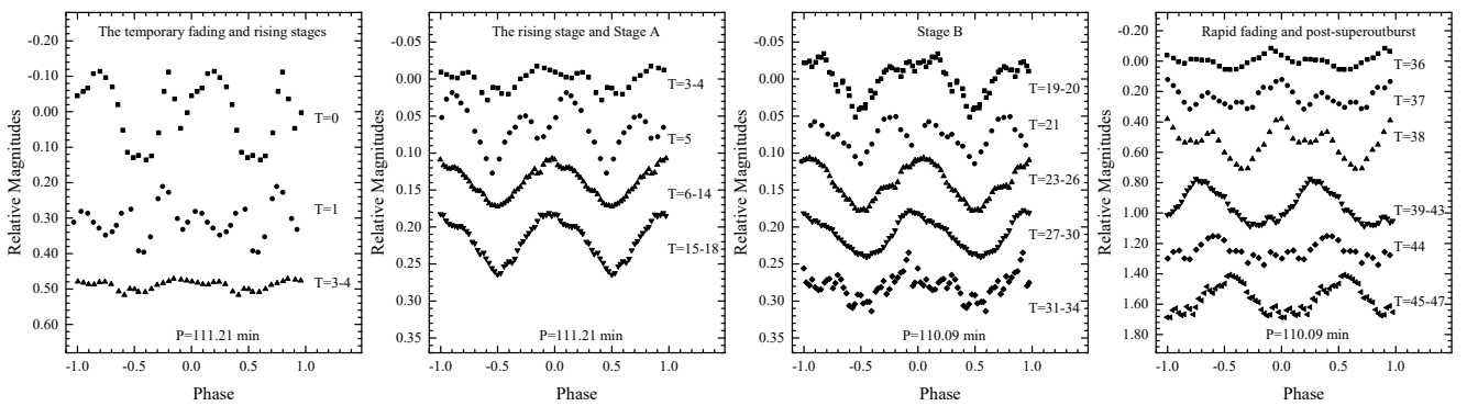
Figure 8. Variation of superhump profiles during the superoutburst of SSS J122221.
