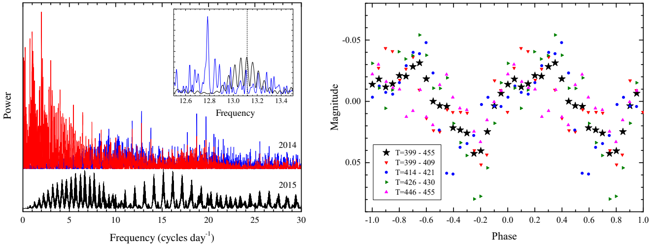
Figure 10. Left: Lomb–Scargle periodogram of the V data combined between T=53 and 148. The inset shows the enlarged region around the frequency 13.026 cycle d^{-1} – the frequency of post-superoutburst modulations observed in 2013. The vertical dashed lines mark the orbital (blue) and stage B superhump (red) frequencies of 13.11 and 13.08 cycle d^{-1} , respectively. Right: the entire set (large stars) and short subsets (small symbols) of the V data between T=53 and 148, folded according to ephemeris HJD_{max} = 245\,6300.0610(3) + 0.07676887(5) \cdot E .
