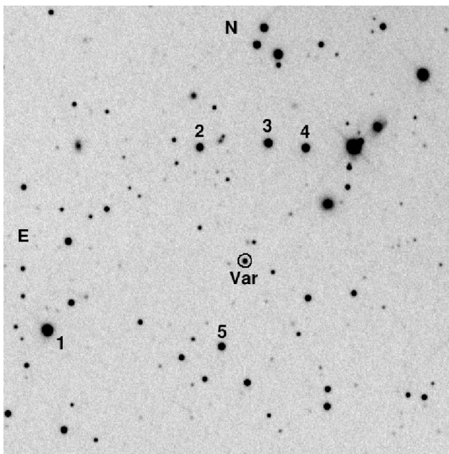
Figure A1. The 6' \times 6' field of view of SSS J122222, oriented such that up is North and left is East. The object's location is indicated by a ring. Calibrated comparison stars are labelled as 1, 2, 3, 4 and 5, and their magnitudes are listed in Table A1.
