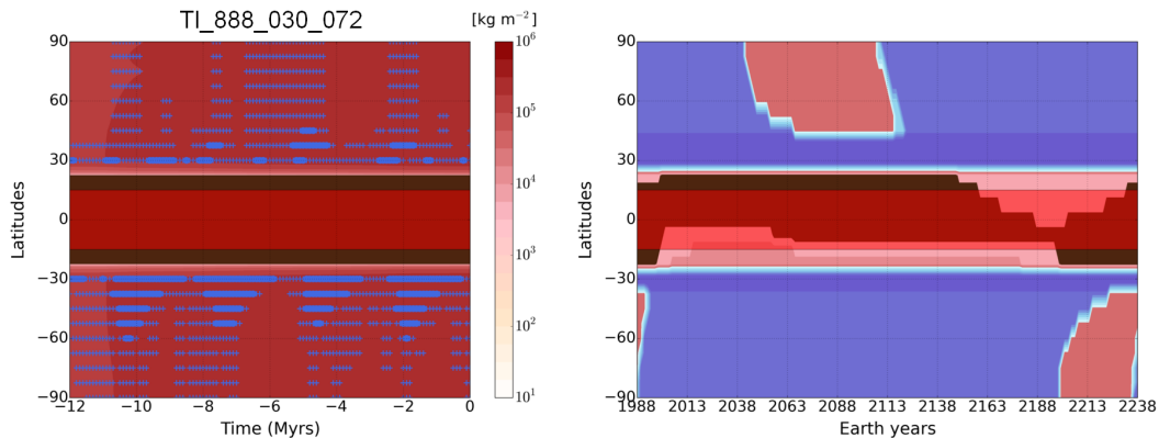
Fig. 6. Simulation #TI888_030_072. Same as Figure 4 and Figure 5 (legends are the same), except for an equatorial \text{CH}_4 ice albedo of 0.3 (very dark BTM).
