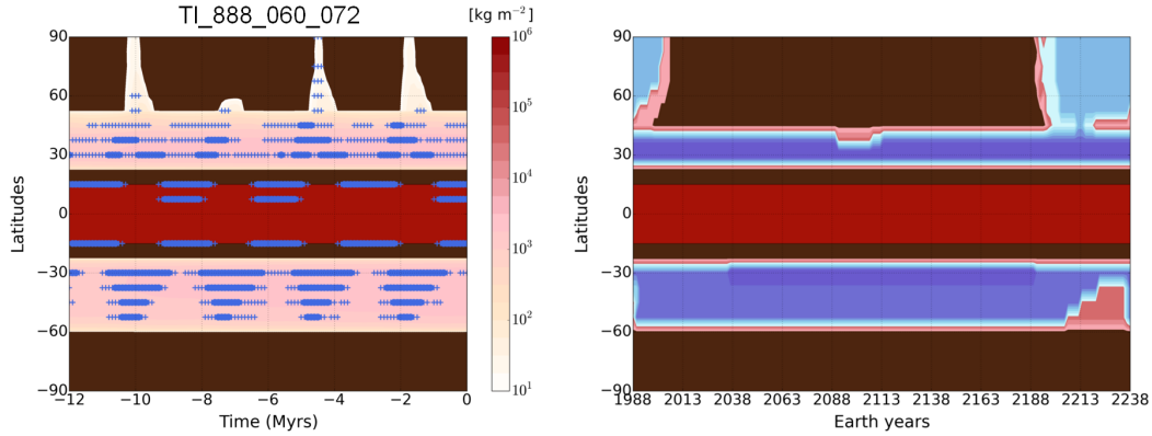
Fig. 7. Simulation #TI888_060_072. Same as Figure 4 and Figure 5, except for an equatorial \text{CH}_4 ice albedo of 0.60 (relatively bright BTD).
