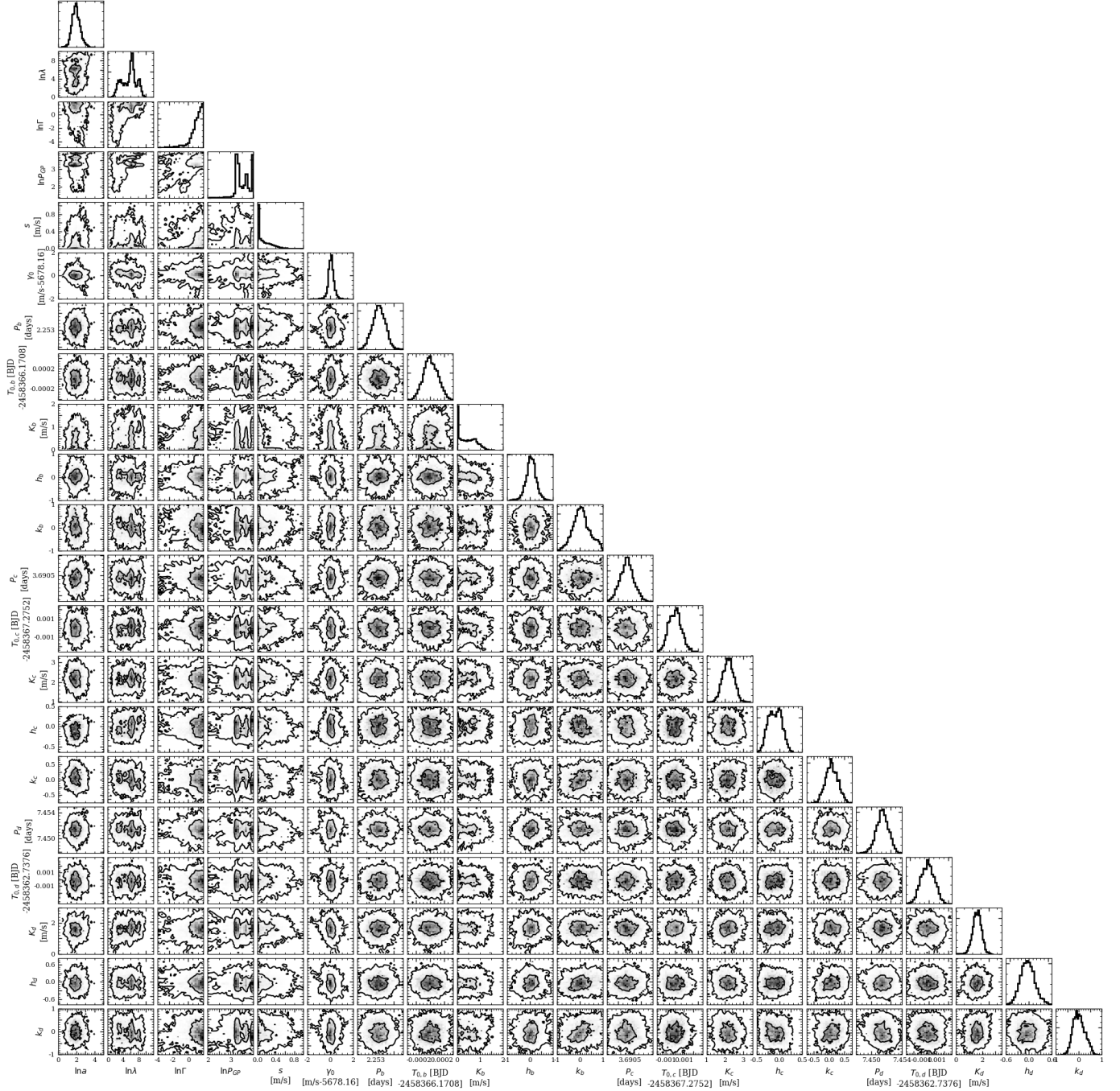
Fig. A.1. Marginalized and joint posterior probability density functions of the model parameters from the RV analysis. The adopted RV model includes a trained GP activity model ( \{\ln a, \ln \lambda, \ln \Gamma, \ln P_{\text{GP}}, s\} ) plus the star's systemic velocity ( \{\gamma_0\} ) and three Keplerian planet solutions ( \{P_i, T_{0,i}, K_i, h_i, k_i\} for i = b, c, d ).
