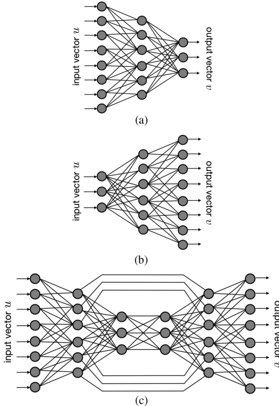
Fig. 4. Simplified schematics of layer width progression strategies for DNNs. (a) Contracting architecture. (b) Expanding architecture. (c) Encoder–decoder architecture.
