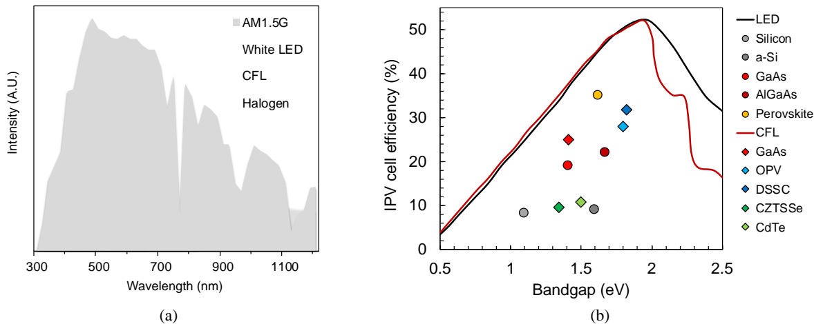
Figure 5: (a) Outline of the different light spectra under which photovoltaic device efficiency is evaluated including the standard solar spectrum (AM1.5G) and typical spectra from White LED, CFL and Halogen sources. (b) The maximum efficiencies versus bandgap measured for indoor photovoltaic devices to date where circles represent measurements under LED bulbs and diamonds under CFL illumination [2], [14], [28]–[31]. Also shown are the maximum theoretical efficiencies calculated in [26] using the detailed balance limit of efficiency method considering an LED spectrum (black line) and a CFL spectrum (red line).
