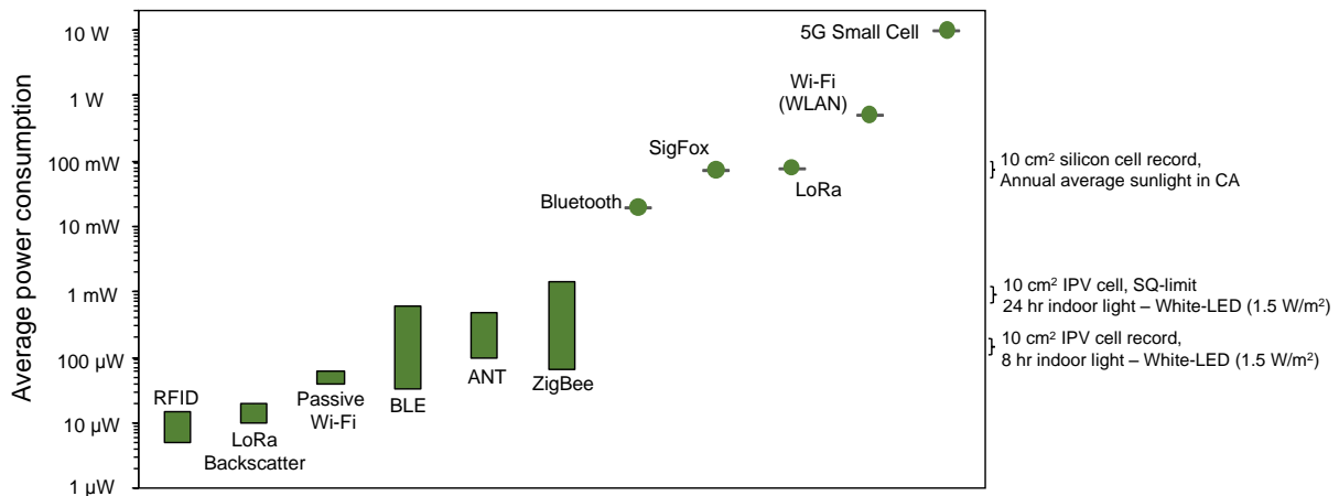
Figure 3: A comparison between the average power consumption of wireless protocols with the average power produced by PV cells of different efficiencies under some example lighting conditions. Power consumption values are taken from the measured and expected values for numerous backscatter and active radio nodes in [12], measurements taken by Dementyev et al. for RFID, BLE, ANT and ZigBee [15] protocols under various communication ranges and frequencies and the expected power requirements for future 5G small cells as in [16].
