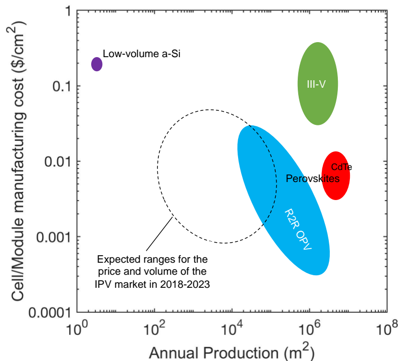
Figure 6: Predicted solar module manufacturing cost versus the scale of production (m 2 /year) for multiple cell types and manufacturing processes [40]–[52]. Also indicated by the shaded region is the expected volume and maximum price point for
