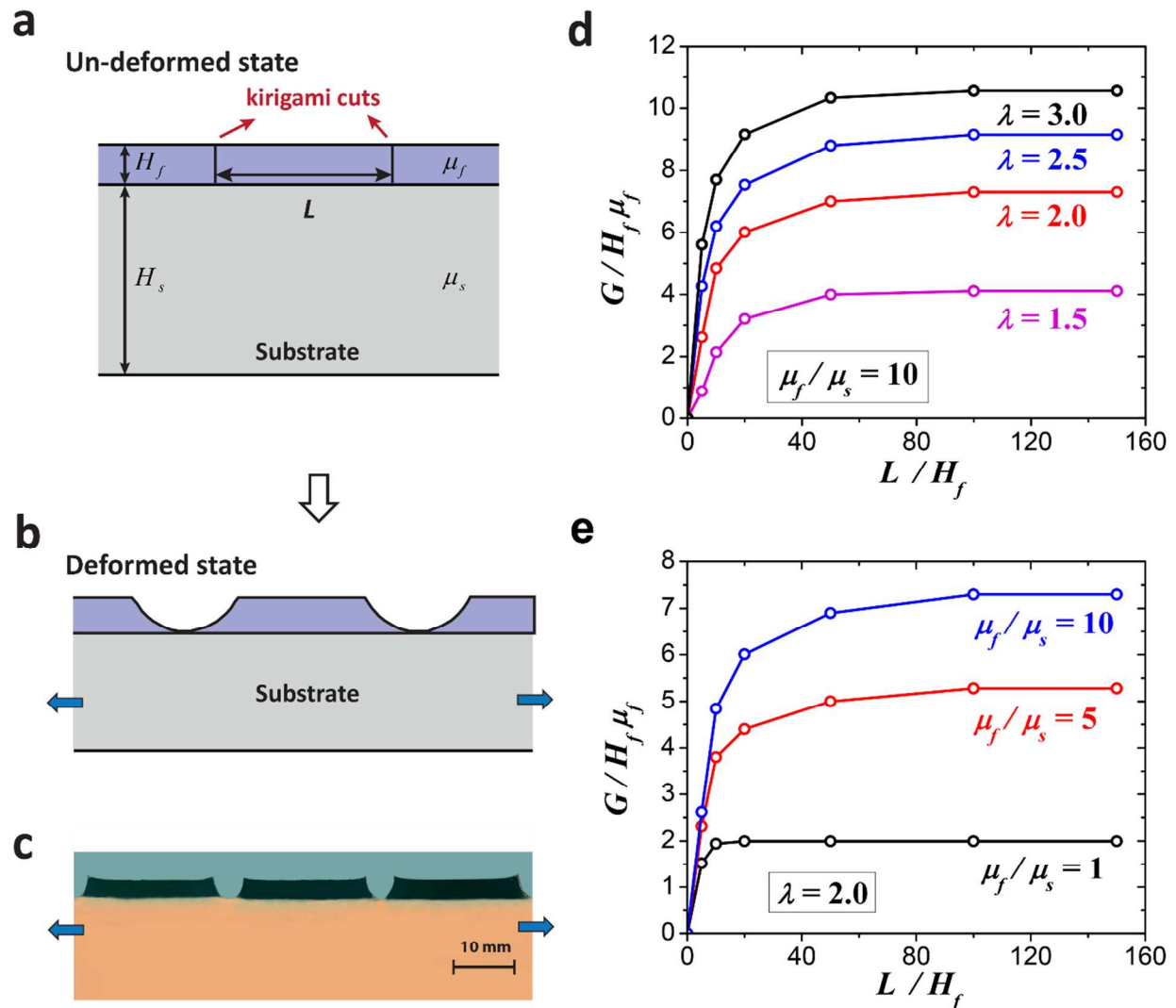
Fig. 2. Shear-lag effect of the film segments in a kirigami film. a) Schematic of the cross section of a film segment at the undeformed state. b) Deformation of film segments on a substrate under uniaxial stretch. The shear deformation around the edges of film segments gives the shear-lag effect, which reduces energy release rate compared with continuous film. c) Photo of deformed film segments on a substrate under uniaxial stretch. d) The normalized energy release rate G/H_f \mu_f for debonding initiation as a function of film segment size L/H_f and applied
