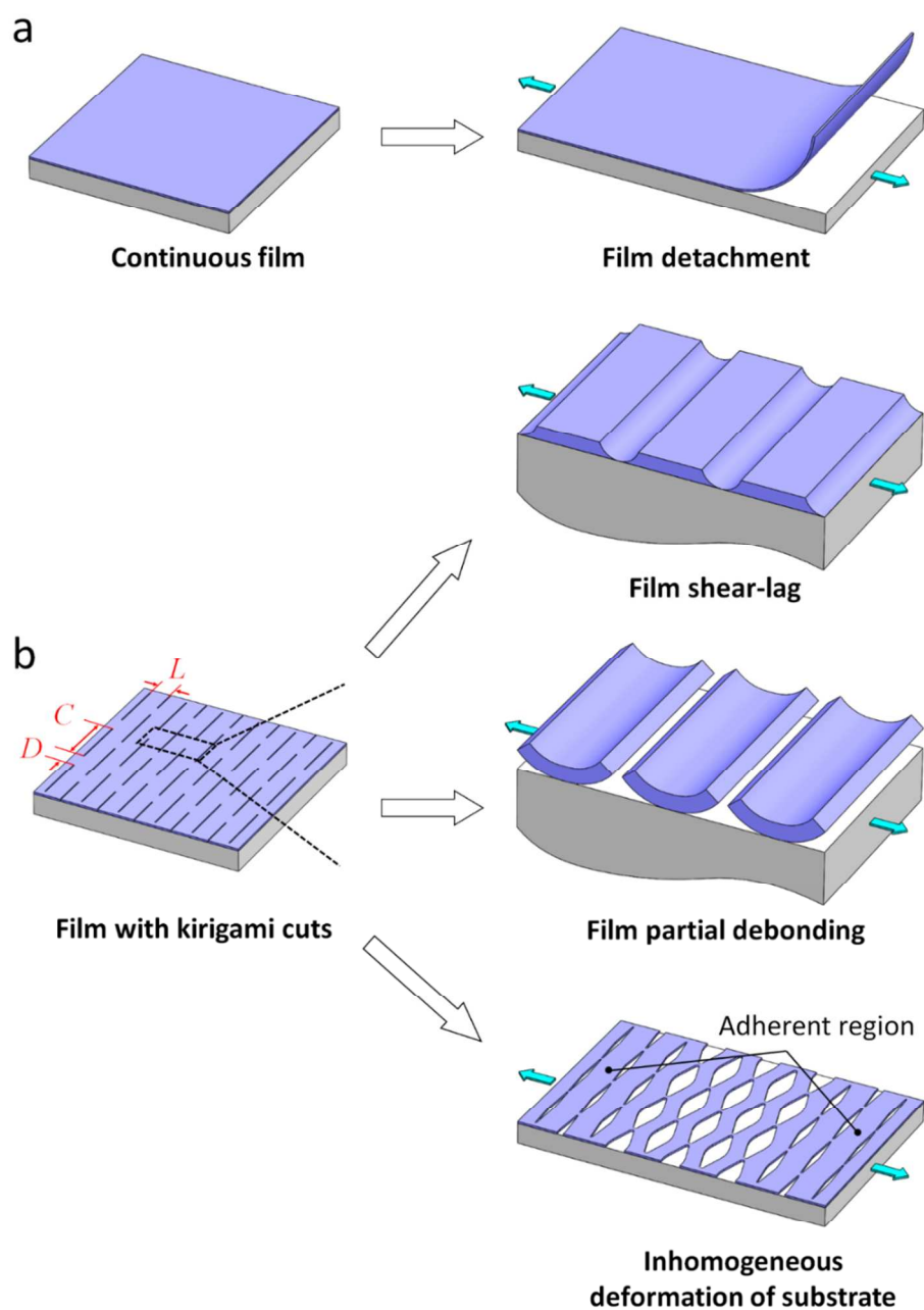
Fig. 1. Schematic illustration of mechanisms for kirigami enhancing film adhesion a) The continuous film delaminates from a substrate under critical strain. b) The film with designed kirigami cuts can significantly enhance the critical strain for delamination owing to shear-lag
