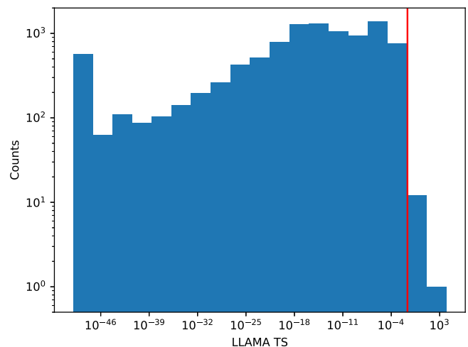
Figure A3. Background TS distribution of the LLAMA search for BBH mergers detected with the two aLIGO and the AdVirgo detectors at O2 sensitivity. Here TSs < 10^{-50} are collected in the 10^{-50} bin. The red line shows the one-sided 3\sigma threshold.
