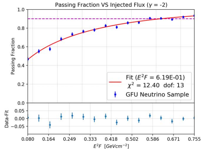
Figure A2. The 90% sensitivity flux for GW170729, computed by injecting an increasing neutrino flux according to an E^{-2} power-law spectrum and calculating the fraction of trials that return an observed \Lambda greater than the median of the background distribution shown in Figure A1. We use a \chi^2 CDF to fit the data and compute the time-integrated flux, which gives a 90% passing fraction. This is defined as the sensitivity for the particular GW event.
