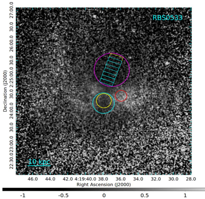
Figure 6. Model-subtracted relative residual image of RBS 0533 (same as in Figure 2) given by (N_I - N_M)/N_M . Overlaid are circular regions used in significance testing (see Table 3), where the magenta circle is the approximate location and size of an X-ray bubble. Since the bubble has no clear rims, rectangular regions are used to find the approximate edge of a bubble where its structure is barely detected ( S/N < 5 ), which corresponds to the yellow rectangle; see text for more details. Color regions to the south of the magenta circle may also be a cavity, although the S/N within these regions is low. This image is Gaussian smoothed with a 3'' kernel radius.
