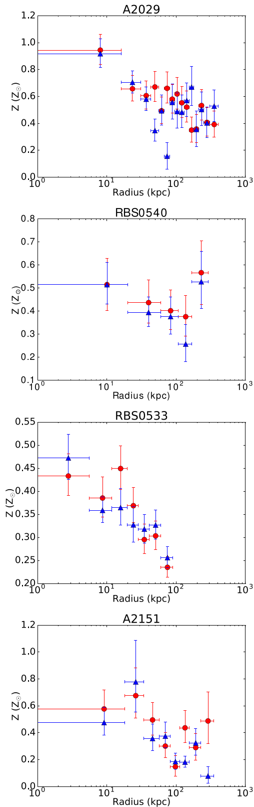
Figure 8. Metallicity profiles for the spoiler clusters, from top to bottom: A2029, RBS 0540, RBS 0533, A2151. Abundances along the jet axis are represented by red circles, while those for spectra in orthogonal directions or other off-jet locations are denoted by blue triangles. A2029’s along-jet profile shown here is of its northwest jet. These profiles show no evidence that metal-enriched gas preferentially lies along the jet axis, which is consistent with Figure 7. All errors here are reported at the 2\sigma level.
