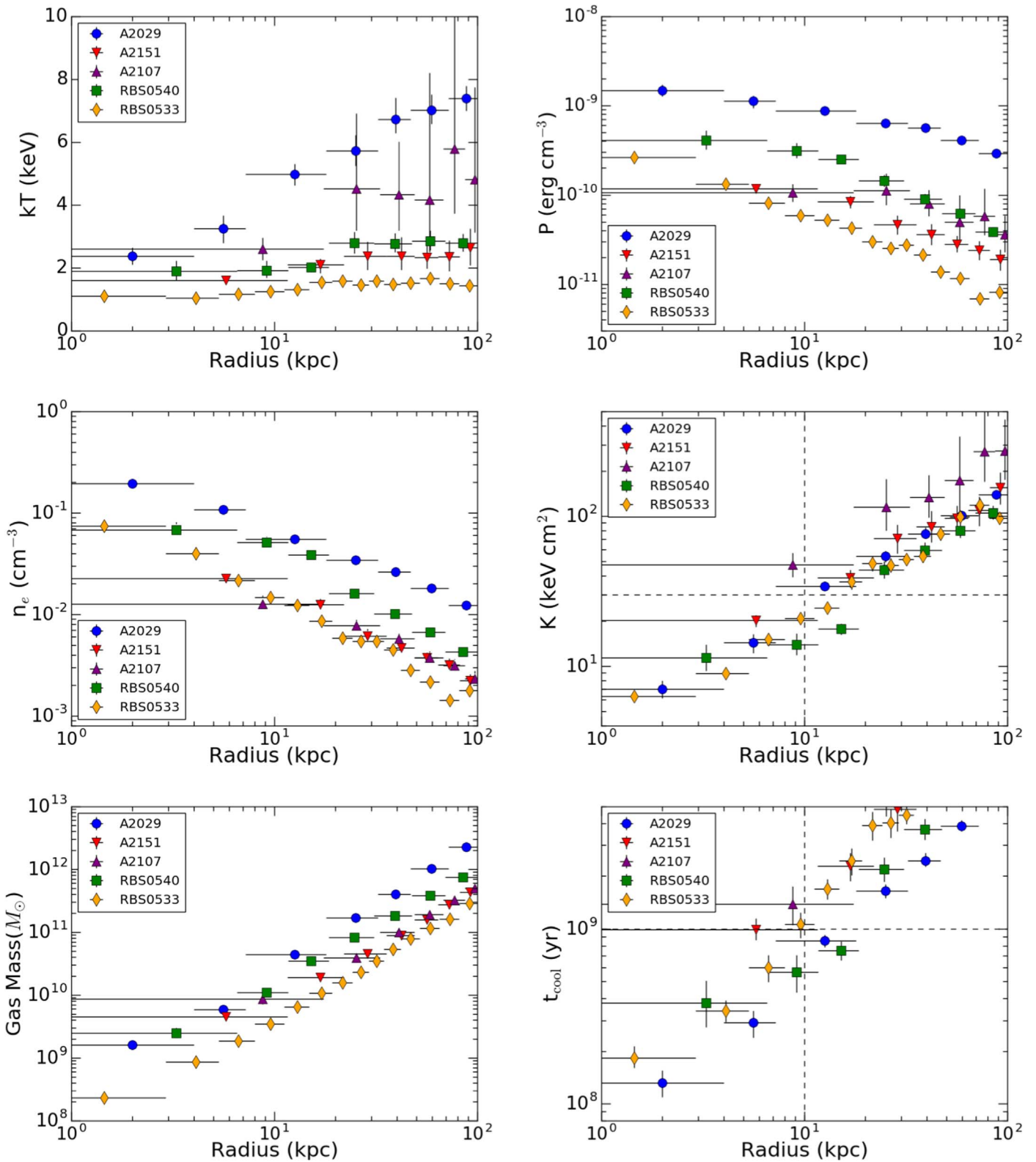
Figure 4. Deprojected temperature, pressure, density, entropy, gas mass, and cooling time profiles. The dashed horizontal lines represent the thresholds for the cooling time ( t_{\text{cool}} = 1.0 \times 10^9 yr) and entropy ( K = 30 keV cm 2 ). All errors here are reported at the 2\sigma level.
