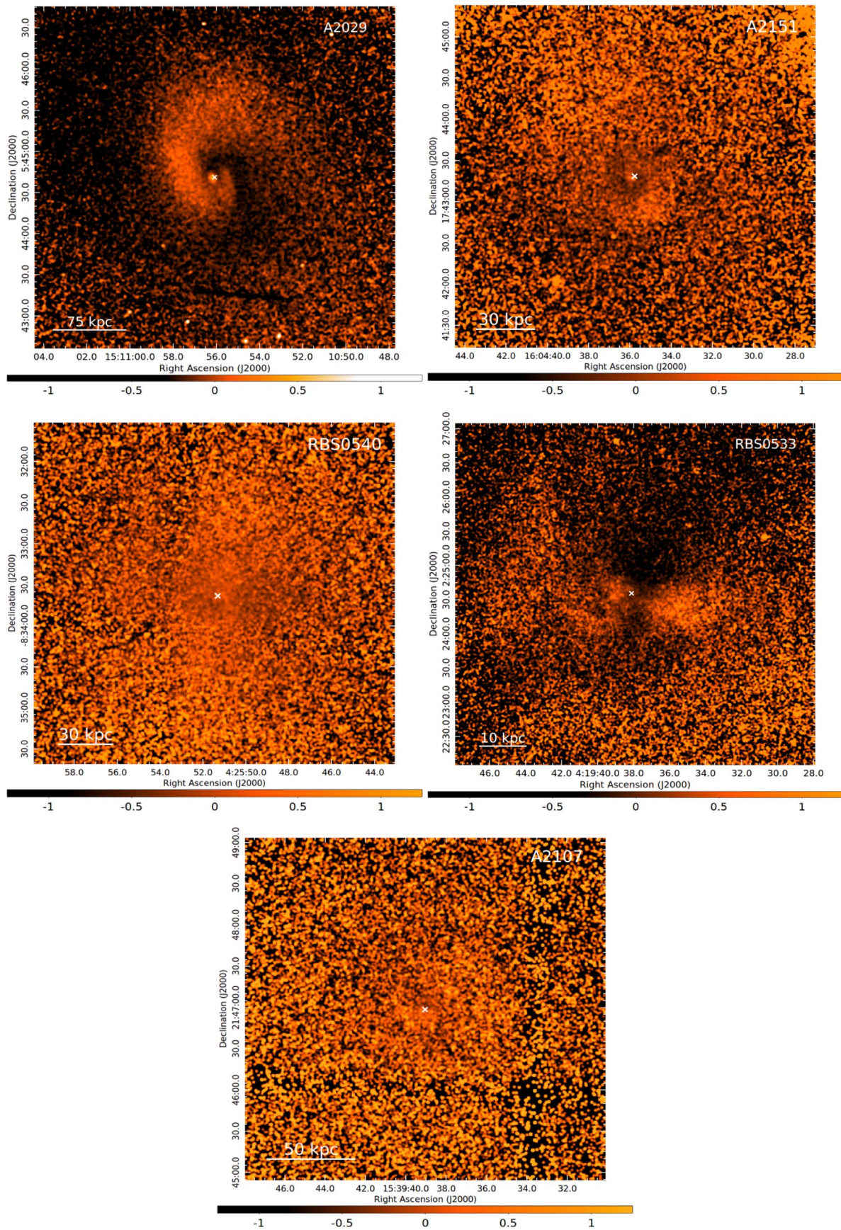
Figure 2. Model-subtracted relative residual images of each cluster. Images were obtained by fitting a double \beta -model to the cluster's surface brightness profile of the form in Equation (1) and then taking the relative difference between the images in Figure 1 and that of the model. The white cross represents the location of the brightest pixel and is the center used in \beta -model fitting. These images are Gaussian smoothed with a 3'' kernel radius.
