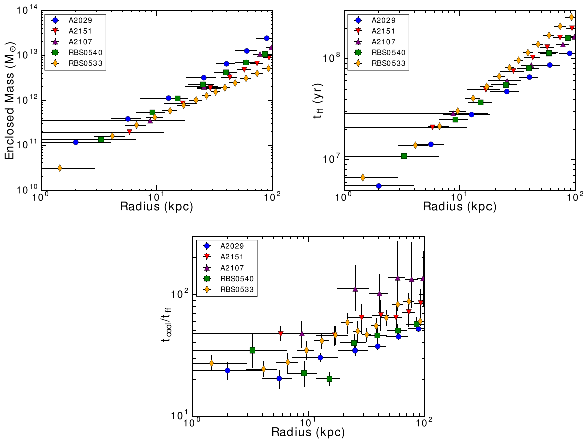
Figure 5. Top left: enclosed mass found from mass fitting; see Table 2. Top right: freefall profiles calculated using Equation (7). Bottom: deprojected t_{\text{cool}}/t_{\text{ff}} profiles.
