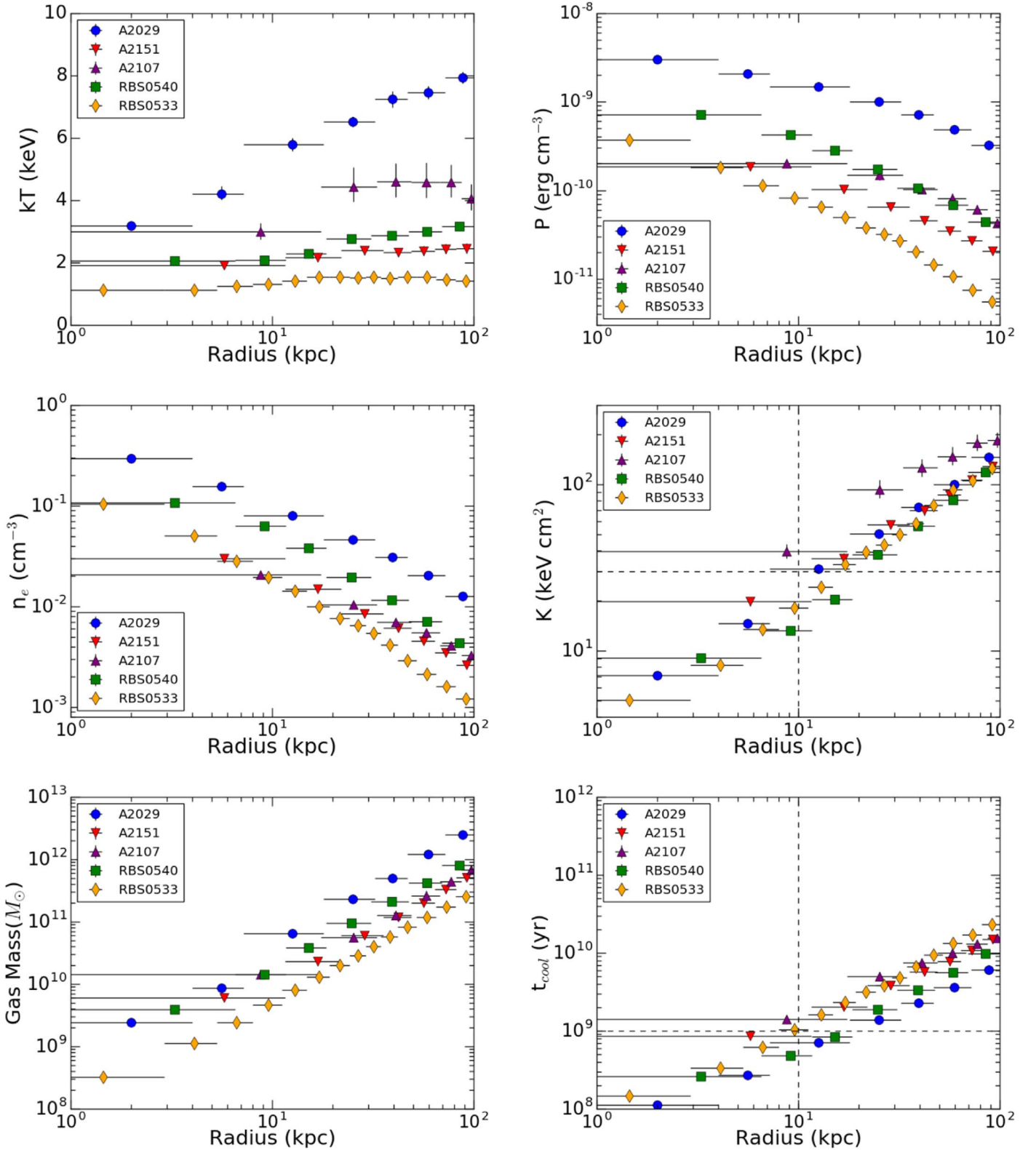
Figure 3. Projected temperature, pressure, density, entropy, gas mass, and cooling time profiles. The dashed horizontal lines represent the thresholds for the cooling time ( t_{cool} = 1.0 \times 10^9 yr) and entropy ( K = 30 keV cm 2 ). All errors here are reported at the 2\sigma level.
