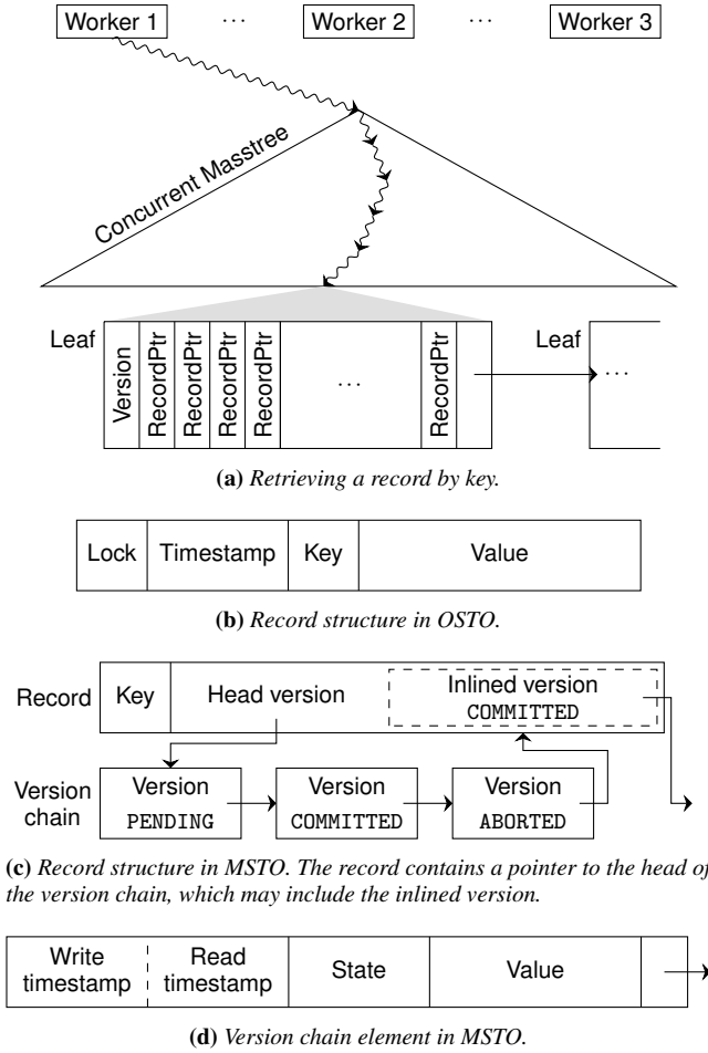
Figure 1: STOV2 overview.
