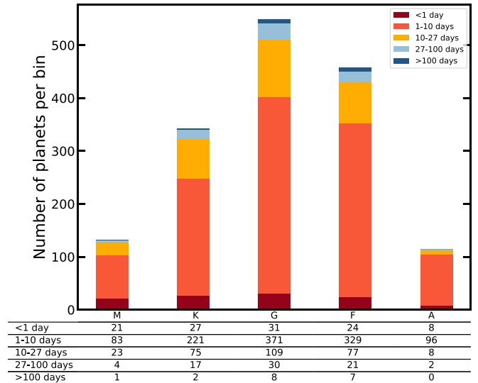
Figure 8. Period distribution for TOIs, subdivided by host star spectral type (M, K, G, F, and A). False-positive TOIs and TOIs with P = 0 are not included. For each spectral type, TESS has detected many TOIs in the 1–10 day period regime. These data are not corrected for completeness.
