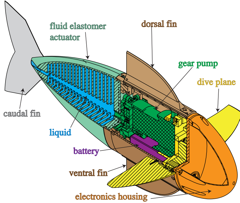
Fig. 1: Isometric cut of fish assembly
