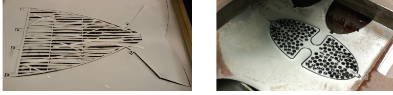
Fig. 6: Laser cut center constraint layer and water jet head constraint
