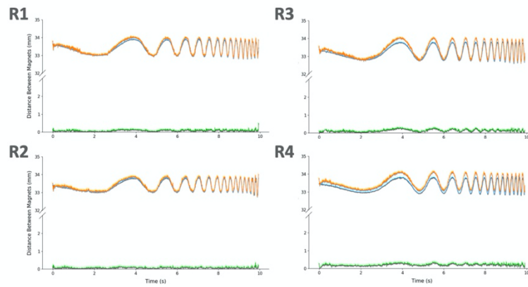
Supplementary Figure 2: Magnetomicrometry (Blue) Against Fluoromicrometry (Orange), with Absolute Difference (Green), for Mechanical Frequency Sweep on Turkey A Gastrocnemius. All plots correspond to trials from the same leg (right side). Plots R1, R2, R3 and R4 correspond to the first, second, third, and fourth trials.
