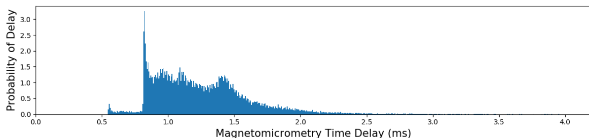
Supplementary Figure 1: Time Delay in Tracking Two Magnets with Disturbance Compensation for Magnetomicrometry. The time delay was measured as the time between receipt of the raw data by the computer and completion of the multi-magnet tracking algorithm with magnetic disturbance compensation. This histogram shows the distribution of time delays across all 22 mechanical frequency sweep magnetomicrometry trials. The 99 th -percentile time delay was 2.52 ms.
