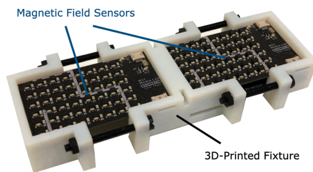
Figure 6: Magnetic Field Sensing Array. Two 6x8 magnetic field sensor grids were custom designed and held together using a 3d-printed fixture and nylon nuts and bolts.
