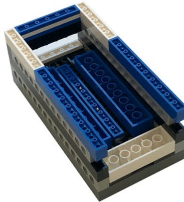
Supplementary Figure 9: LEGO Assembly Used in Static Magnetomicrometry Versus Fluoromicrometry. A LEGO assembly was constructed to hold the sensor array fixture of Figure 6 sensor-side down and position the magnetic beads apart from one another at 16-mm separation distance intervals. Magnetic beads are shown positioned in a 1x10 LEGO plate at the base of the assembly. Sensor proximity was modified by the attachment of 2x12 plates along the sides of the assembly.
