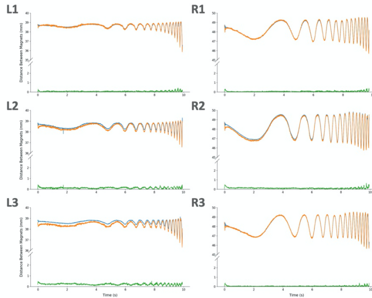
Supplementary Figure 3: Magnetomicrometry (Blue) Against Fluoromicrometry (Orange), with Absolute Difference (Green), for Mechanical Frequency Sweep on Turkey B Gastrocnemius. Plots L1, L2, and L3 correspond to the first, second, and third trials on the left leg, and plots R1, R2, and R3 correspond to the first, second, and third trials on the right leg.
