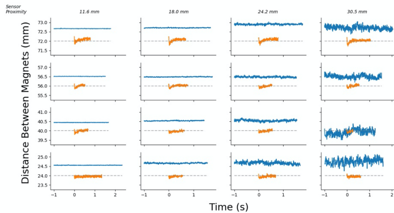
Supplementary Figure 10: Static Magnetomicrometry Versus Fluoromicrometry (Time-Series). Magnetomicrometry (blue) and fluoromicrometry (orange) measurements were taken while magnets were placed at separation distances of approximately 24, 40, 56, and 72 mm in a LEGO block (horizontal dashed gray lines in each row), with the sensing array at various heights above the magnets. In contrast with Supplementary Figure 6, the vertical axis shows the separation distances, and the different columns correspond to the different sensor proximities (annotated above plots). Magnetomicrometry data is plotted for one second before and one second after the start and end of the fluoromicrometry measurements, respectively. It can be observed from these plots that some of the fluoromicrometry measurements exhibit a warm-up time lasting a small fraction of a second.
