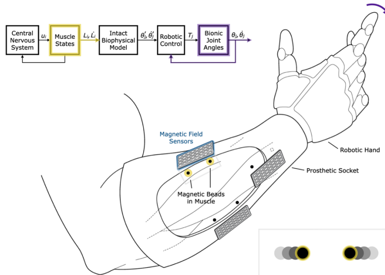
Figure 1: Free-Space Control of a Robotic Prosthesis via Muscle Magnetomicrometry. Passive magnetic beads (highlighted here in yellow) implanted in muscle can be used to wirelessly track muscle length via an array of magnetic field sensors (blue) mounted to the outside of the body. The pair of magnetic beads highlighted here is placed in a single muscle, in line with the muscle fiber orientation. Muscle length data can be streamed to a control unit, which can in turn be used to stream commands to neuroprosthetic devices such as exoskeletons, muscle stimulators, or the robotic hand shown here. In a free-space control methodology, agonist and antagonist muscle states (box indicated in yellow) voluntarily commanded by the user are mapped through a model of an intact biological limb to control joint angles (indicated here in purple) by modulating motor torque. This control strategy can be extended beyond free-space control by incorporating muscle activation or direct force measurement.
