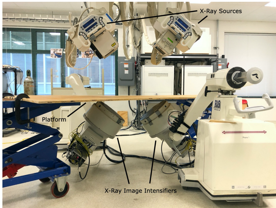
Supplementary Figure 8: XROMM Setup. Two X-ray sources above and two X-ray image intensifiers below were used to collect stereo X-ray video of the radio-opaque magnetic beads in the turkey leg. A platform was placed between the X-ray sources and image intensifiers for the turkey to rest on and on which to mount the motor and spring.
