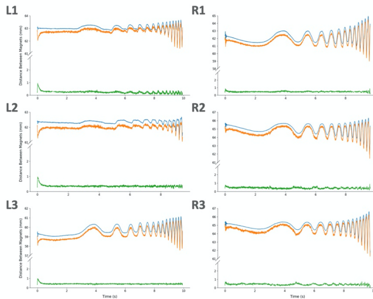
Supplementary Figure 4: Magnetomicrometry (Blue) Against Fluoromicrometry (Orange), with Absolute Difference (Green), for Mechanical Frequency Sweep on Turkey C Gastrocnemius. Plots L1, L2, and L3 correspond to the first, second, and third trials on the left leg, and plots R1, R2, and R3 correspond to the first, second, and third trials on the right leg.
