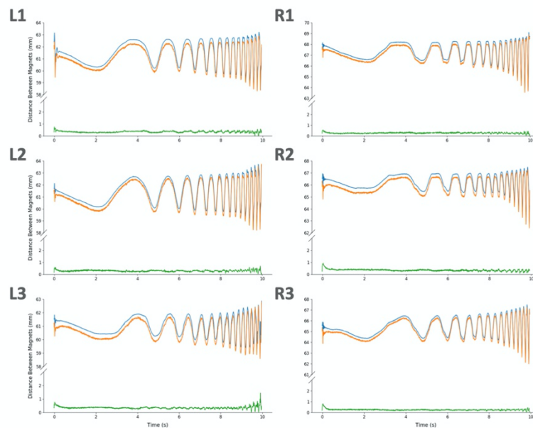
Supplementary Figure 5: Magnetomicrometry (Blue) Against Fluoromicrometry (Orange), with Absolute Difference (Green), for Mechanical Frequency Sweep on Turkey D Gastrocnemius. Plots L1, L2, and L3 correspond to the first, second, and third trials on the left leg, and plots R1, R2, and R3 correspond to the first, second, and third trials on the right leg.
