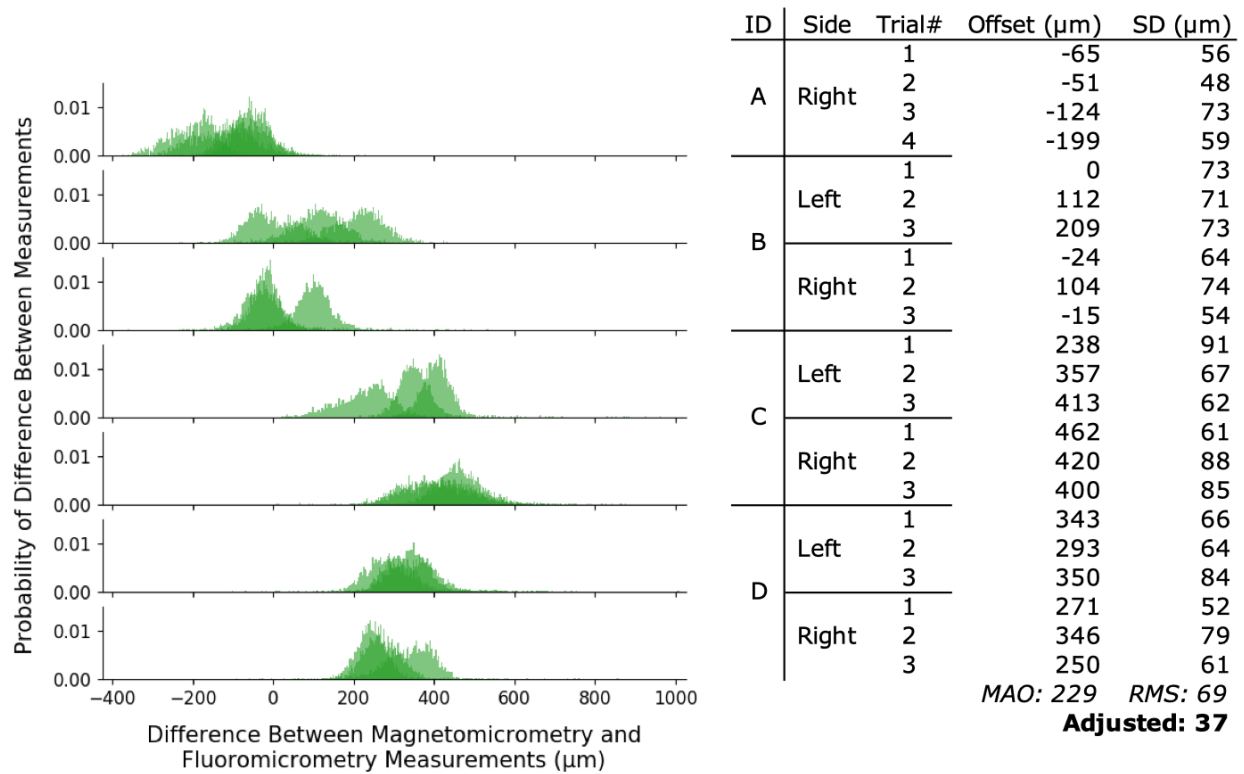
Figure 3: Difference Between Magnetomicrometry and Fluoromicrometry Gastrocnemius Frequency Sweep Measurements, in Micrometers. Histograms show the probability distribution of the difference between magnetomicrometry and fluoromicrometry for each of the four turkeys (turkeys A through D, show from top to bottom alternating between left and right legs), for all trials with each leg. The table shows the offset and standard deviation (SD) for each of the trials, giving a representation of the accuracy and intra-trial precision. Across all trials, the mean absolute offset (MAO) was 229 \mu\text{m} , and the measured precision was 69 \mu\text{m} , root-mean-square (RMS), with an adjusted RMS precision of 37 \mu\text{m} (accounting for the noise from fluoromicrometry). Note that the left gastrocnemius of turkey A was omitted from these trials, as discussed in the results of the migration study.
