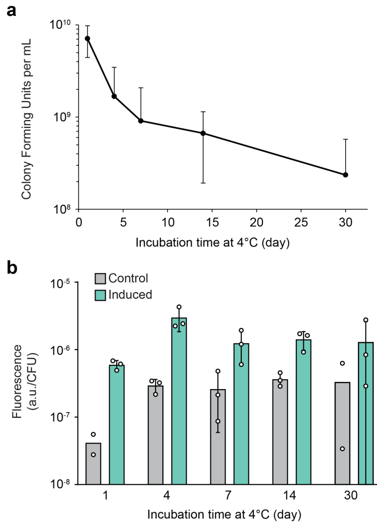
Supplementary Fig. 13 | Cell survival and inducibility after storage at low temperature. (a) CFU counts for cells retrieved from hydrogel beads after storage in a refrigerator (4°C) across 30 days (b) Comparison of aTc-induced fluorescence profiles of retrieved cells after storage at 4°C for various time periods. Samples prepared in triplicate (duplicate for the control group on day 1 and 30), data represent the mean \pm 1 SD.
