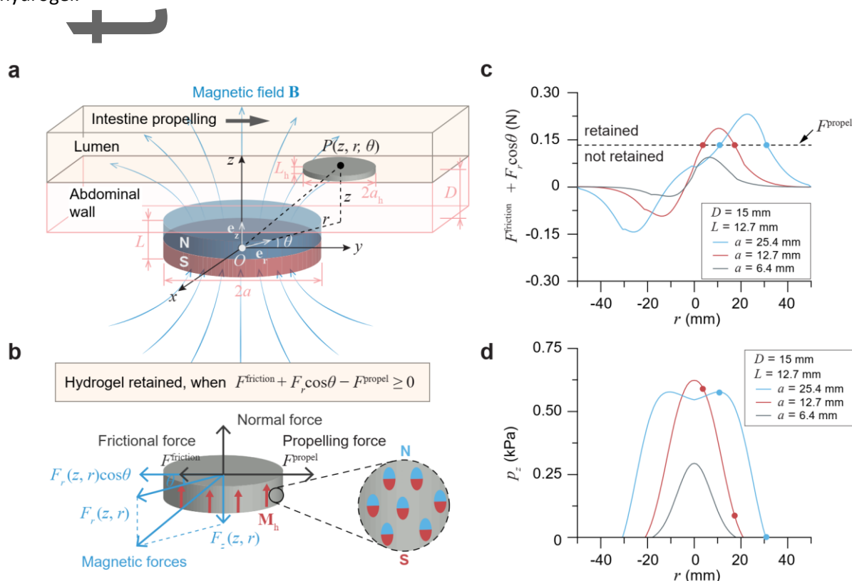
Figure 2. Model for intestinal retention and localization of the magnetic living hydrogel. a) Schematic illustration of a disc-shaped magnetic hydrogel (radius a_h and thickness L_h ) residing in a lumen under a magnetic field \mathbf{B} generated by a disc-shaped magnet (radius a and thickness L ). The vertical distance between the lumen and the magnet is D . b) Free body diagram of the magnetic hydrogel in the intestinal lumen, when it is moving along the intestinal propelling direction. The magnetization of the hydrogel \mathbf{M}_h is uniform and along the axial direction of the hydrogel disc. c) Net retarding force ( F^{\text{friction}} + F_r \cos \theta ) of a magnetic hydrogel (radius a_h 10 mm, thickness L_h 1 mm) at a vertical distance of 15 mm away from a magnet (radius a 6.4, 12.7, or 25.4 mm, thickness L 12.7 mm). The
