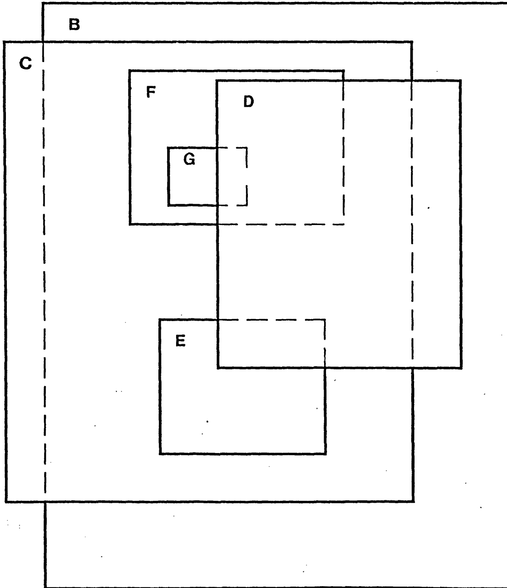
Figure 3 - Overlapping Windows
