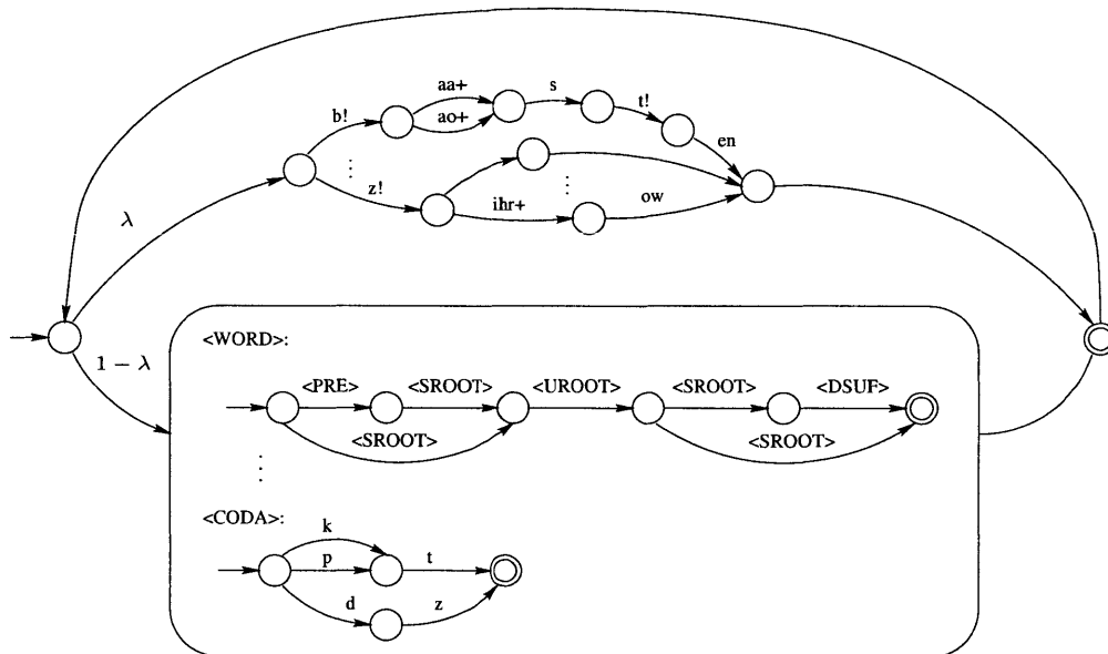
Figure 3-5: The FST topology for the hierarchical and phoneme network hybrid model. Similar to the phoneme filler model, there are two branches in the FST network. The phoneme network branch is used for modeling in-vocabulary words. The hierarchical RTN branch is used for modeling previously unseen words.
