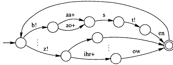
Figure 3-2: FST topology for the phoneme network model. Each path represents a legitimate phoneme sequence from words in the vocabulary.
