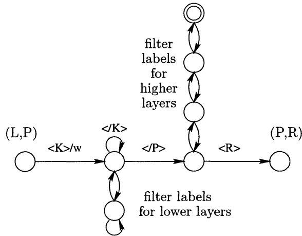
Figure 3-8: The state diagram in an intermediate layer probability FST. It shows the transitions from a state (L,P) to state (P,R) , where P , L , and R are the current parent, its left sibling and its right sibling in the parse tree, respectively. “ w ” is the probability \text{Prob}(P \mid L, K) , where K is the first child of P .
