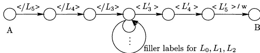
Figure 3-9: The state diagram in a phone advancement probability FST. It shows the transition from the left column A ( [L_0, L_1, L_2, L_3, L_4, L_5] ) to the right column B ( [L_0, L_1, L_2, L_3', L_4', L_5'] ). L_0 is the top layer category. “w” is the probability of the right phone ( L_5' ) given the left column.
