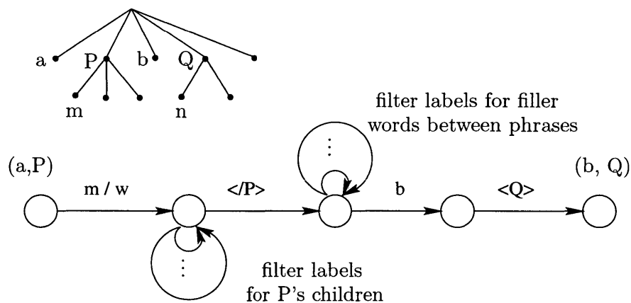
Figure 5-3: The context state transition diagram in the phrase-level context-dependent rule-start probability FST. It shows the transitions from a state (a,P) to state (b,Q) , where P , a , Q , and b are the current parent, the current parent’s left sibling, the next parent, and the next parent’s left sibling in the shallow parse tree, respectively. “ w ” is the context-dependent rule-start probability \text{Prob}(m \mid a, P) normalized by the generic rule-start probability \text{Prob}(m \mid \#, P) , where “ m ” is the first child of P , and “ \# ” is the rule-start marker.
