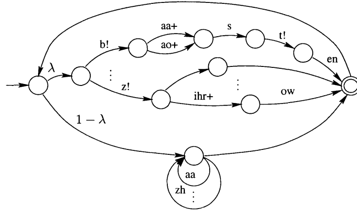
Figure 3-3: FST topology for the phoneme network model with fillers. The top branch is the same as the phoneme network model, and the bottom branch represents the phoneme fillers. \lambda and 1 - \lambda are the transition weights that control the penalty of entering each branch.
