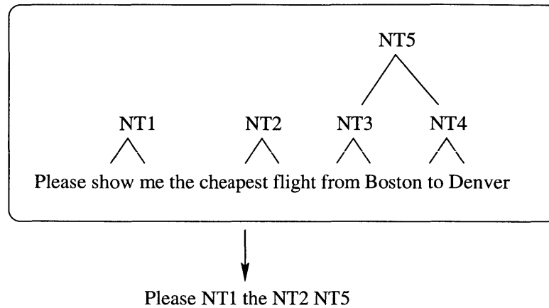
Figure 4-2: The phrase reduction from the original sentence to the reduced sentence. NT1 through NT5 are nonterminals in the phrase grammar.
