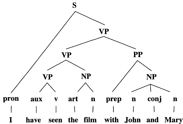
Figure 4-3: Sample parse tree of the sentence “I have seen the film with John and Mary”, according to a syntactic grammar. The bottom layer above the words contains the POS tags, such as pronoun (pron), auxiliary (aux), verb (v), article (art), and preposition (prep). The parse nodes above the bottom layer are the nonterminals defined in the syntactic grammar, such as noun phrase (NP), verb phrase (VP), and sentence (S).
