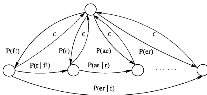
Figure 3-4: FST topology for the phoneme bi-gram model. The states at the bottom are context states, which are used to remember the current left phoneme contexts. Bi-gram probabilities are encoded in weighted transitions from current context states to next context states shown at the bottom of the figure. \epsilon transitions are associated with the back-off weights, and the back-off uni-gram transitions are weighted from uni-gram probabilities.
