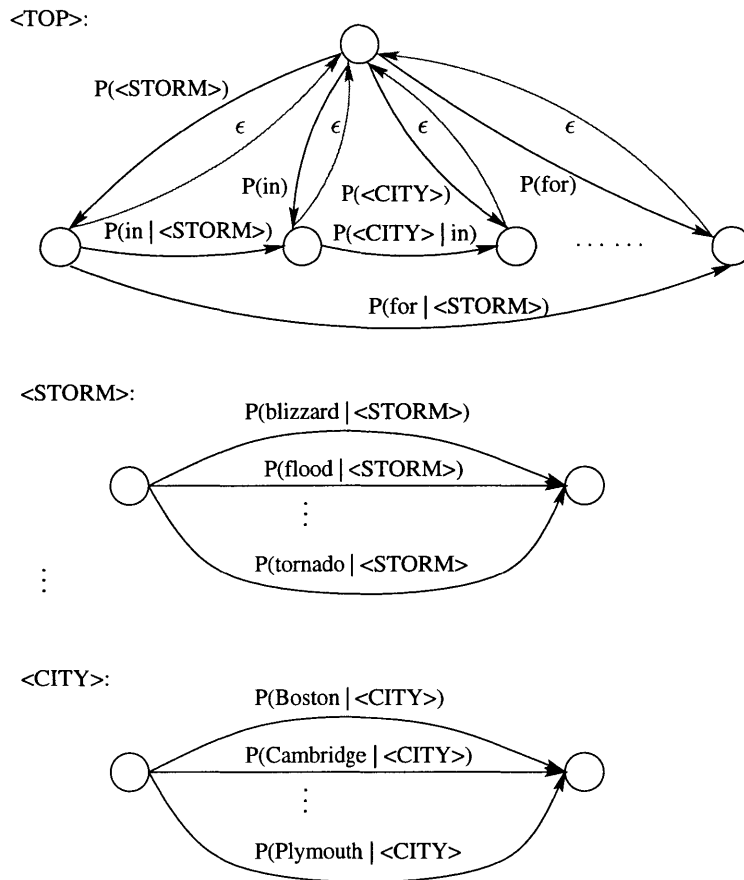
Figure 5-1: FST topology for a class bi-gram model. The top-level network has the same structure as a regular word bi-gram model, except that some transitions are labeled with classes. Other sub-networks represent the class expansions, and are weighted according to the probabilities of each word within the class.
