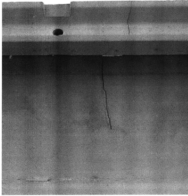
Figure 6-3: Cracking observed during casting, which runs from the deck to the neutral axis [9].
