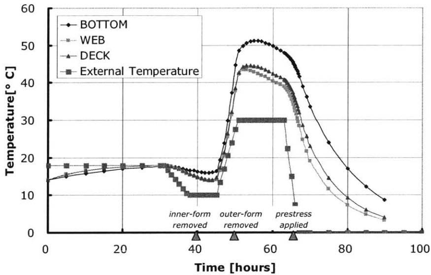
Figure 6-11: Temperature history from the simulation with E_a/R = 4,000 K .
