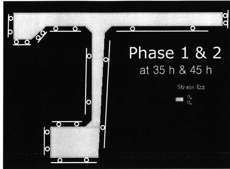
Figure 6-20: Distribution of the longitudinal plastic strain in the composite matrix ( \varepsilon_{M,zz}^p ) at both 35 and 45 hours after casting in Phase 1 and 2, respectively.
