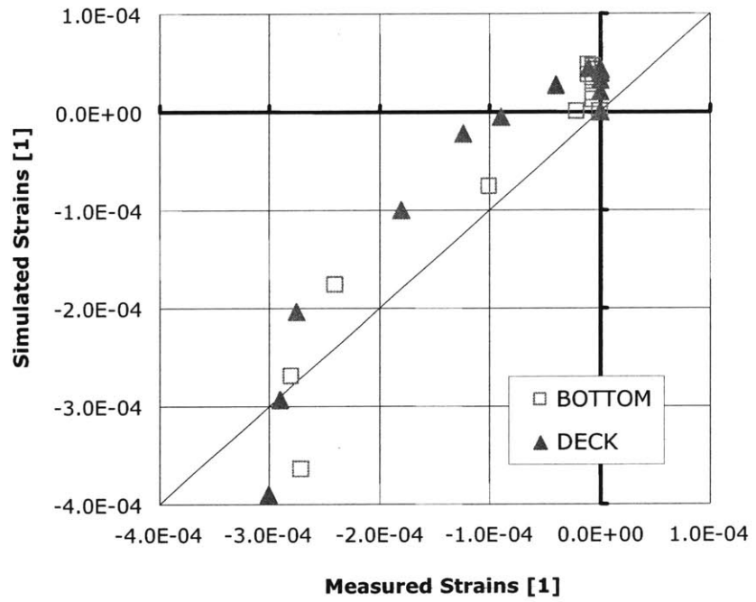
Figure 6-17: Measured strains compared with simulated strains.
