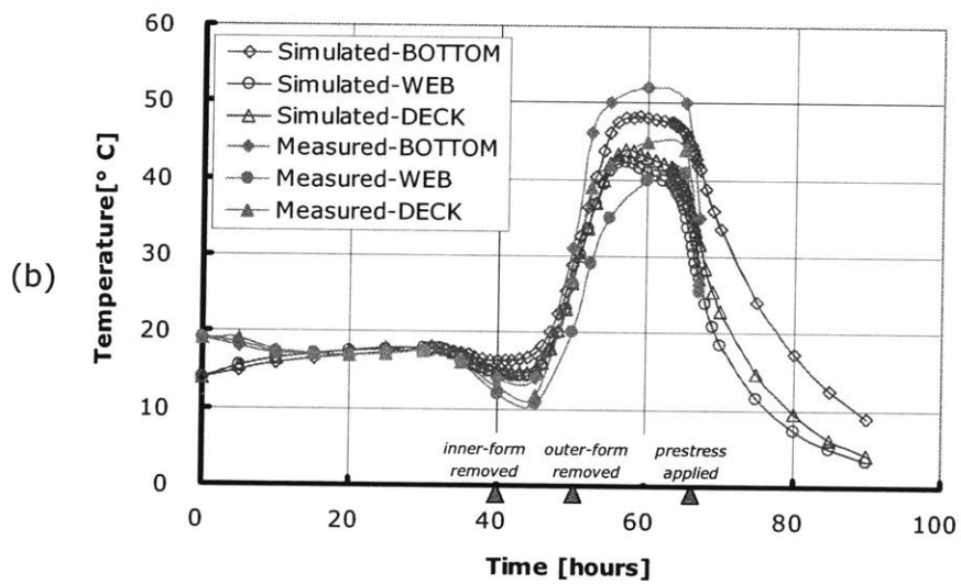
Figure 6-12: Comparison of on-site measured and simulated temperature histories: (a) E_a/R = 4,000 K , (b) E_a/R = 4,150 K .
