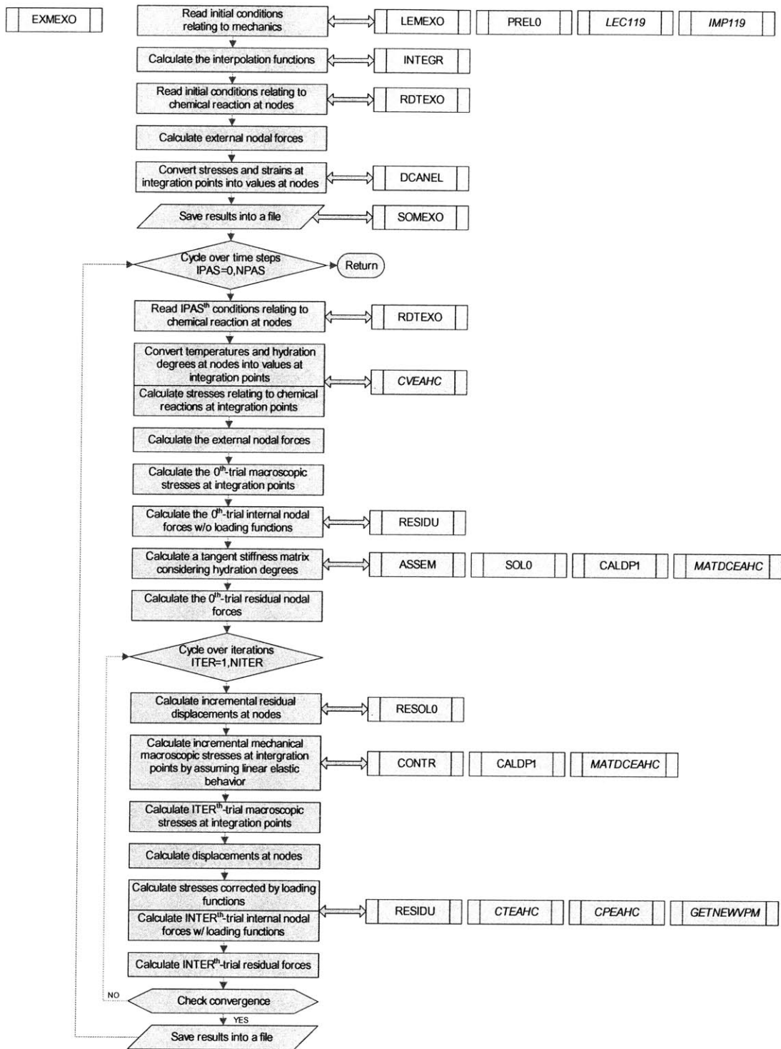
Figure 5-4: Flow chart of the subroutine EXMEXO and corresponding subroutines, where italic letters indicate newly developed subroutines for the EAHC module.
