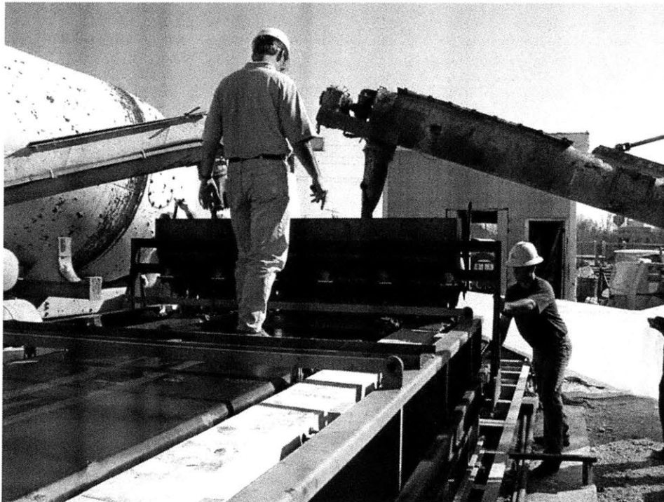
Figure 1-2: Construction of the Ductal TM bridge girders at Lexington, Kentucky [9].
