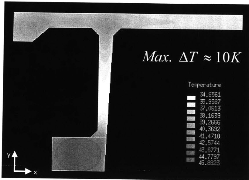
Figure 6-14: Temperature distribution at the moment of prestress application.
