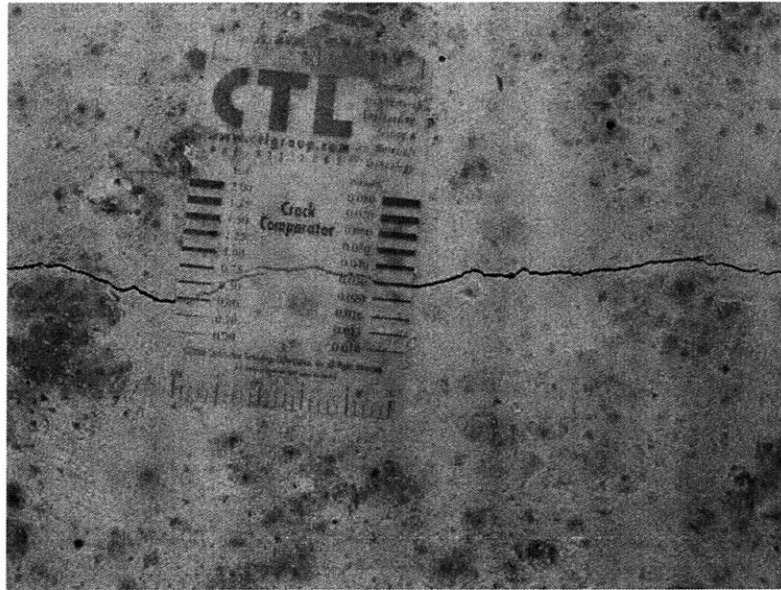
Figure 1-3: Early-age cracking observed during casting of on UHPC bridge girder [9].
