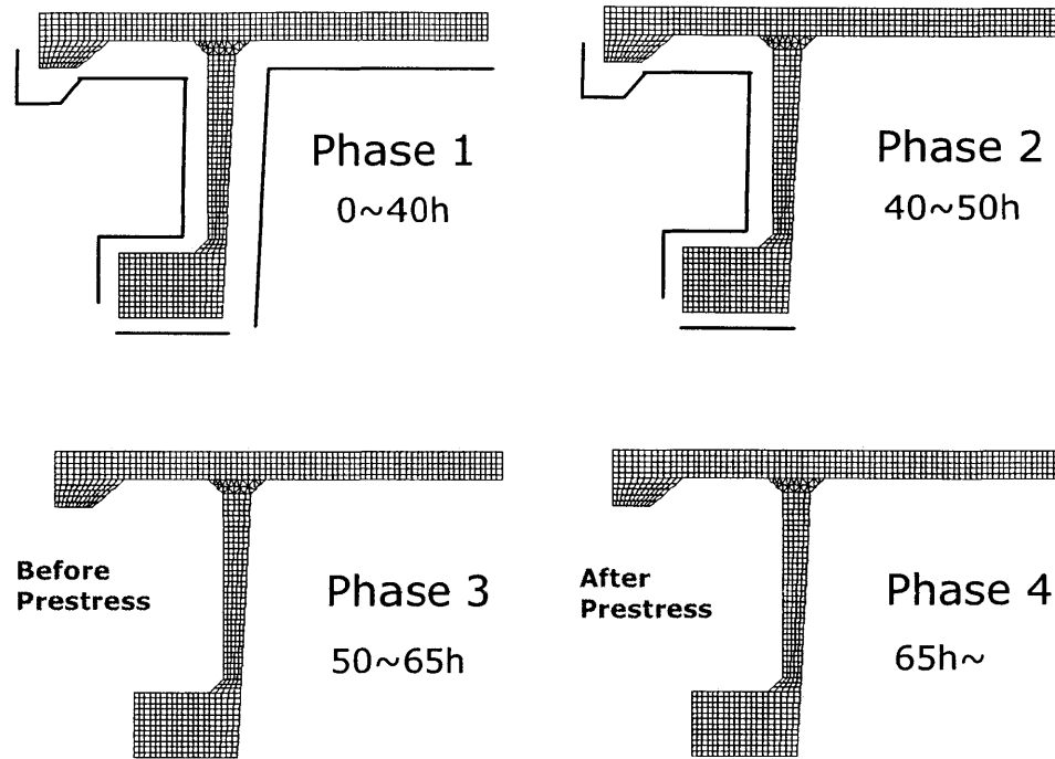
Figure 6-5: Progressive formwork removal inducing change in thermal boundary conditions.
