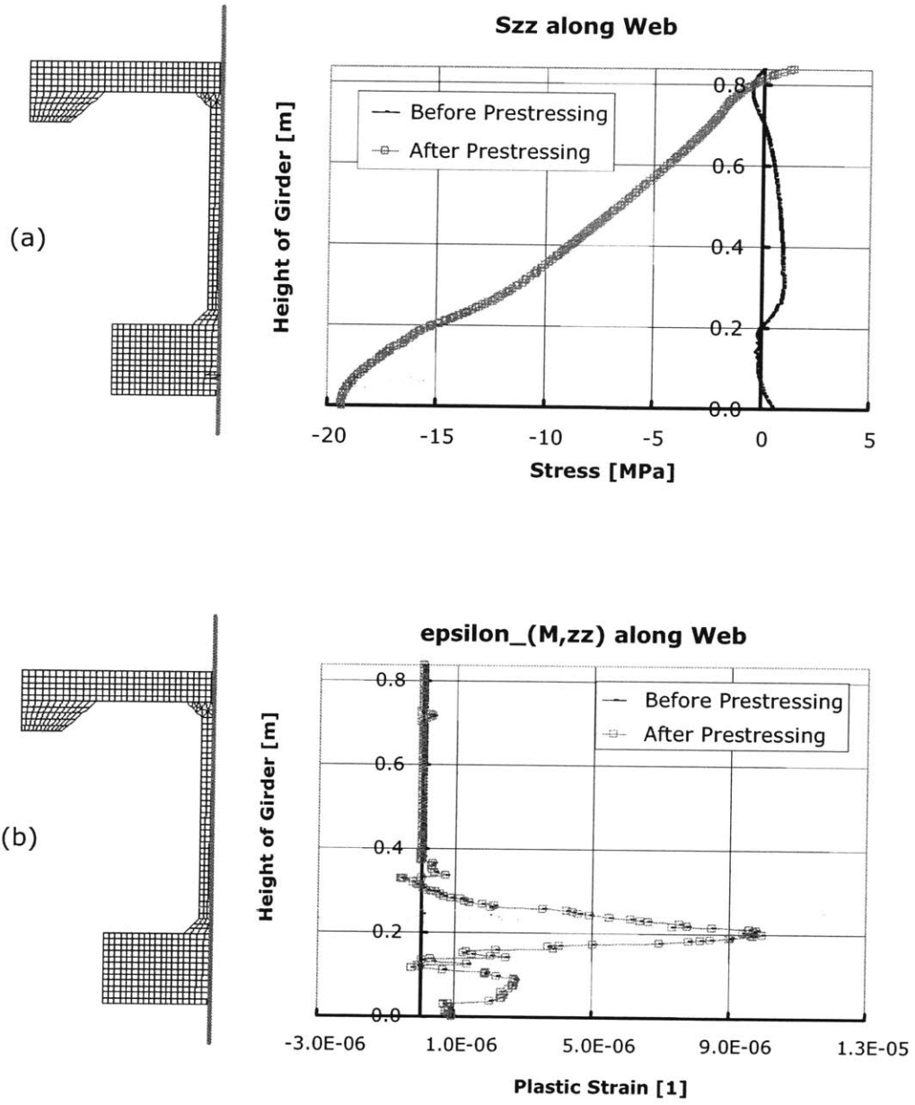
Figure 6-22: (a) Longitudinal macroscopic stress profile along the web, (b) Longitudinal plastic strain in the composite matrix along the web.
