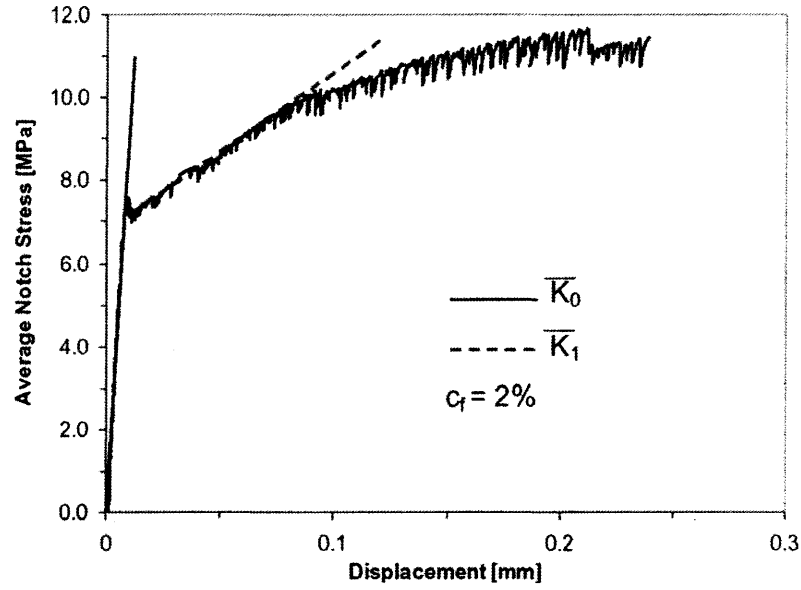
Figure 2-9: Average notch stress-displacement curve for Ductal TM -Steel Fiber [7].
