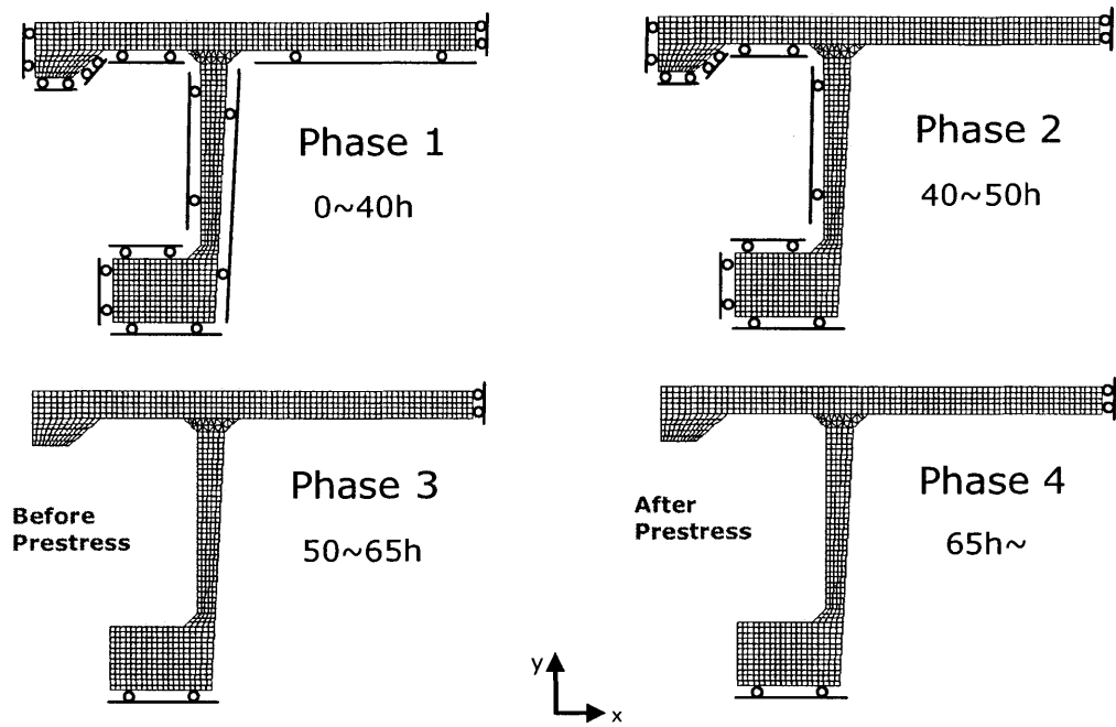
Figure 6-15: Progressive formwork removal inducing a change in displacement boundary conditions.
