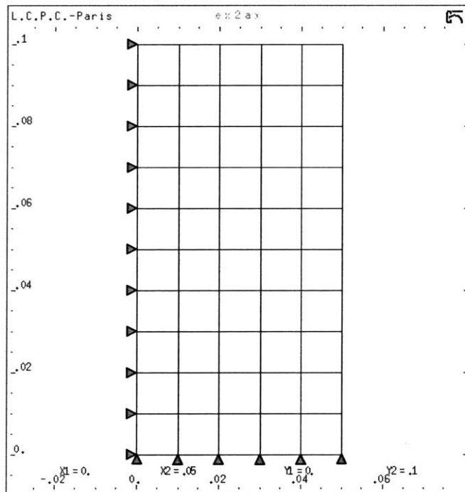
Figure 5-5: Mesh design and boundary conditions of the uniaxial tension test simulation using axisymmetric elements: (a) Single element, (b) Fifty elements.
