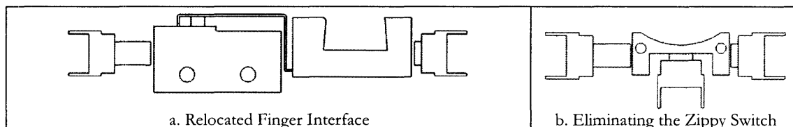
Figure 15: Alternative Key Designs
