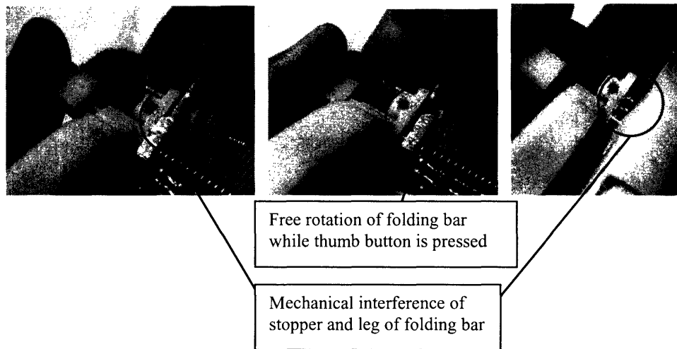
Figure 12: Locking Mechanism
