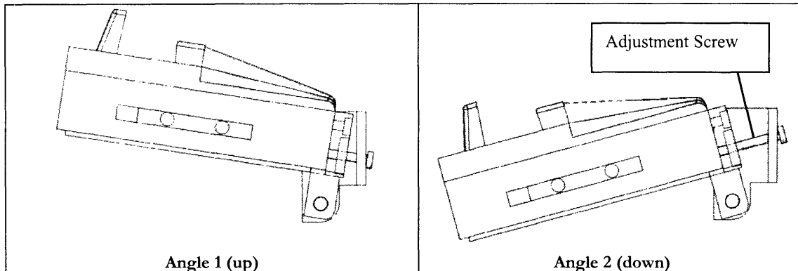
Figure 11: Angle Adjustment
