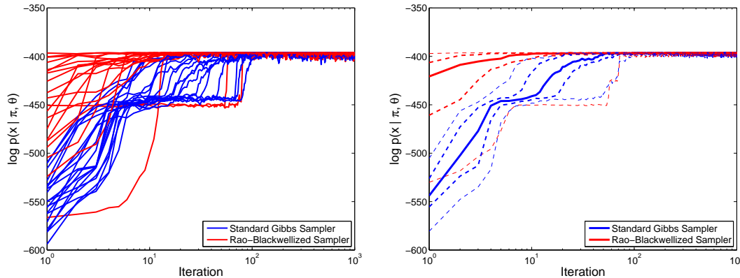
Figure 2.20. Comparison of standard (Alg. 2.1, dark blue) and Rao–Blackwellized (Alg. 2.2, light red) Gibbs samplers for a mixture of K = 4 two-dimensional Gaussians. We compare data log-likelihoods at each of 1000 iterations for the single N = 300 point dataset of Figs. 2.18 and 2.19. Left: Log-likelihood sequences for 20 different random initializations of each algorithm. Right: From 100 different random initializations, we show the median (solid), 0.25 and 0.75 quantiles (thick dashed), and 0.05 and 0.95 quantiles (thin dashed) of the resulting log-likelihood sequences. The Rao–Blackwellized sampler has superior typical performance, but occasionally remains trapped in local optima for many iterations.
