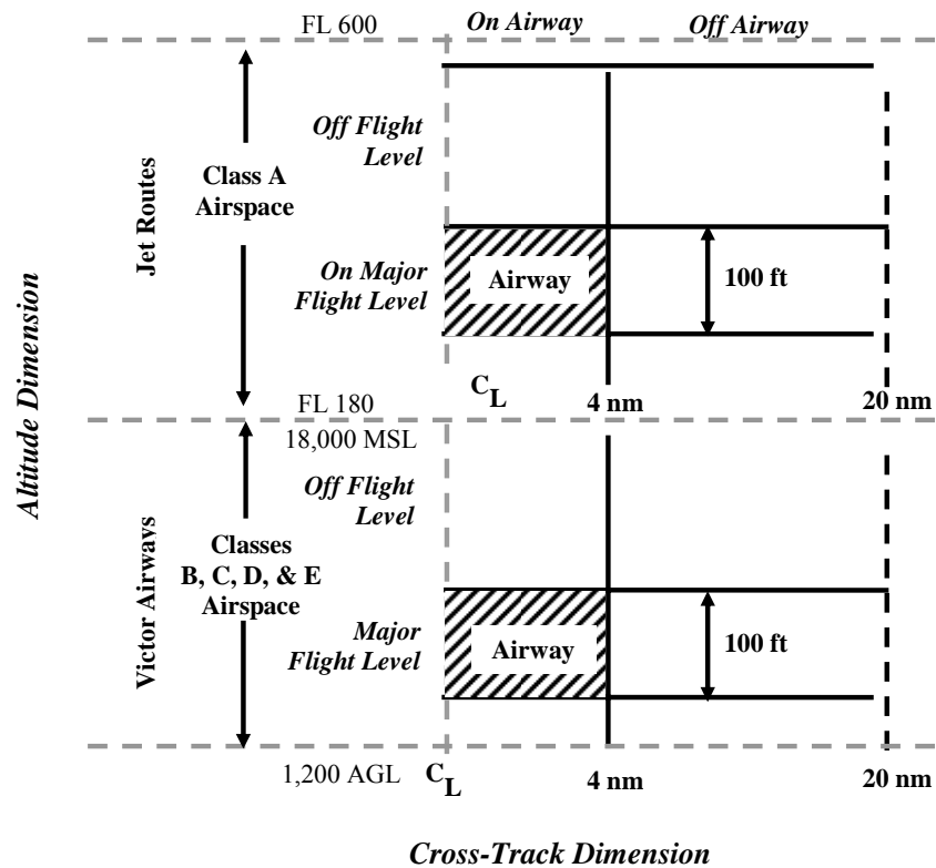
Figure 29: Conceptual Areas of Operation in the Vicinity of Airways
