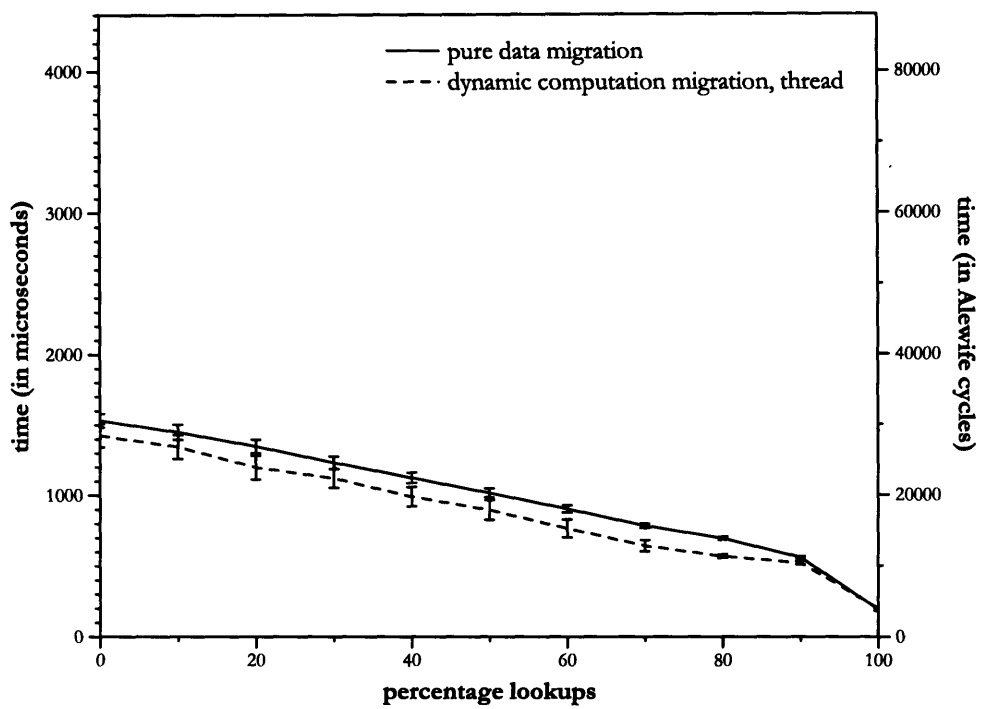
Figure 7-16. Cost per iteration of accessing a B-tree on Alewife using the REPEAT heuristic.
