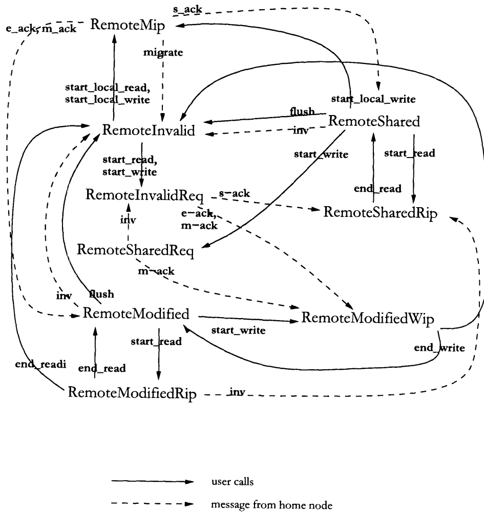
Figure A-3. Remote state diagram for MCRL
