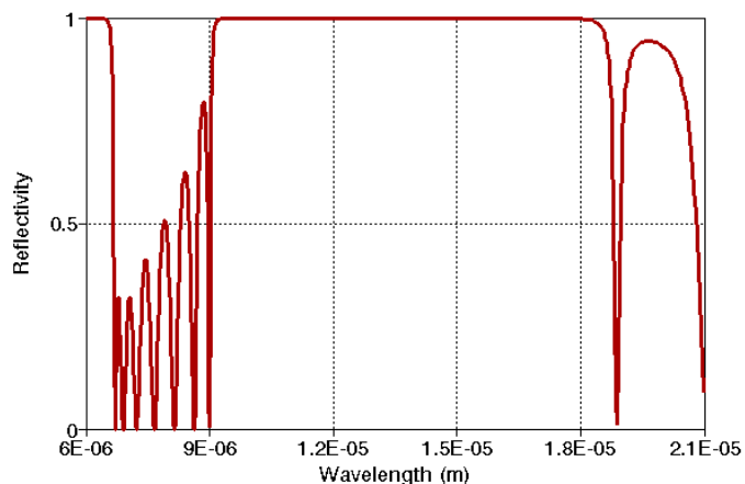
Figure 6 45° incidence. TE polarization.
