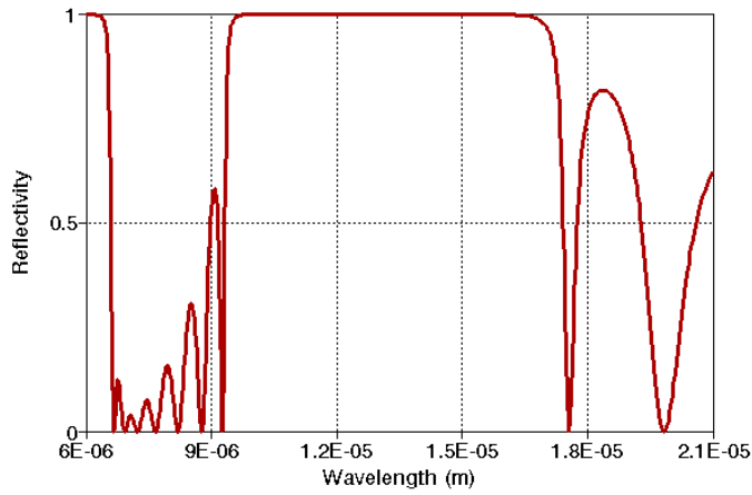
Figure 7 45° incidence. TM polarization.
