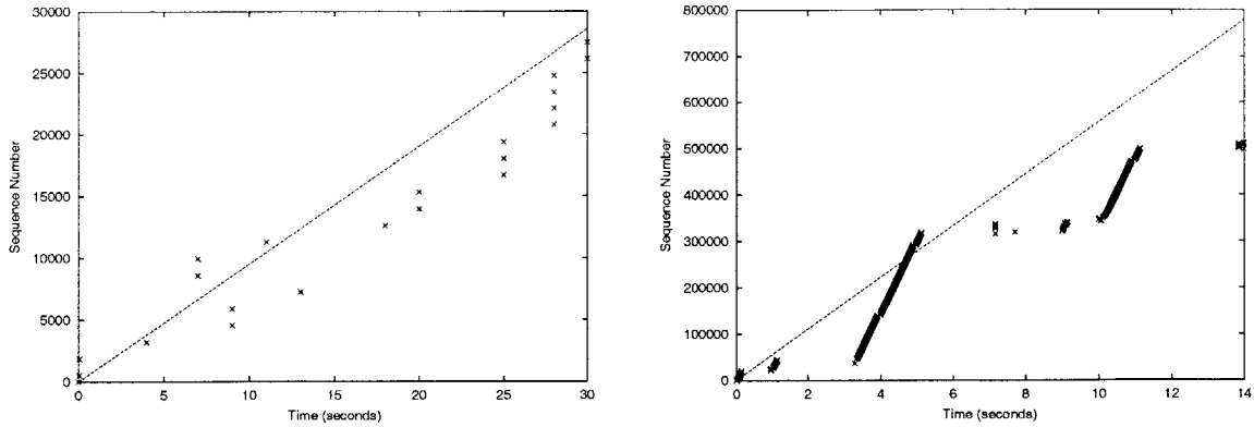
Figure 4-10: Left: a TCP trace between two Span non-coordinator nodes. Right: a TCP trace between two Span coordinators. In both figures the x-axis is the time that the packet was received, with t = 0 equal to the time the first byte was received. The y-axis is the sequence number of the last byte in the received packet. Each point on the graph represents the receipt of a 1024-byte packet. The dotted line shows the link bandwidth.
