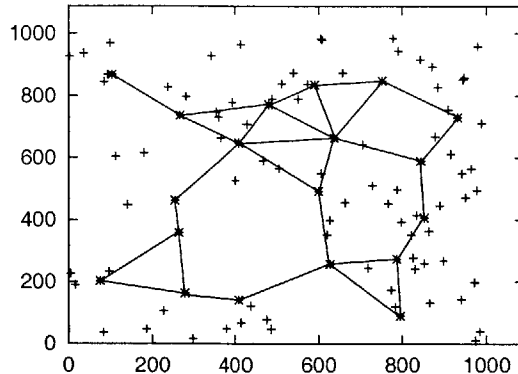
Figure 2-8: A scenario with 100 nodes, 19 coordinators, and a radio range of 250 meters. The nodes marked “*” are coordinators; the nodes marked “+” are non-coordinator nodes. Solid lines connect coordinators that are within radio range of each other.
