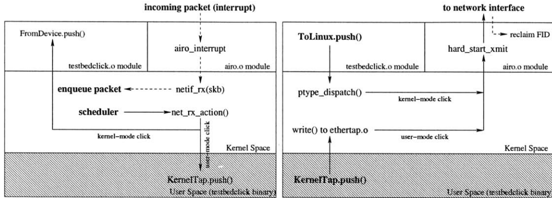
Figure 3-2: Left: the path of an incoming packet as it travels from the network interface to the Span layer of the networking stack. Right: the path of an outgoing packet as it travels from the Span layer of the networking stack to the network interface. Dotted lines indicate calls made in interrupt context; solid lines indicate calls made in process context. User space is shaded; kernel space is unshaded.
