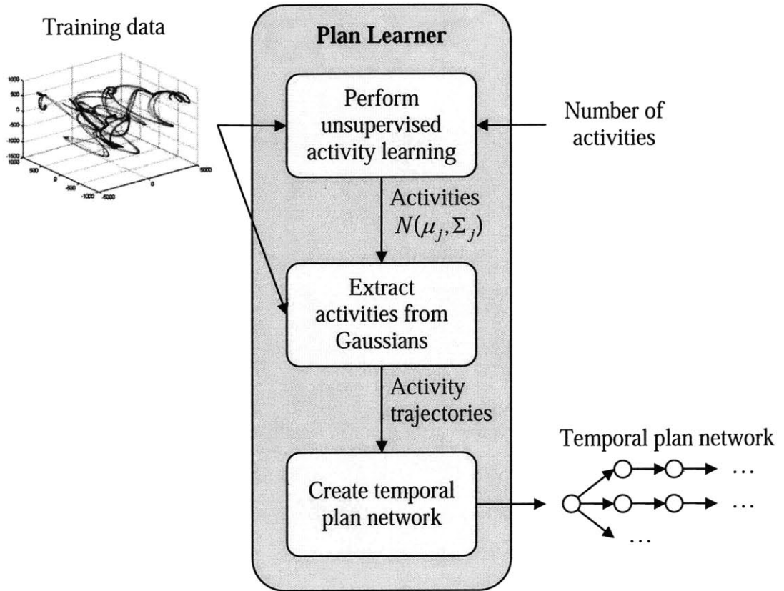
Figure 4-1: Overview of the plan learning process
