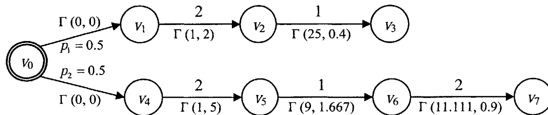
Figure 5-6: TPN of a simple example
