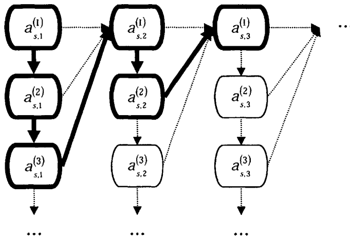
Figure 8-5: A most likely path in the HMM that we have cached
