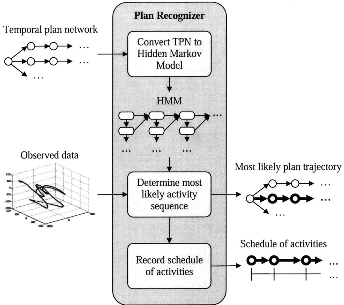
Figure 5-1: Overview of the plan recognition process
