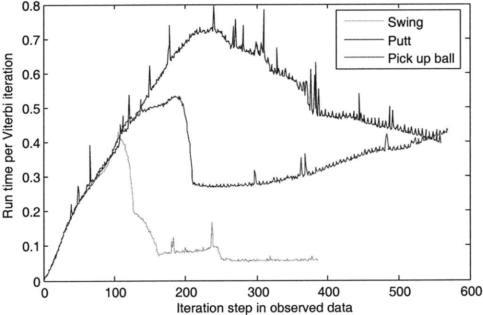
Figure 7-12: Run times for individual iterations during recognition for swing, putt, and pick up ball motions
