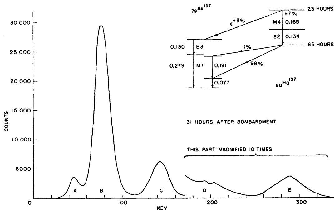
FIG. 1. \gamma spectrum of the samples and decay scheme of \text{Hg}^{197*} . Note.—The number at the extreme top-right-hand side of the figure should be 25 (hours) rather than 23 (hours).
