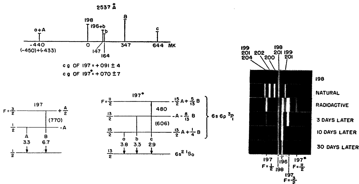
FIG. 3. The hyperfine structure of the 2537 Å line and the corresponding energy levels; decay of the radioactive components.
