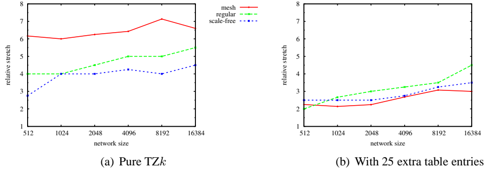
Figure 7-5: Maximum stretch relative to shortest-path routes
