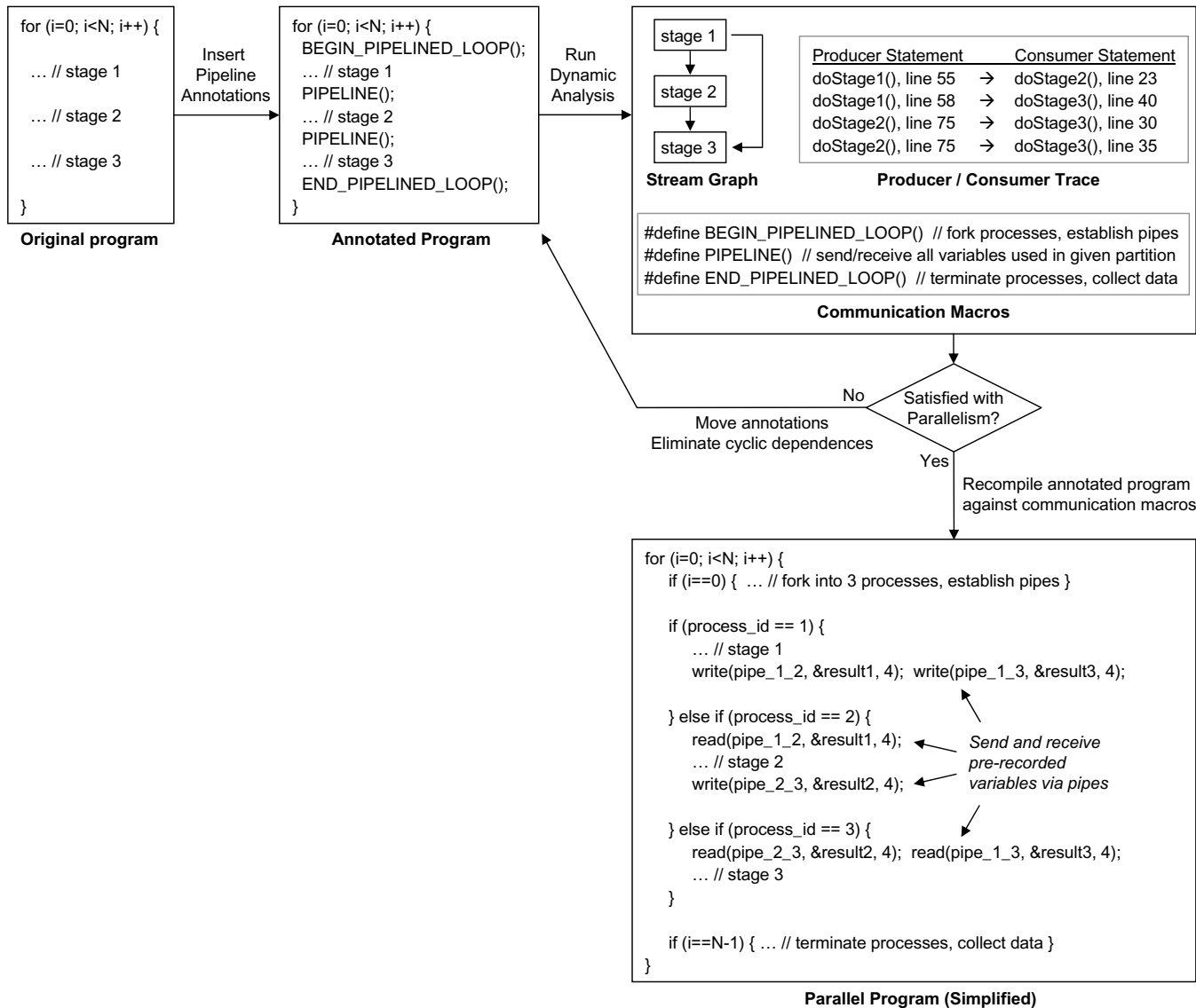
Figure 6-1: Overview of our approach.
