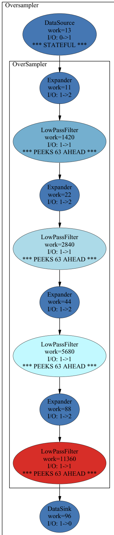
Figure B-54: Stream graph for Oversampler.
