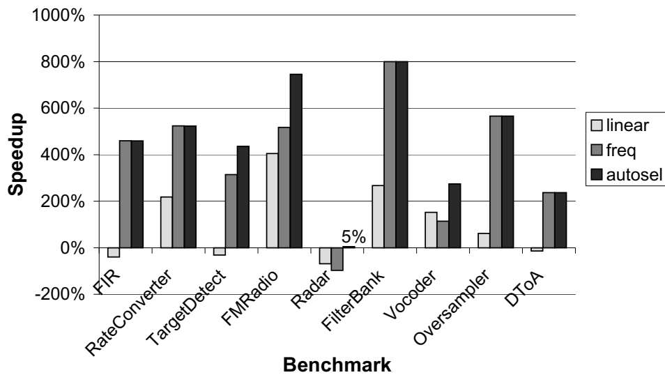
Figure 4-15: Execution speedup for maximal linear replacement, maximal frequency replacement, and automatic optimization selection 1 .
