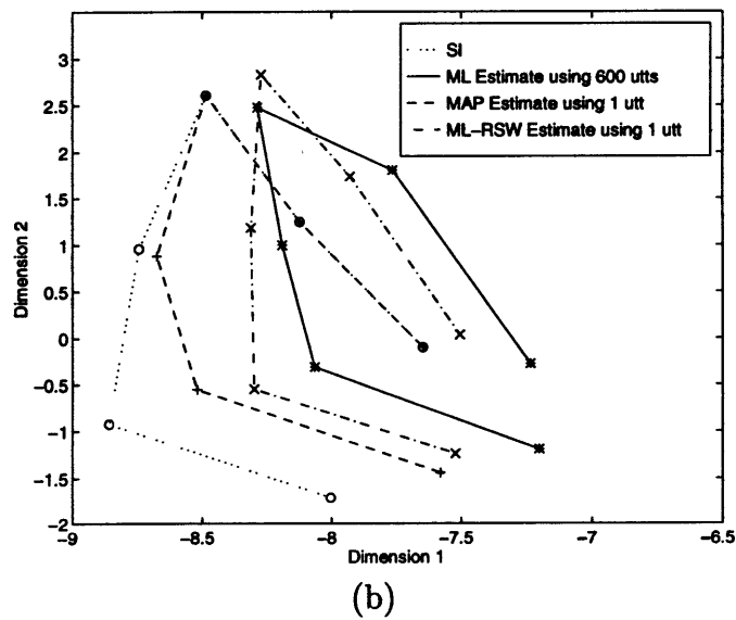
Figure 4.1: Location of center of mass for six different vowels ([i], [e], [æ], [a], [o], and [u]) for the following estimates: (1) the SI model, (2) the ML estimate from 600 adaptation utterances, (3) the MAP estimate from one adaptation utterance, and (4) the RSW estimate from one adaptation utterance.
