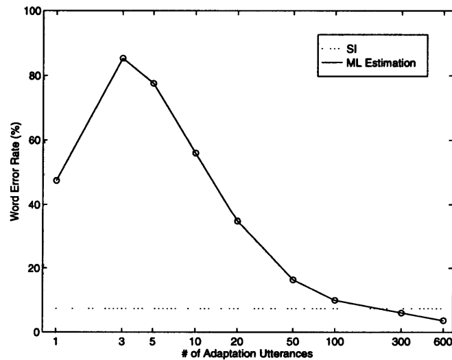
Figure 3.4: Performance of ML trained SD models as the number of adaptation utterances is varied from 1 to 600.
