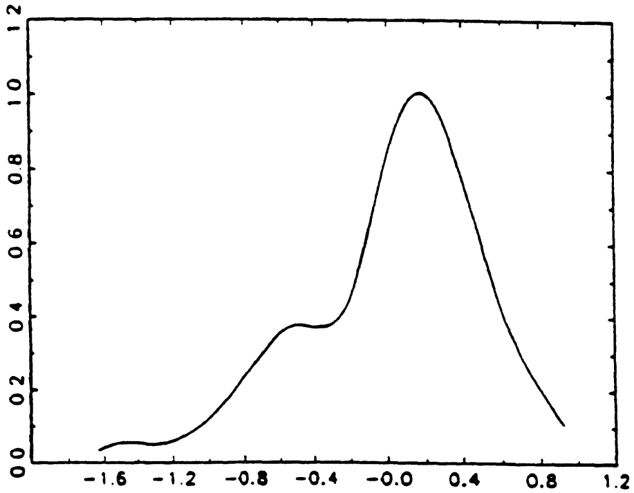
Figure 3.1 Single Index Function for Housing Data
