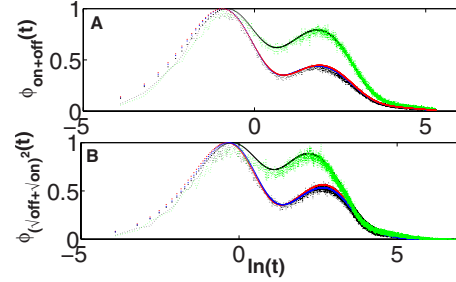
FIG. 6. (Color online) (A) The binned successive WT-PDFs for on-off events (lower curve), and the same WT-PDF from the randomized data. The fit for the randomized data is obtained from the amplitudes and rates of the \phi_x(t) 's. Two fit curves are shown for the actual data (blue and red, online), which overlap almost perfectly with each other and with the experimental curve. These curves are obtained from the direct fitting using our exponential-fit subroutine, and by further translating the found coefficients into the \sigma_{on+off} 's. (B) \phi_{(\sqrt{off}+\sqrt{on})^2}(t) for the randomized data (upper curve) and the actual data. The fit for the randomized data is based on the amplitudes and rates of the \phi_x(t) 's. The fits for the actual data are found from direct fitting, and by further translating the found coefficients into the matrix \sigma_{on,off} 's. Here, also, both fit curves overlap with each other and with the experimental curve.
