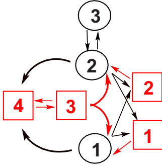
FIG. 3. (Color online) An irreversible transition KS with three off substates and four on substates. This is a rank 2 KS, with a corresponding RD form in Fig. 2(d).
