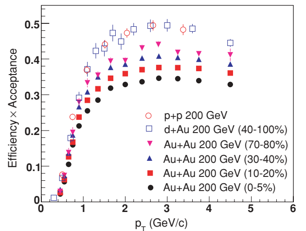
FIG. 4. (Color online) Reconstruction efficiency including acceptance of \phi meson as a function of p_T in several centrality bins for Au + Au, d + \text{Au} , and p + p 200 GeV collisions.
