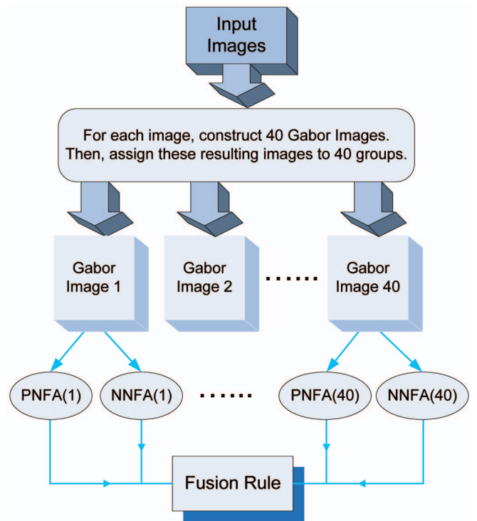
Fig. 2. The procedure of dual NFA-based multiple classifier framework. PNFA(i) and NNFA(i) mean performing PNFA and NNFA on the i th Gabor image.
