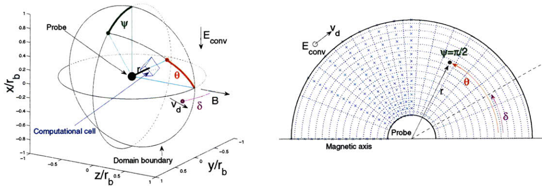
Figure III-2: (a) Three-dimensional view of the computational domain. (b) Cross-section at \psi = \pi/2 , half plane containing the drift velocity v_d . Computational cell centers for \cos \theta \leq 0 are indicated by "x"-symbols.
