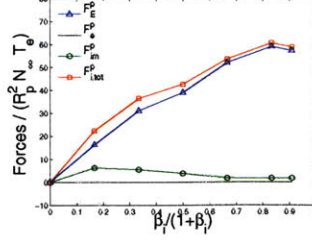
(e) v_d = 0.5c_{s0} , \lambda_{De} = 3
