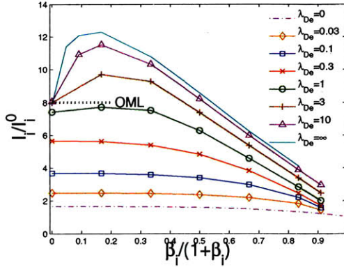
Figure VI-11: Total ion current normalized to I_i^0 = 4\pi N_\infty R_p^2 v_{ti}/2\sqrt{\pi} as a function of ion magnetization \beta_i , self-consistently calculated with SCEPTIC3D with \tau = 1 , \phi_p = -8 and \delta = \pi/2 . Curves labeled “ \lambda_{De} = 0 ” refer to quasineutral computations (chapter IV), and curves labeled “ \lambda_{De} = \infty ” to direct orbit integration (chapter V). (a) v_d = 0.2c_{s0} . (b) v_d = 0.5c_{s0} . (c) v_d = c_{s0} . (d) v_d = 1.5c_{s0} .
