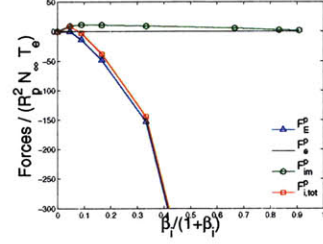
(i) v_d = c_{s0} , \lambda_{De} = 20
