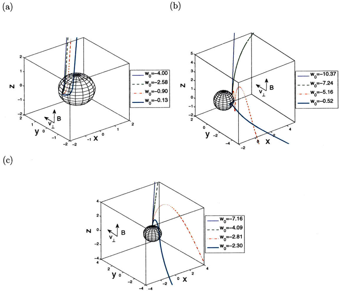
Figure V-4: Selection of 3D ion orbits, solutions of Sys. (V.28), traced backwards from the probe surface at (a) x = -1, z = 0^+ , (b) x = 1, z = 0^+ and (c) x = 0, y = 0, z = 1 . w_0 = v_0/v_{ti} is the “initial” backwards parallel velocity of the considered orbit. The simulation parameters for this example plots are \chi_p = 10 , \beta_i = 50 , and w_\perp = 0.5 .
