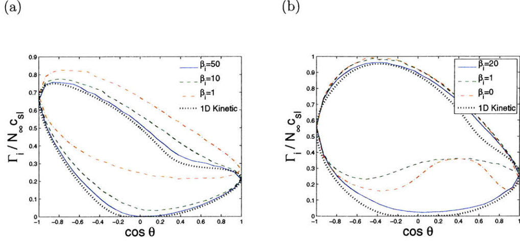
Figure IV-8: Angular ion-charge flux-density distribution to the probe major cross-section in the plane of flow and magnetic field \{0, \mathbf{e}_y, \mathbf{e}_z\} normalized to N_\infty c_{sI} , self-consistently calculated with SCEPTIC3D for different ion magnetizations \beta_i . “1D Kinetic” refers to the semi-analytic solution of chapter II. (a) \tau = 1 , v_d = c_{s0} and \delta = \pi/4 . (b) \tau = 0.1 , v_d = c_{s0} and \delta = 3\pi/8 .
