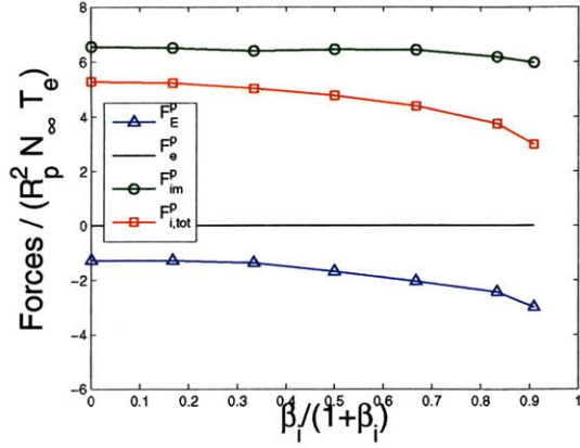
(c) v_d = 0.35c_{s0} , \mathbf{e}_x -axis
