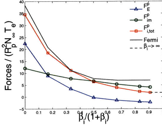
(c) \tau = 1, v_d = 1.5c_{s0}, \lambda_{De} = 20
