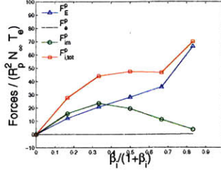
(k) v_d = 1.5c_{s0} , \lambda_{De} = 3
