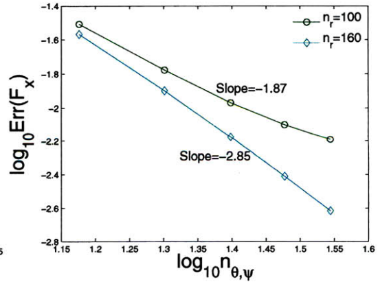
Figure III-7: Relative error on the probe-integrated Maxwell stress tensor computed by SCEPTIC3D in the “artificial” linear Poisson-Boltzmann regime, with r_b = 6 , \lambda_{De} = 0.5 , |\mathbf{E}_{\text{cnv}} R_p| = T_e/e . (a) Fixed angular resolutions, and (b) Fixed radial resolution.
