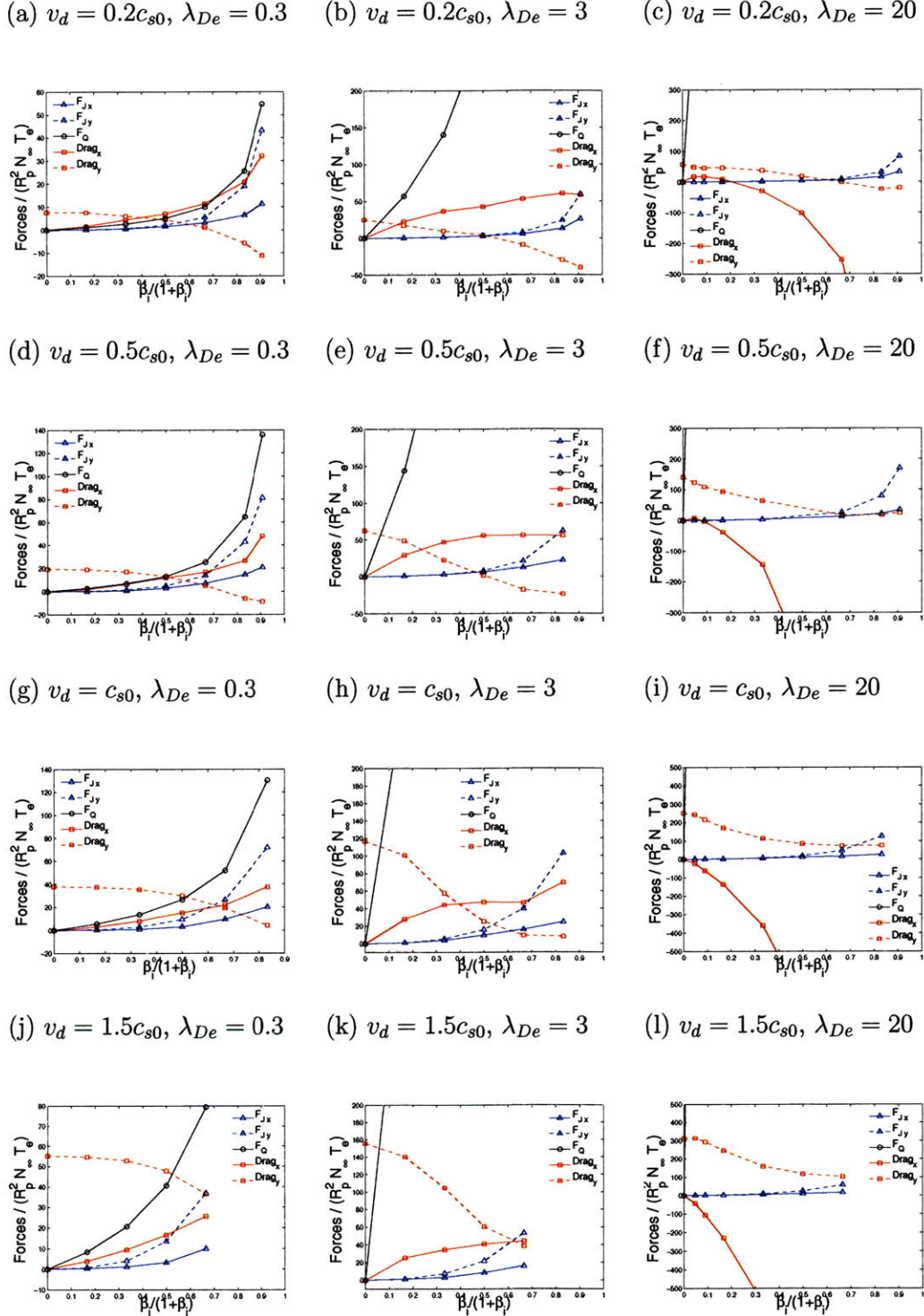
Figure VII-12: Comparison of the total ion-drag force computed by SCEPTIC3D with the parameters of Fig. (VII-10), with the non ion-drag forces \mathbf{F}_j and \mathbf{F}_Q . For easy reading, lines referring to forces acting along \mathbf{e}_x are solid, and dashed for \mathbf{e}_y .
