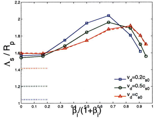
Figure VII-4: Effective shielding length \Lambda_s , such that the self-consistent dust capacitance computed by SCEPTIC3D is expressed as (VII.29). Solid lines correspond to pure cross-field flows ( \delta = \pi/2 ), and dashed lines to \delta = \pi/4 . The dotted limits at \beta_i = 0 are given by Eq. (VII.30).
