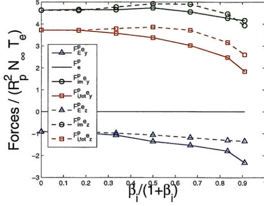
(c) v_d = 0.35c_{s0} , \mathbf{e}_x -axis
