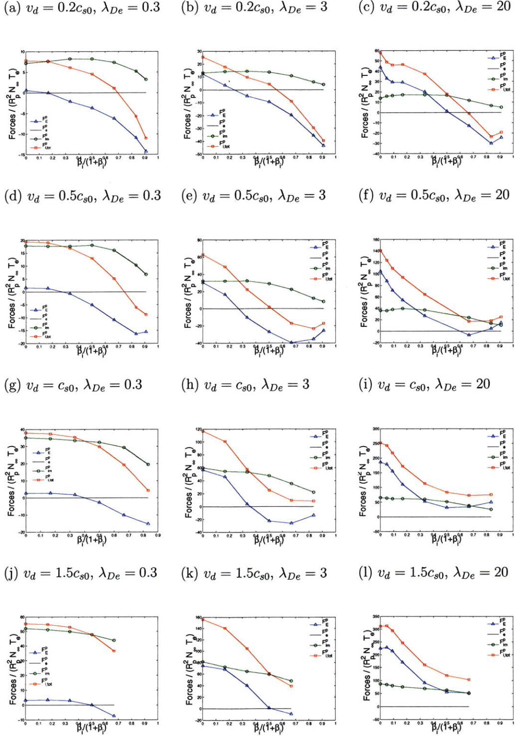
Figure VII-10: Self-consistent ion-drag computed at the dust surface by SCEPTIC3D along \mathbf{e}_y as a function of \beta_i with \tau = 1 , \phi_p = -8 , \delta = \pi/2 , and variable \lambda_{De} and v_d .
