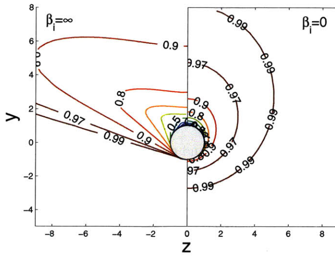
Figure II-15: Analytic free-flight charge-density contours at infinite (Eq. (II.82)) and zero (Eq. (II.88)) ion magnetization, for the case w_d = w_\perp = 0.5 and w_\infty = 0 .
