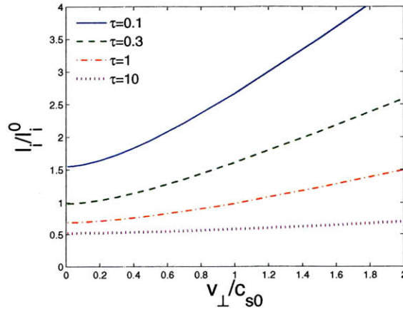
Figure V-7: Total (i.e. sphere-integrated) ion current normalized to I_i^0 = 4\pi R_p^2 N_{\infty} v_{ti} / 2\sqrt{\pi} , solution of the collisionless quasineutral 1D-kinetic model of chapter II (kinetic equation (II.50), valid when \beta_i \rightarrow \infty and \Lambda_{De} \ll R_L ) with v_{\infty} = 0 . Except in the limit \tau \gg 1 , the ion current at v_{\perp} = 0 is higher than the geometric limit I_i^0/2 .
