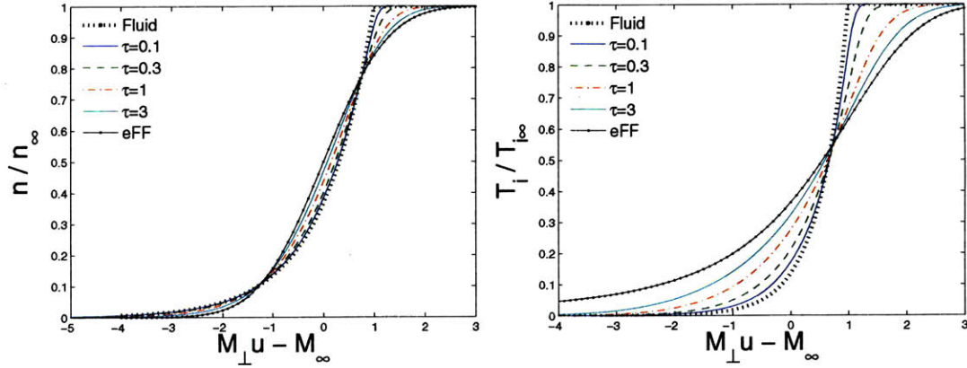
Figure II-8: Evolution of the electron density and ion temperature along the presheath parametrized by \mu_I = M_{\perp} u - M_{\infty} , for different temperature ratios. “Fluid” refers to Hutchinson’s fluid solution, and “eFF” to the extended free-flight solution described in Paragraph II.4.4.
