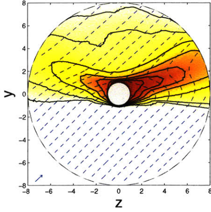
(c) \tau = 0.1, v_d = 0.5c_{s0}, \delta = \pi/4
