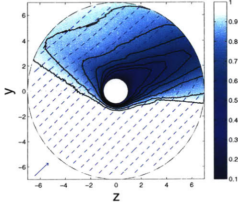
(c) \lambda_{De} = 0.3
