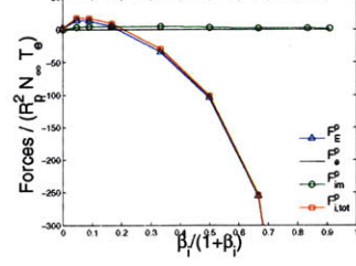
(f) v_d = 0.5c_{s0} , \lambda_{De} = 20
