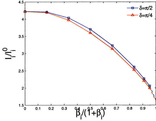
(c) \tau = 0.1, v_d = c_{s0}
