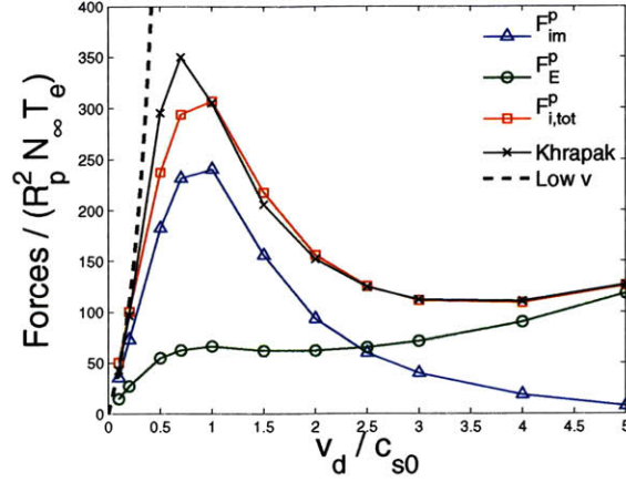
Figure VII-1: Comparison of ion-drag force computed by SCEPTIC(2D) ( \mathbf{F}_i^P , decomposed in \mathbf{F}_{im}^P and \mathbf{F}_E^P ) with Khrapak’s analytic solution (sum of \mathbf{F}_{im}^\infty (Eq. (VII.7)) and \mathbf{F}_E^\infty (Eq. (VII.13)) with \ln \Lambda given by Eq. (VII.17), and the low velocity limit (VII.20)). The parameters are \tau = 0.1 , \phi_p = -4 , and \lambda_{De} = 20 .
