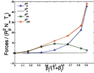
(g) v_d = c_{s0} , \lambda_{De} = 0.3
