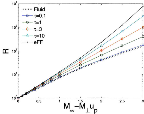
Figure II-11: Upstream to Downstream flux ratio against M_\infty - M_\perp u_p \in [0, 3] , for different temperature ratios. The tangents of the flux ratio logarithms at the origin have a slope given by 1/M_c(\tau) .
