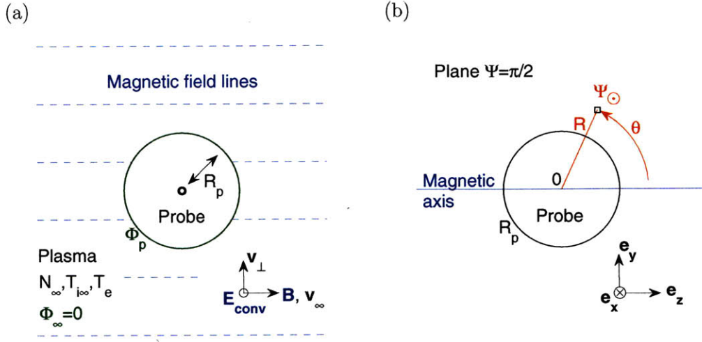
Figure III-1: (a) Problem parameters in their geometry, in the \{0, e_y, e_z\} -plane. (b) Spherical and Cartesian coordinate systems, projected on the plane of flow and magnetic field ( \psi = \pi/2 ).
