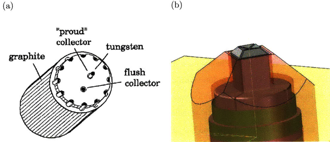
Figure II-4: (a) Drawing of the probe on which the term Gundestrup has been coined [21]; twelve tungsten pins span the tip of a cylindrical head. (b) CAD view of the WASP (Wall Actuated Scanning Probe), a four-electrode Gundestrup probe installed in the inner wall of the Alcator C-Mod tokamak [22].
