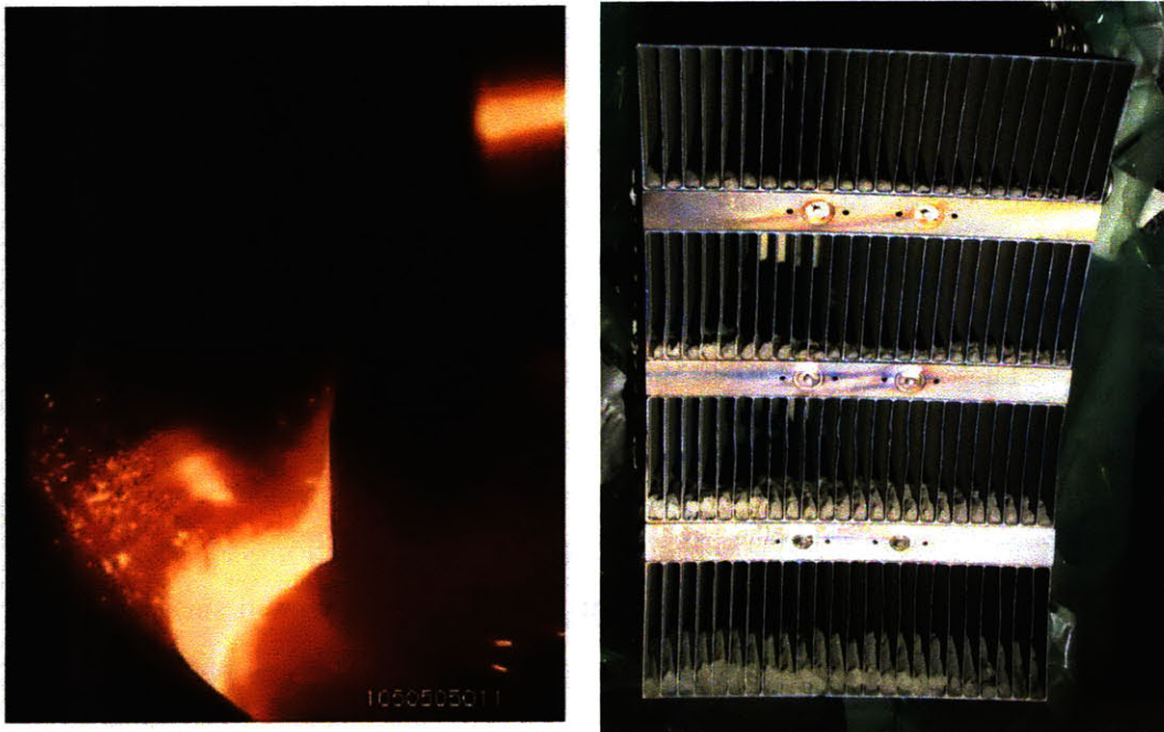
Figure V-2: In the 2005 Alcator C-mod tokamak campaign, the lower hybrid launcher experienced corrosion by hydrogen and deuterium, spewing titanium dust across the machine. (a) Dust particles in visible light (red dots), as they radiate before eventually melting. (b) Dust deposited on the launcher after plasma operation.
