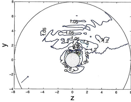
(c) T_{i,xx}, \lambda_{De} = 3
