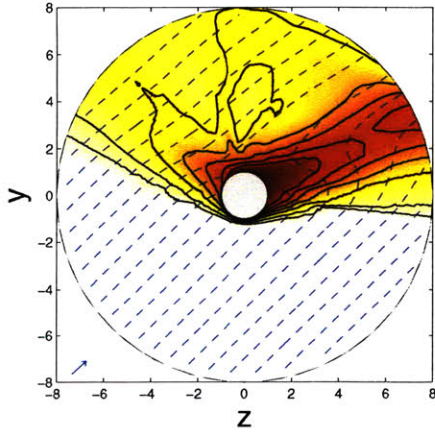
Figure IV-2: Selection of charge-density contour-plots in the \{0, \mathbf{e}_y, \mathbf{e}_z\} -plane, with strongly magnetized ions \beta_i = 20 (except in (b) where a comparison with the magnetic-free regime is provided). Iso-density contours for n = 0.4, 0.5, 0.6, 0.7, 0.8, 0.9, 0.95 are full black, while fluid stream lines are dashed blue. The external velocity is indicated by a blue arrow on the figures' lower left corners.
