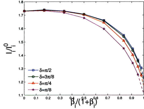
Figure IV-7: Total ion saturation current normalized to I_i^0 = 4\pi R_p^2 N_\infty v_{ti} / 2\sqrt{\pi} as a function of ion magnetization \beta_i , self-consistently calculated with SCEPTIC3D. (a) \tau = 0.1, v_d = 0.2c_{s0} . (b) \tau = 1, v_d = 0.5c_{s0} . (c) \tau = 0.1, v_d = c_{s0} . (d) \tau = 1, v_d = 1.5c_{s0} . The dashed portions of curves at high \beta_i connect our simulations at finite magnetization to I_i^{|\beta_i|=\infty} (Eq. (IV.3) with \Gamma_{i||}^{|\beta_i|=\infty} from chapter II).
