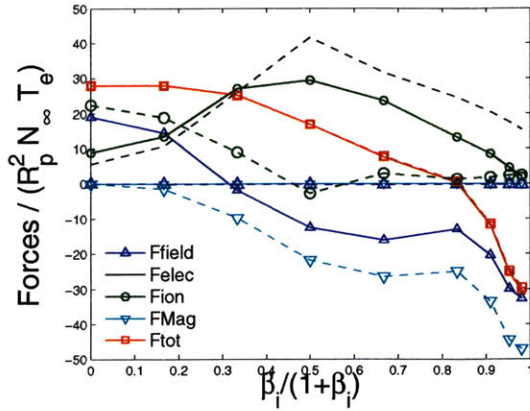
(c) e_d -axis
