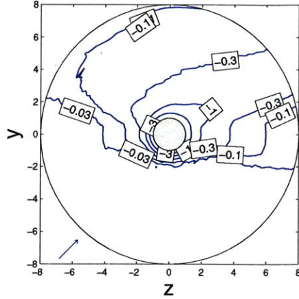
(c) \{0, \mathbf{e}_y, \mathbf{e}_z\} , \lambda_{De} = 3
