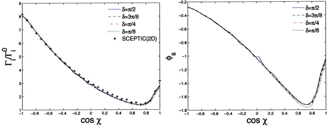
Figure III-5: (a) Ion saturation flux and (b) sheath entrance potential as a function of the position projected on the drift axis ( \cos\chi ), for the case \tau = 0.1 , v_d = c_{s0} , \beta_i = 0 and a selection of \delta s. The points labeled “SCEPTIC(2D)” correspond to the solution from the appendix in Ref. [9]. SCEPTIC3D runs have been performed with r_b = 8 , n_r = 120 , n_\theta = n_\psi = 30 , and n_{\text{part}} = 51.2M .
