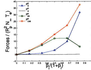
(j) v_d = 1.5c_{s0} , \lambda_{De} = 0.3
