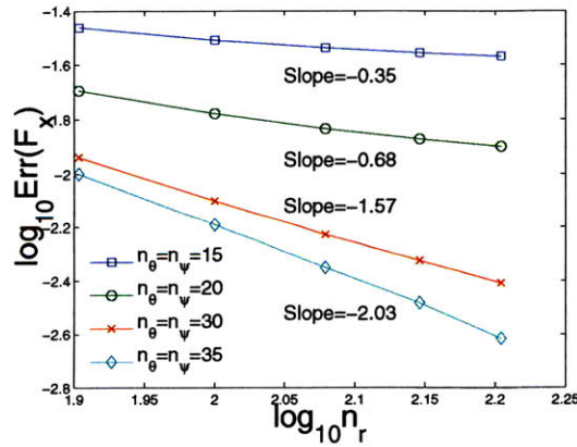
Figure III-7: Relative error on the probe-integrated Maxwell stress tensor computed by SCEPTIC3D in the “artificial” linear Poisson-Boltzmann regime, with r_b = 6 , \lambda_{De} = 0.5 , |\mathbf{E}_{\text{cnv}} R_p| = T_e/e . (a) Fixed angular resolutions, and (b) Fixed radial resolution.
