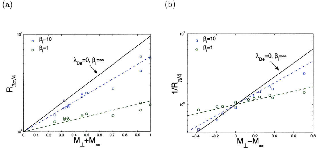
Figure VI-15: Upstream to downstream flux ratios on the probe major cross-section at (a) \eta = 3\pi/4 and (b) \eta = \pi/4 , versus respectively M_{\perp} + M_{\infty} and M_{\perp} - M_{\infty} , from a large set of SCEPTIC3D runs spanning v_d \in [0 : 1]c_{s0} and \delta \in [\pi/8 : \pi/2] , for \tau = 1 , \lambda_{De} = 0.1 , and \phi_p = -8 . Also shown are the corresponding fitting lines, whose slopes 1/M_c are taken from Fig. (VI-16a).
