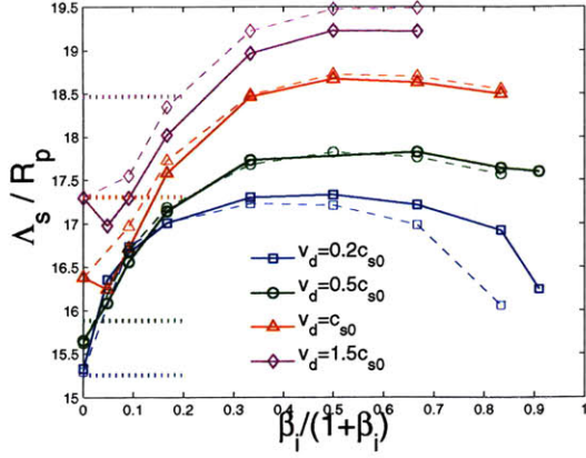
(c) \tau = 1, \lambda_{De} = 0.1
