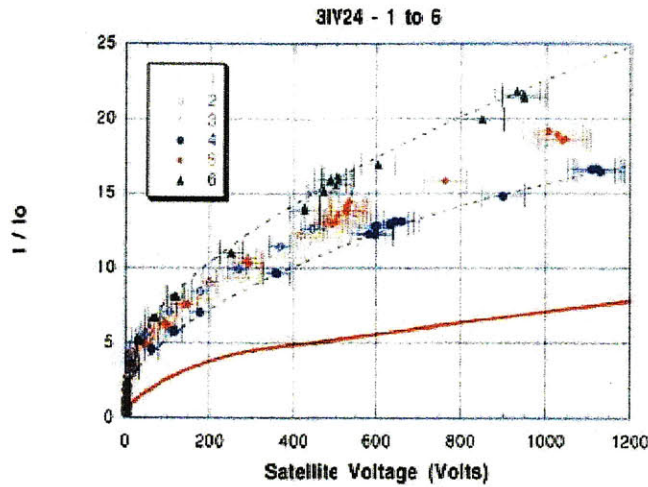
Figure VI-2: Compilation of Current-Voltage characteristics from the TSS-1R experiment (colour version of Fig. (2) in Ref. [57]). The points correspond to different voltage sweeps, and the thick red line to the Parker-Murphy upper bound (Eq. (V.44)).
