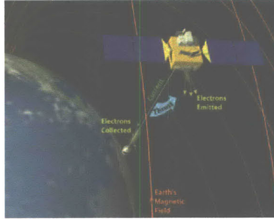
Figure VI-1: Artist view of the Electro Dynamic Tether concept (From http://www.tethers.com/EDTethers.html ).
