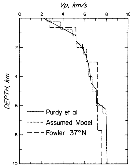
Fig. 6. Velocity-depth models. The solid line shows the preliminary velocity-depth function obtained from refraction data along the profile shown in Figure 1 [Purdy et al. , 1982]. The dashed line shows the plane-layered structure assumed for calculating microearthquake locations. The velocity structure determined by Fowler [1976] for the median valley of the Mid-Atlantic Ridge near 37°N is also shown. See text for a discussion of the effects of varying the assumed velocity model on hypocenter determinations.
