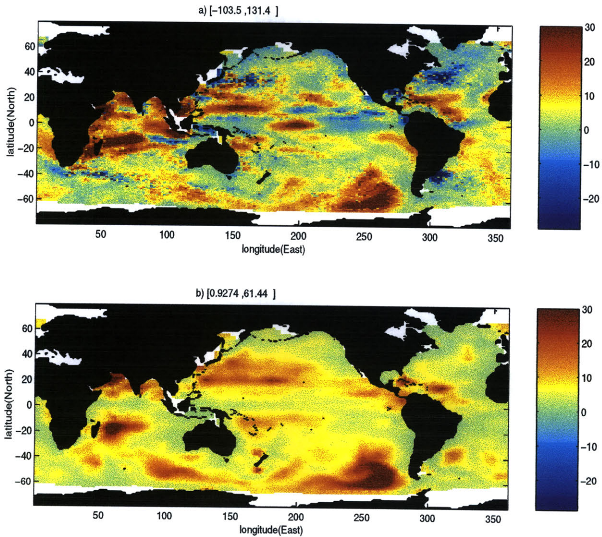
Figure 5.2: Variance of the projection of the model error onto the sea level in \text{cm}^2 ( \text{diag HPH}^T ) a) from equation (5.10) and b) for the \mathbf{Q} actually used in F99. The correlation between the two fields is 0.56. The minimum and maximum values are given in the square brackets.
