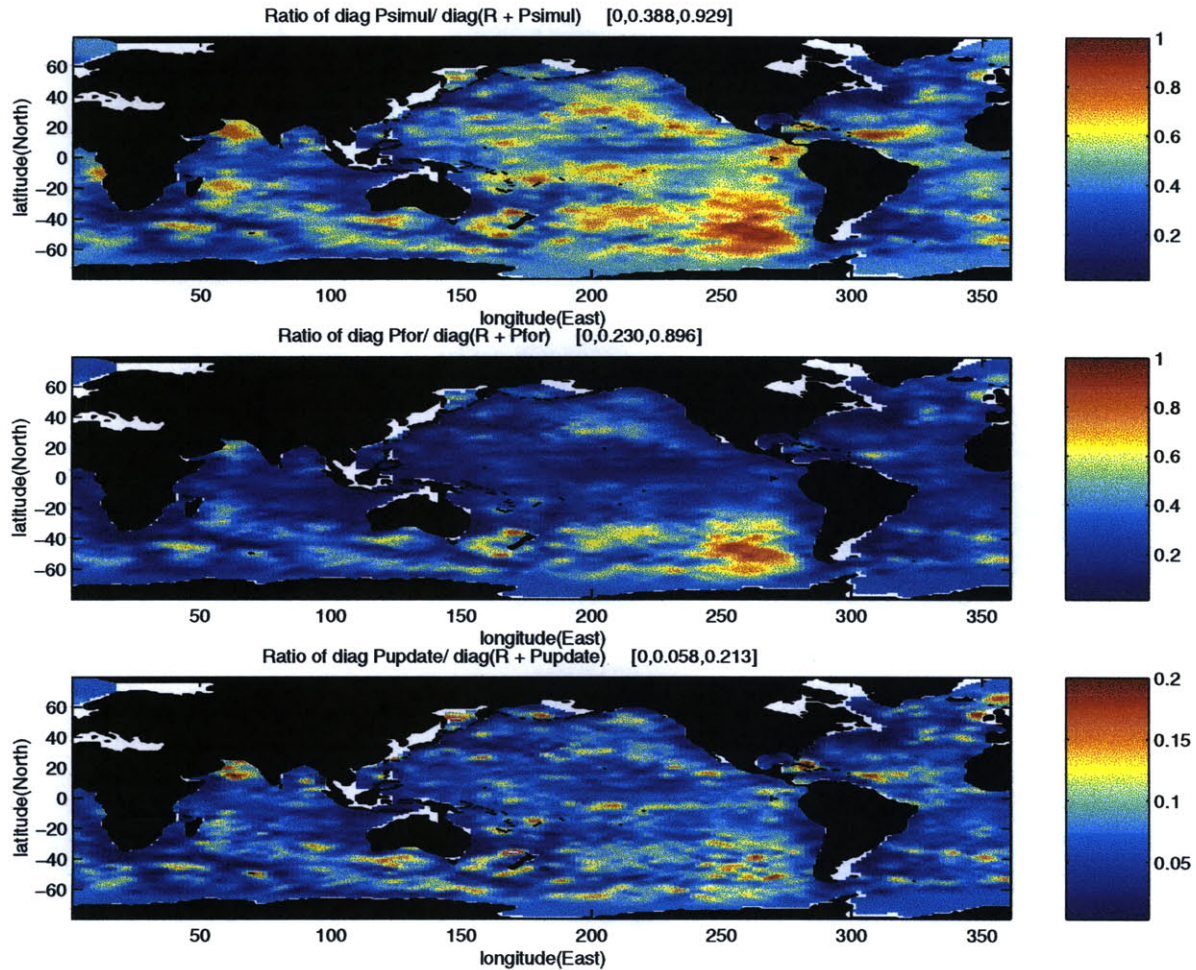
Figure 5.8: Relative ratio of the model and measurement errors for the rescaled covariance model used by F99 for : a) the model error (simulation error) \text{diag} \mathbf{H} \mathbf{P} \mathbf{H}^T / (\text{diag} \mathbf{H} \mathbf{P} \mathbf{H}^T + \text{diag} \mathbf{R}) ; b) forecast error forecast \text{diag} \mathbf{H} \mathbf{\Pi}_s(-) \mathbf{H}^T / (\text{diag} \mathbf{H} \mathbf{\Pi}_s(-) \mathbf{H}^T + \text{diag} \mathbf{R}) ; c) update error \text{diag} \mathbf{H} \mathbf{\Pi}_s(-) \mathbf{H}^T / (\text{diag} \mathbf{H} \mathbf{\Pi}_s(-) \mathbf{H}^T + \text{diag} \mathbf{R}) . Values greater than one half indicate that most residual variance is explained by the model error, and less than one half by the measurement error (which includes representation error). The minimum, mean and maximum values are given in the square brackets.
