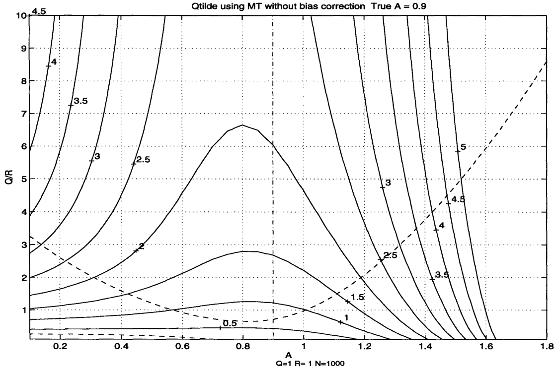
Figure 2.8: The contour plot of \tilde{q}_{\text{mt,biased}} , without the bias correction, as a function q and A for a case when we have a correct estimate of R , the true model is \hat{A} = 0.9 (dash-dotted vertical line), and the ratio \hat{q} is 1. Dashed lines represent the values to which the algorithm will converge depending on the choice of the model A .
