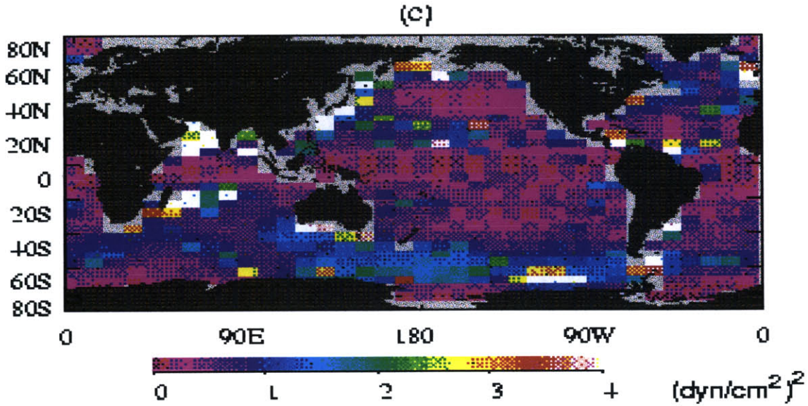
Figure 5.3: Variance of the NCEP wind stress(from F99).
