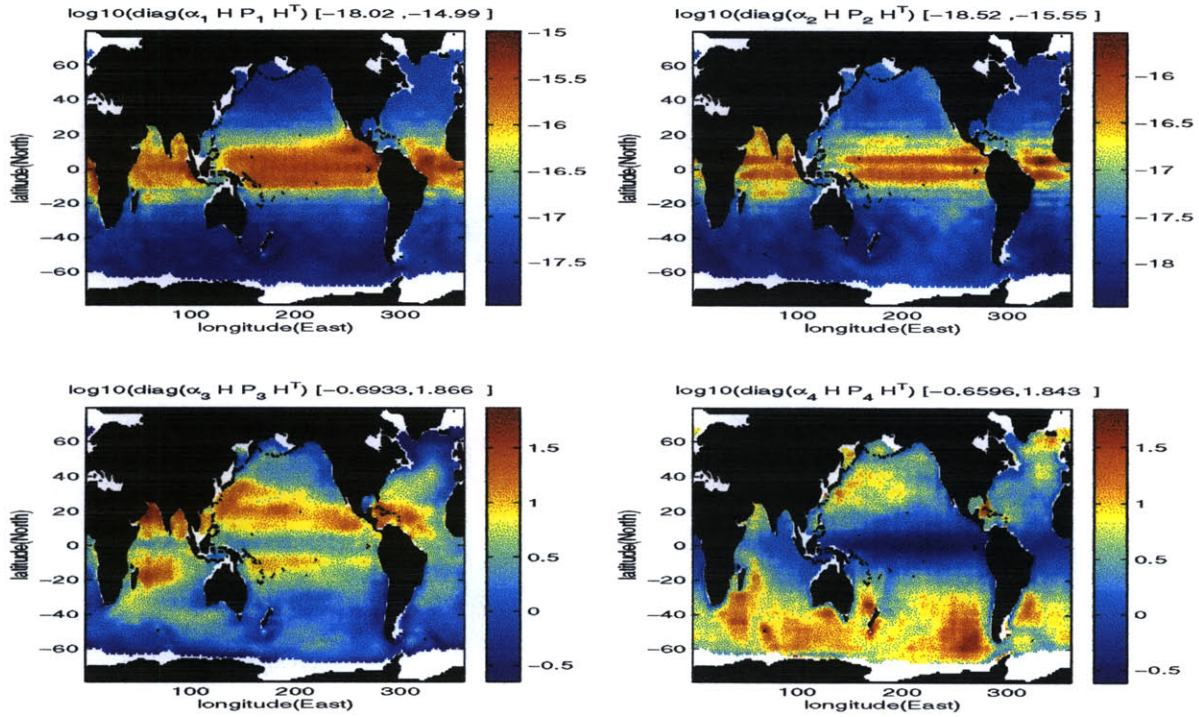
Figure 5.15: Log10 of diagonals of \alpha_k \mathbf{H} \mathbf{P}_k \mathbf{H}^T . The covariance model consists of four diagonal matrices for \mathbf{Q} and the measurement error covariance used in F99. The estimates were obtained using \mathbf{Y} and \mathbf{D}_3 . Note the top two plots are zero, and are presented only to show the signature for the baroclinic velocities u and v . The minimum and maximum values are given in the square brackets.
