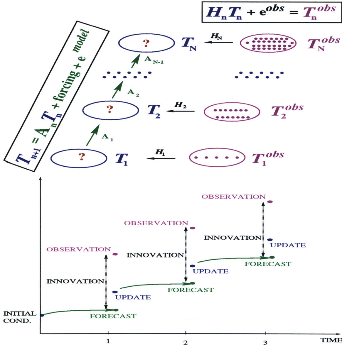
Figure 2.5: Two graphical representations of the Kalman filter. Top) T_n represents all model variables, T_n^{\text{obs}} represents observations, A_n dynamical model which forecasts T_{n+1} using T_n , H_n projection operator which maps model variables onto observations at time n . Both model and measurement equations have errors, e^{\text{model}} and e^{\text{obs}} , respectively. The average magnitudes of these errors (given by their covariances) are used as weighting matrices to obtain the best possible estimate at time n , denoted by the question mark, which is then propagated forward to obtain the forecast at time n + 1 . Bottom) Alternative view of the Kalman filtering. Starting from the initial condition at time 0, we obtain the forecast at time 1, and then get a weighted average of the forecast and the observations (the difference is called innovation vector) to obtain the update state at time 1. This update is then used as initial condition and the model is propagated again to give a forecast at time 2, and so on.
