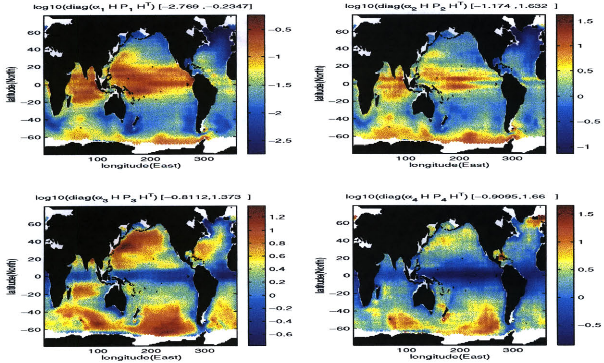
Comparison of contributions of HP,kH,T using Qtype 16 Rtype 21 w. 1 - 32624 of d
