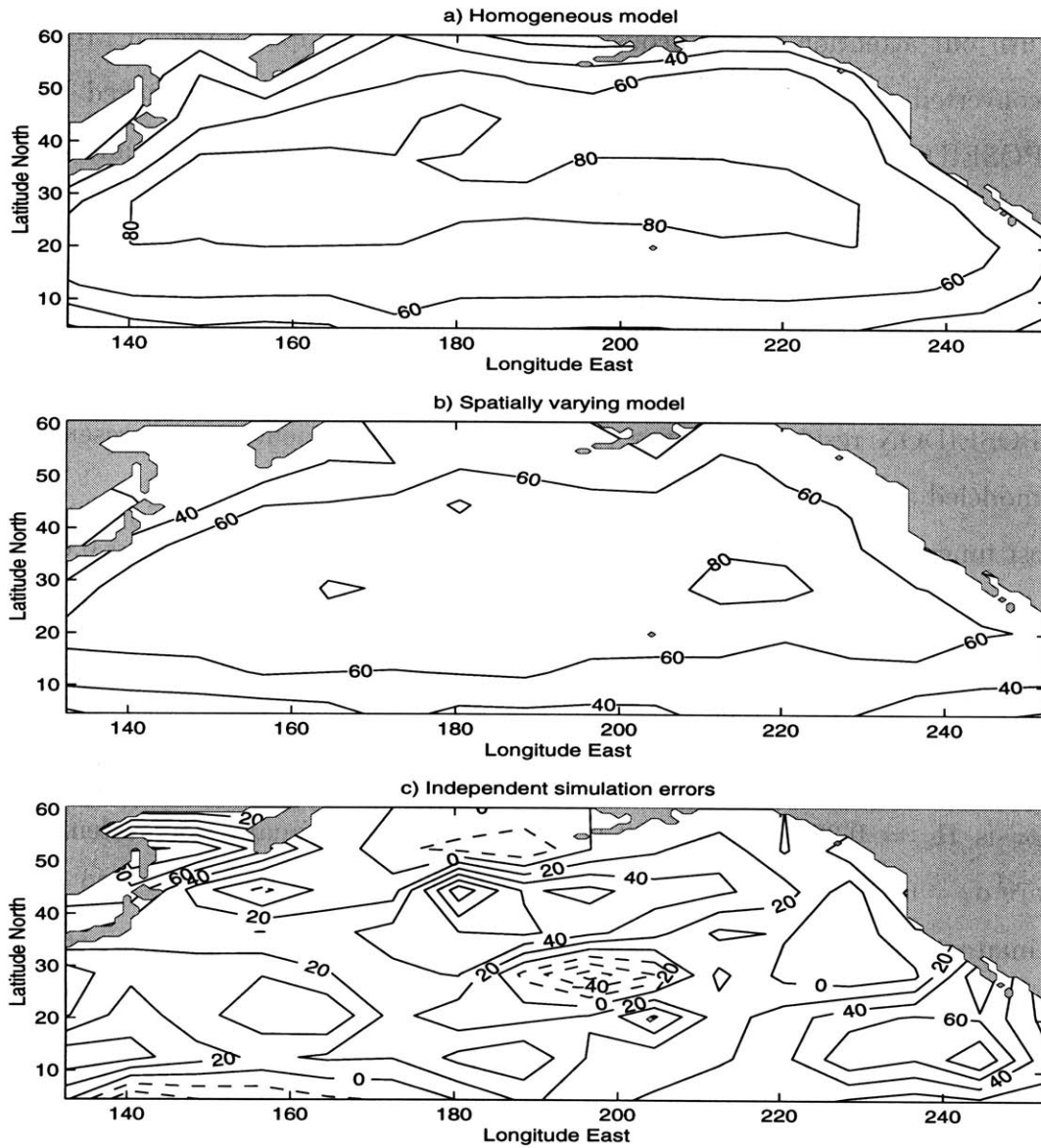
Figure 4.5: Prior estimate for percent variance of GCM-TOPEX/POSEIDON residual which is explained by system error, that is, ratio of diagonal elements of \mathbf{H}\mathbf{P}\mathbf{H}^T in (3.6) to those of \mathbf{Y} . The estimates are obtained using the covariance matching method for a) a homogeneous model for the errors, b) a spatially varying model, and c) the model proposed by Fu et al. (1993) which assumes that the GCM simulation errors are independent from the ocean state. Contour intervals are 20%. Spurious negative regions in c) (dashed contours) result from the large uncertainty of the sample covariance matrices used in the analysis.
