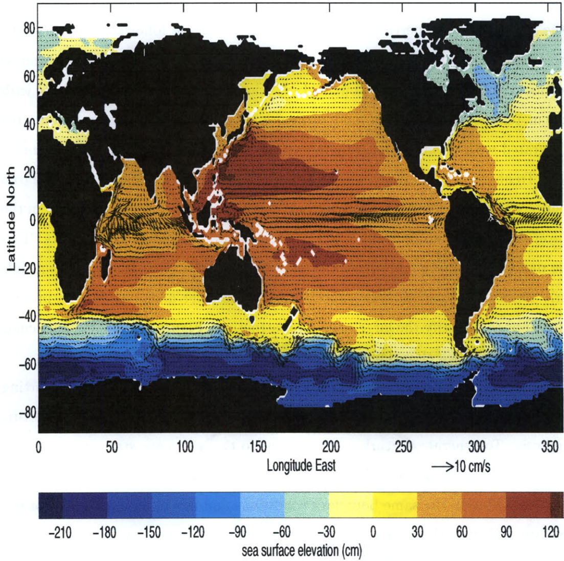
Figure 2.3: July monthly-mean sea surface elevation and horizontal velocity in the 2nd layer produced by the MIT GCM run.
