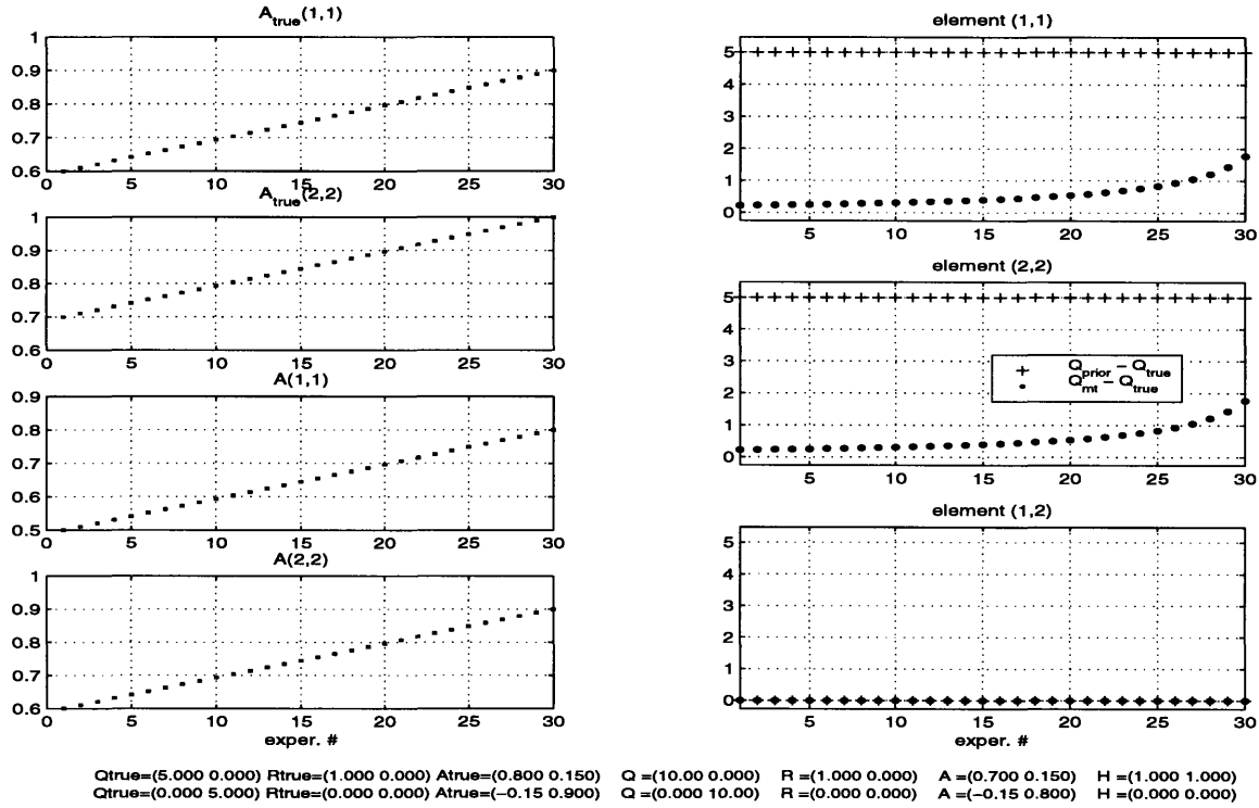
EXPER 109: R=Rtrue RECURSIVE w. 1 param. estim.
