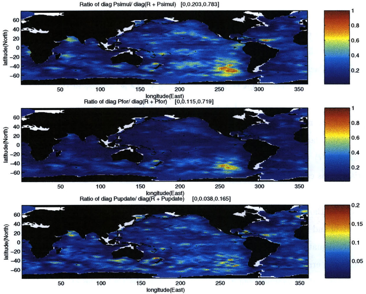
Figure 5.4: Relative ratio of the model and measurement errors for the covariance model used by F99 for : a) the model error (simulation error) \text{diag} \mathbf{H} \mathbf{P} \mathbf{H}^T / (\text{diag} \mathbf{H} \mathbf{P} \mathbf{H}^T + \text{diag} \mathbf{R}) ; b) forecast error forecast \text{diag} \mathbf{H} \mathbf{\Pi}_s(-) \mathbf{H}^T / (\text{diag} \mathbf{H} \mathbf{\Pi}_s(-) \mathbf{H}^T + \text{diag} \mathbf{R}) ; c) update error \text{diag} \mathbf{H} \mathbf{\Pi}_s(-) \mathbf{H}^T / (\text{diag} \mathbf{H} \mathbf{\Pi}_s(-) \mathbf{H}^T + \text{diag} \mathbf{R}) . Values greater than one half indicate that most residual variance is explained by the model errors, and less than one half by the measurement error (which includes representation error). The minimum, mean and maximum values are given in the square brackets.
