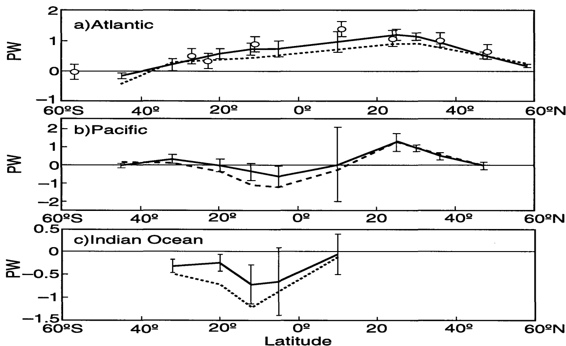
Figure 1.1: Meridional heat transport (in 10^{15} W) for July-December 1993 estimated from global data assimilation with the MIT model and T/P data (solid lines). The unconstrained model for the Atlantic, the Pacific and the Indian Ocean respectively, are shown with the dashed lines. Bars on the solid lines show RMS variability of the transport estimated over individual 10-day periods (reproduced from Stammer et al. 1997).
