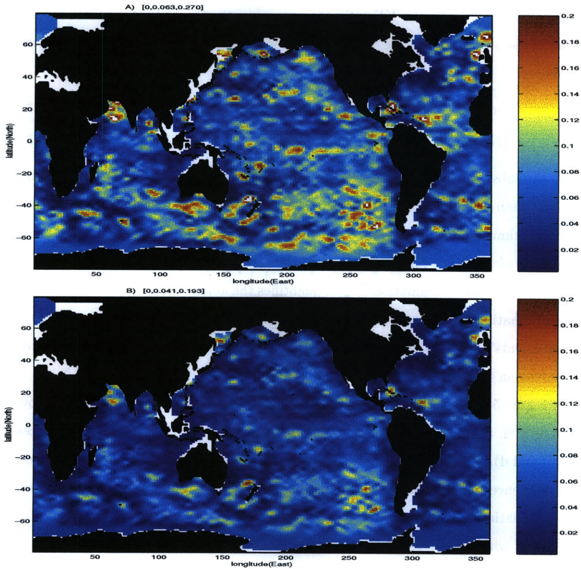
Figure 5.9: Sea level anomaly (cm) associated with Kalman filter changes in model state corresponding to an instantaneous 1 cm model–data difference for a) the rescaled error covariances of F99, b) the original error covariances of F99. The estimates are strictly local reflecting sea level difference at each separate grid point and assuming the instantaneous data distribution used to derive the time-asymptotic limit of the KF.
