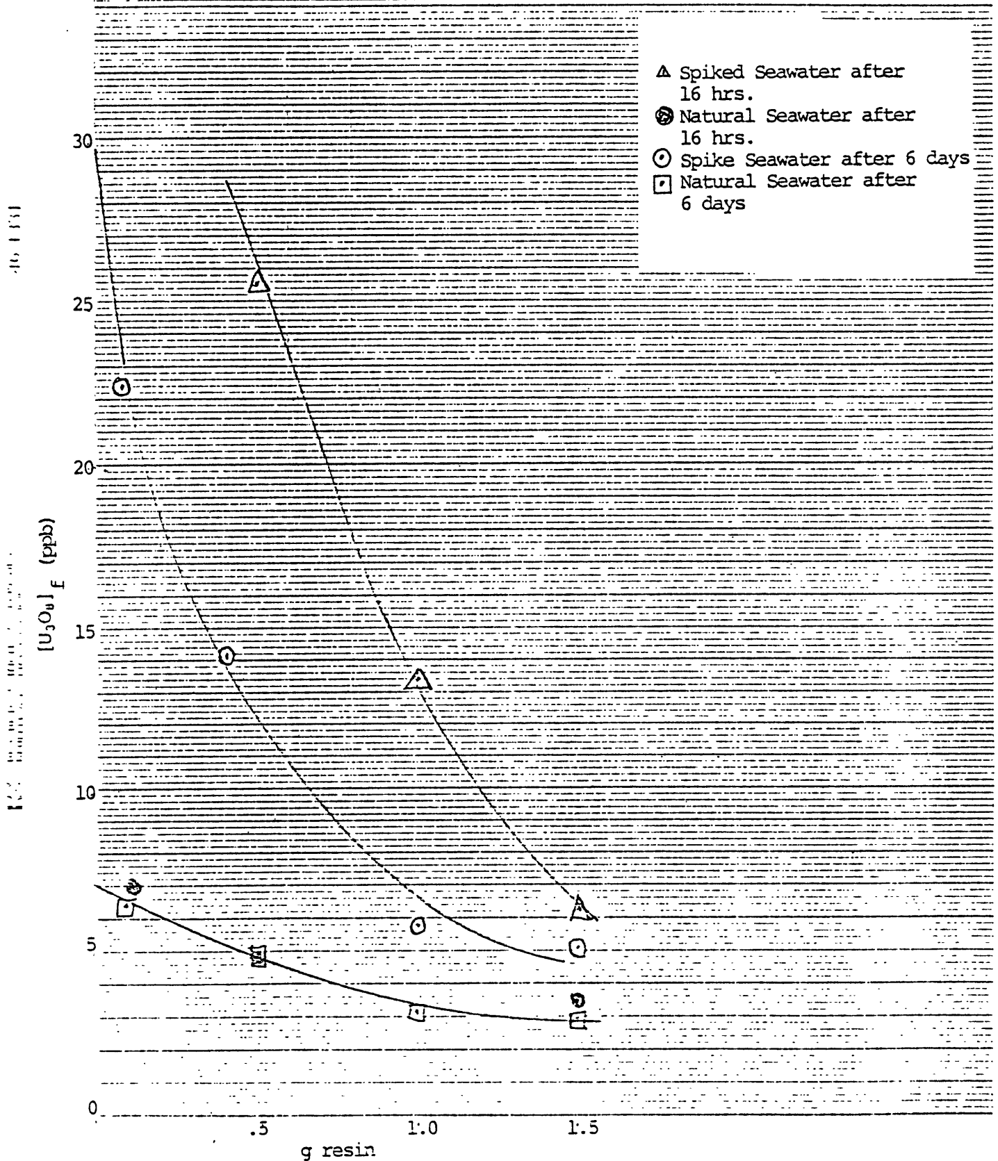
Figure 4 Uranium Concentration at 16 hrs. and 6 Days of Contact with Various Amounts of XE318
