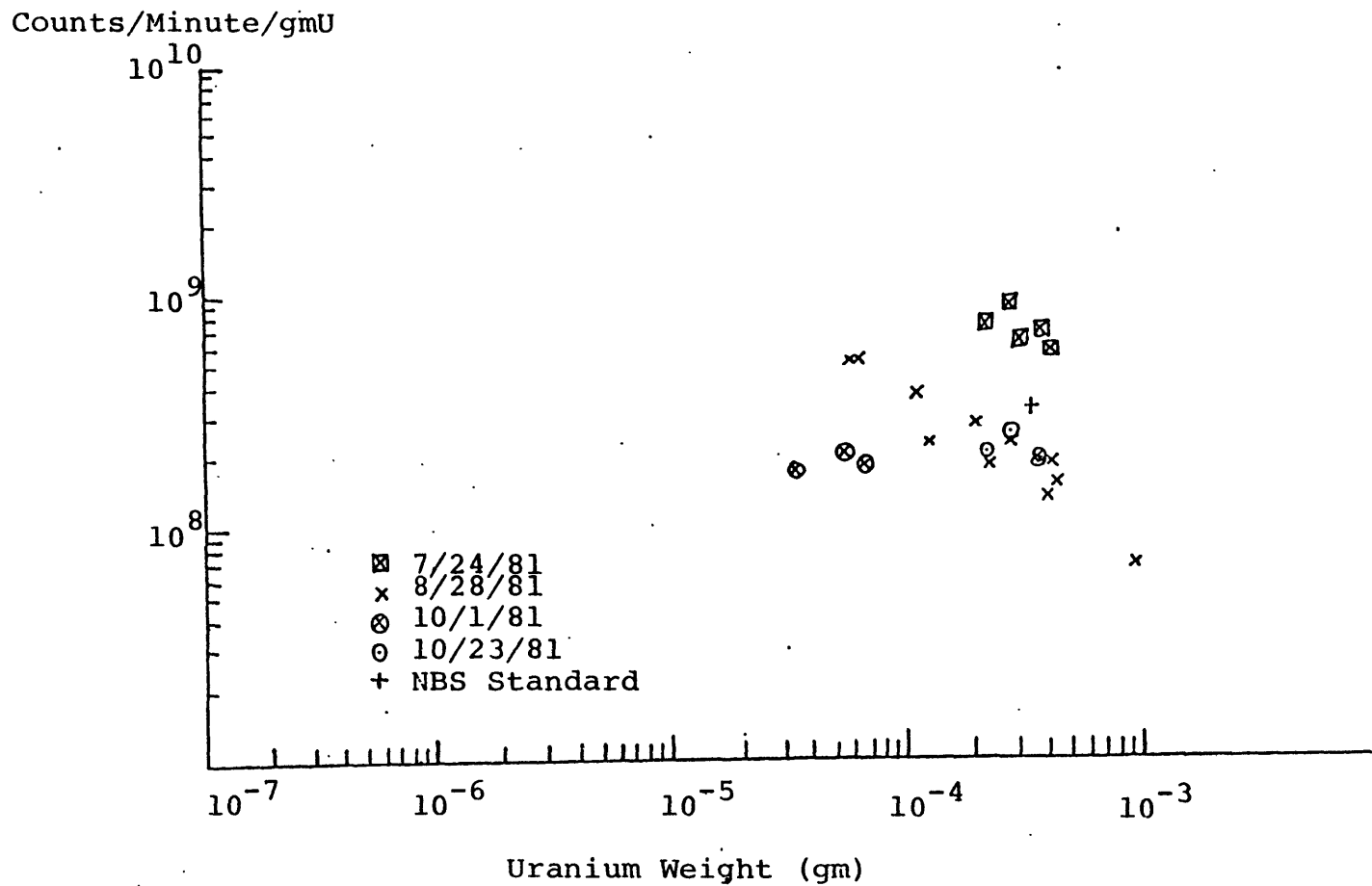
Fig. 2.9 Uranium Dioxide as a Calibration Standard: Cts/min/gmU versus Uranium Weight
