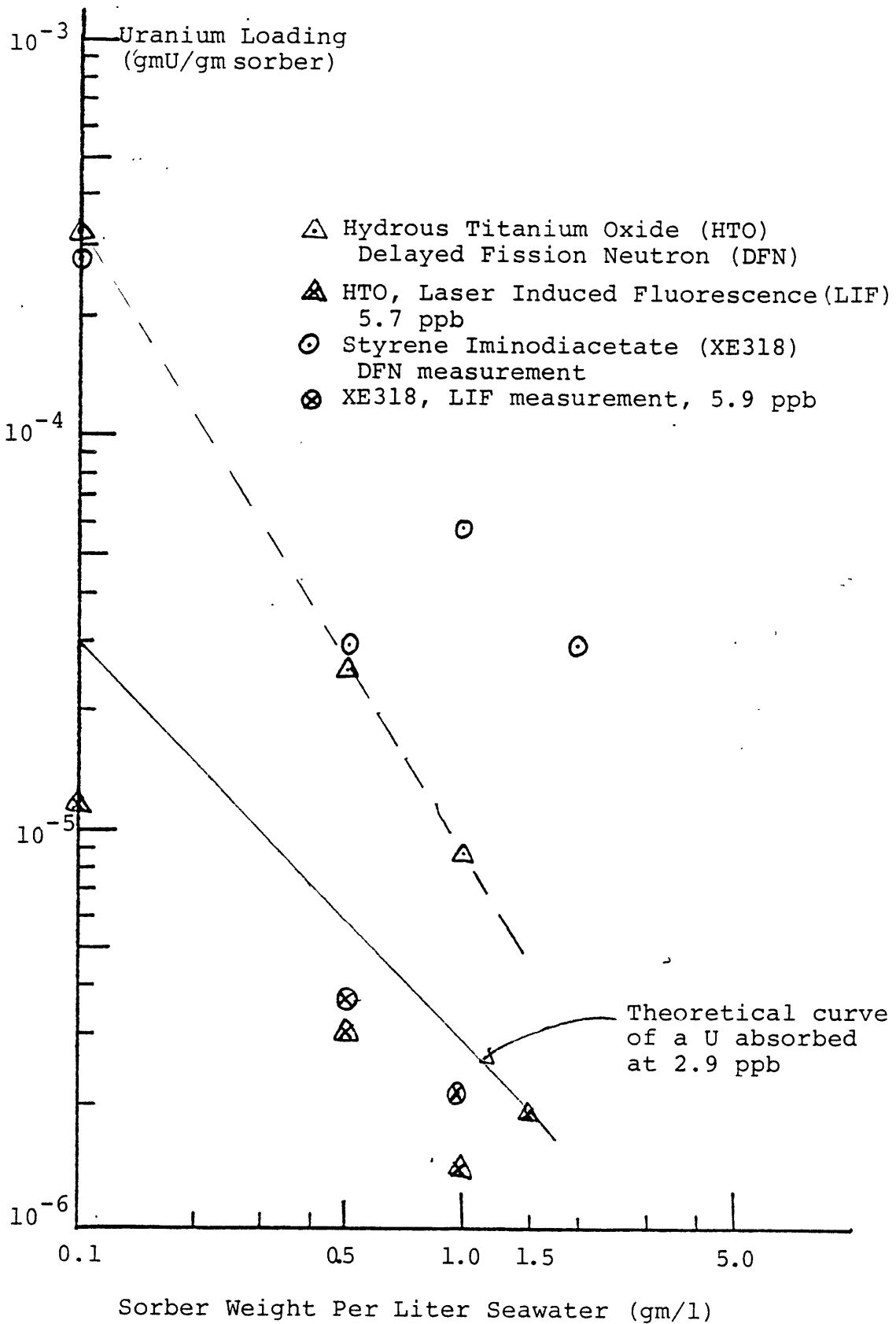
Fig. 4.1 Equilibrium Experiment: Uranium Loading versus Sorber Weight per Liter Seawater (2.9 ppb) for HTO and XE318.
