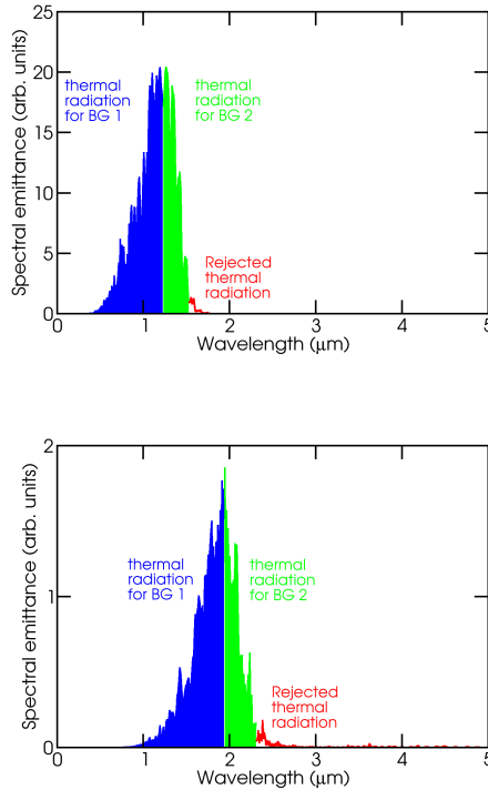
Fig. 15. Optimized emittance spectra for emitters at 2360 K (left) and 1000 K (right). The corresponding efficiencies are 66.3% and 44.0%, respectively.
