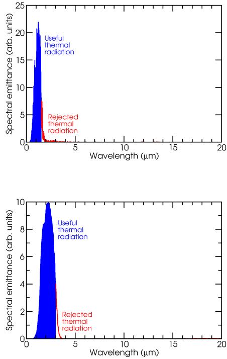
Fig. 14. Optimized emittance spectra for emitters at 2360 K (left) and 1300 K (right). The corresponding efficiencies are 54.2% and 44.7%, respectively.
