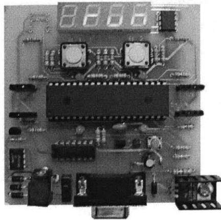
Figure 3-1: Programmable Sensing Board
