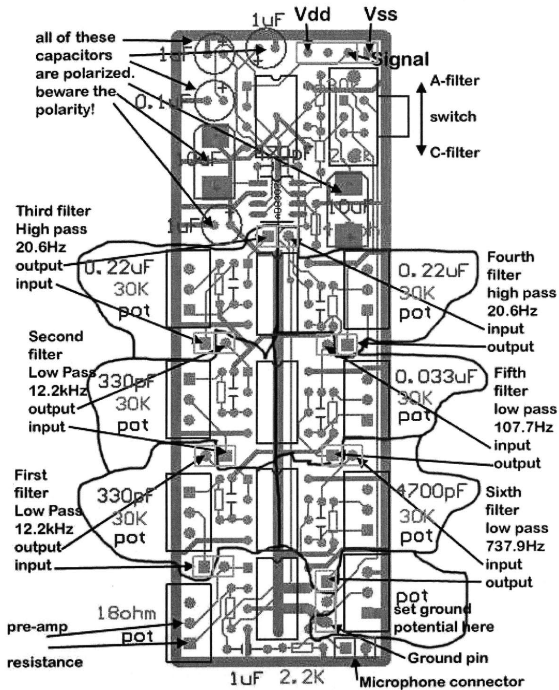
Figure C-2: Noise Sensor PCB Layout
