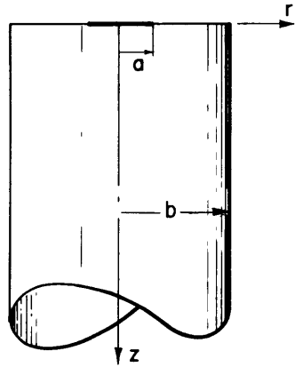
a) MODEL OF A CONTACT
