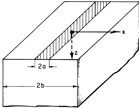
b) MACROSCOPIC HEAT CHANNEL FOR CYLINDRICAL WAVINESS IN ONE DIRECTIONS
