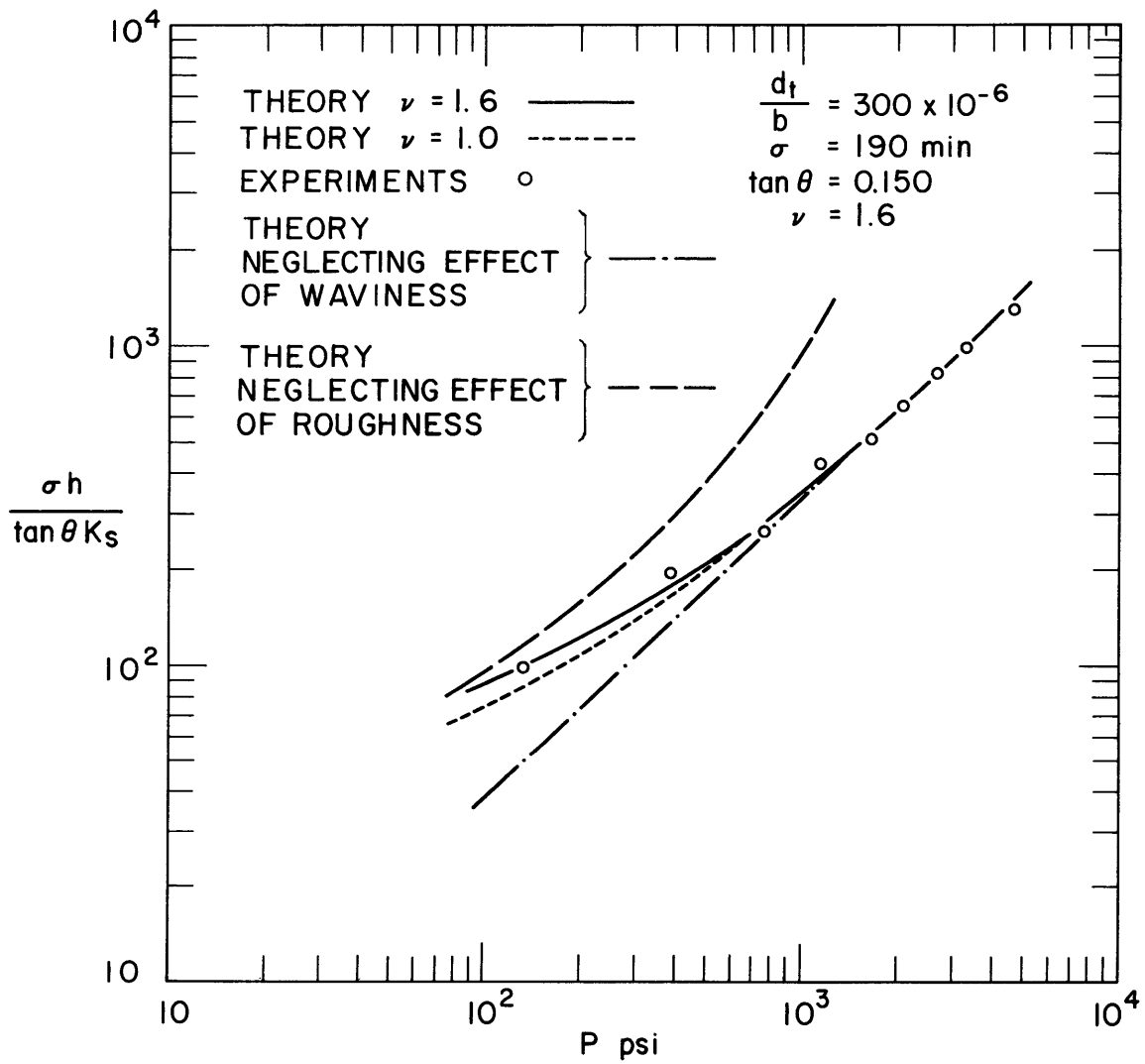
FIG. 26 CONTACT CONDUCTANCE VS. PRESSURE: STAINLESS STEEL PAIR NO. 1
