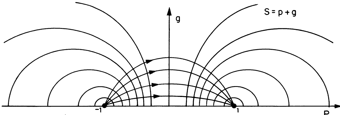
b) HEAT SOURCE AT P=-1 , HEAT SINK AT P=1
