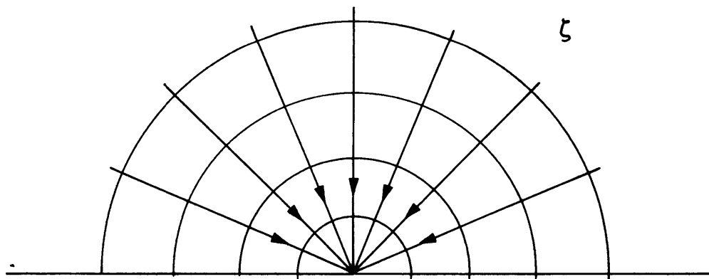
c) HEAT SOURCE AT \zeta = \infty ; HEAT SINK AT \zeta = 0
