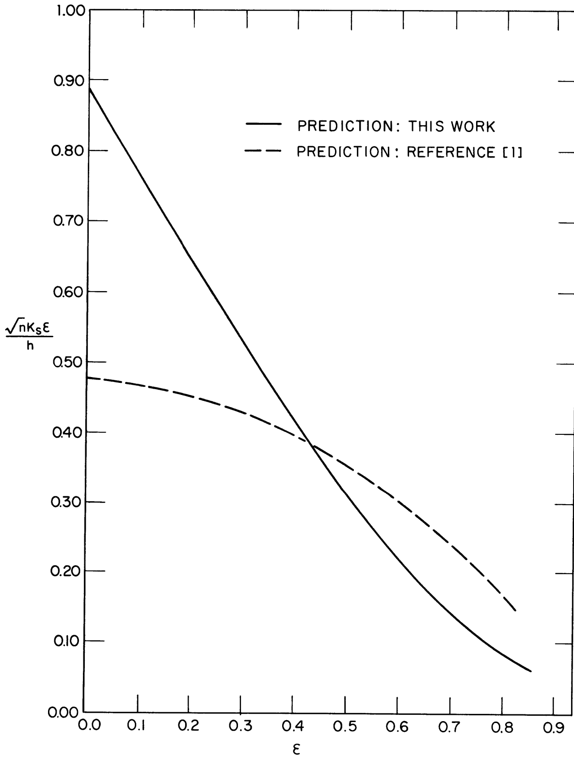
FIG. 34 COMPARISON BETWEEN THEORY OF REF. [1] AND THIS WORK
