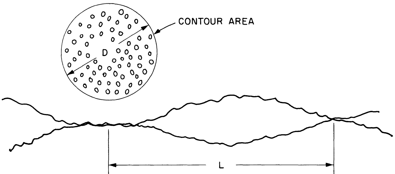
b) CONTOUR AREA (FOR CASE OF SPHERICAL WAVINESS)
