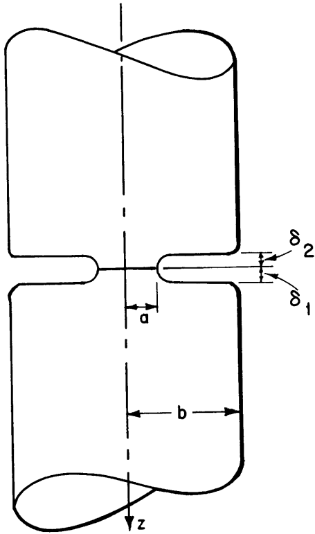
a) TYPICAL HEAT CHANNEL
