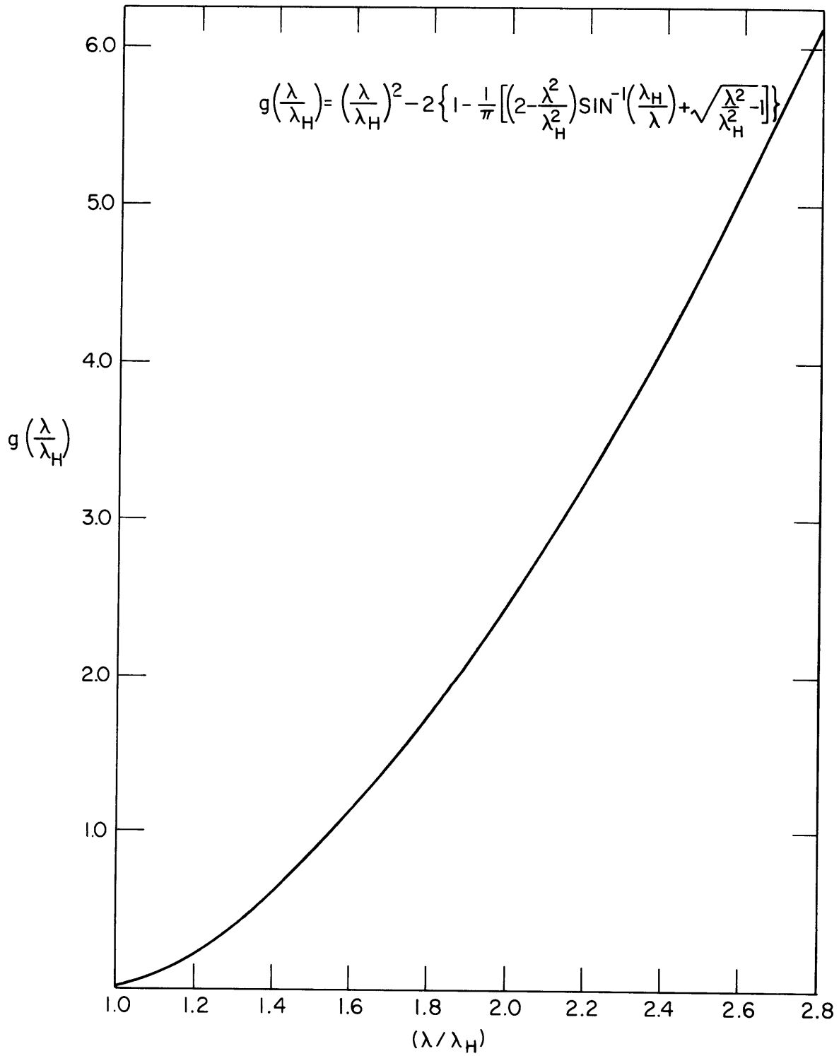
FIG. 20 WAVINESS FACTOR
