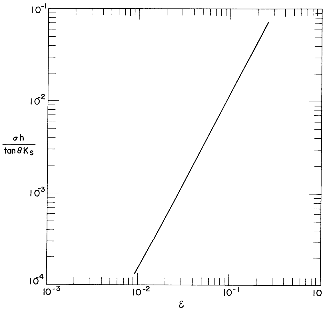
FIG. 12 THERMAL CONTACT CONDUCTANCE VS. CONTACT AREA RATIO
