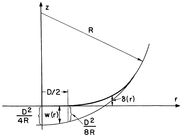
b) LOCAL DEFORMATION OF A SPHERE PRESSED AGAINST A RIGID PLANE
