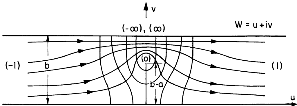
a) HEAT FLOW BETWEEN TWO PARALLEL PLANES WITH CONSTRUCTION OF FLOW AT U=0
