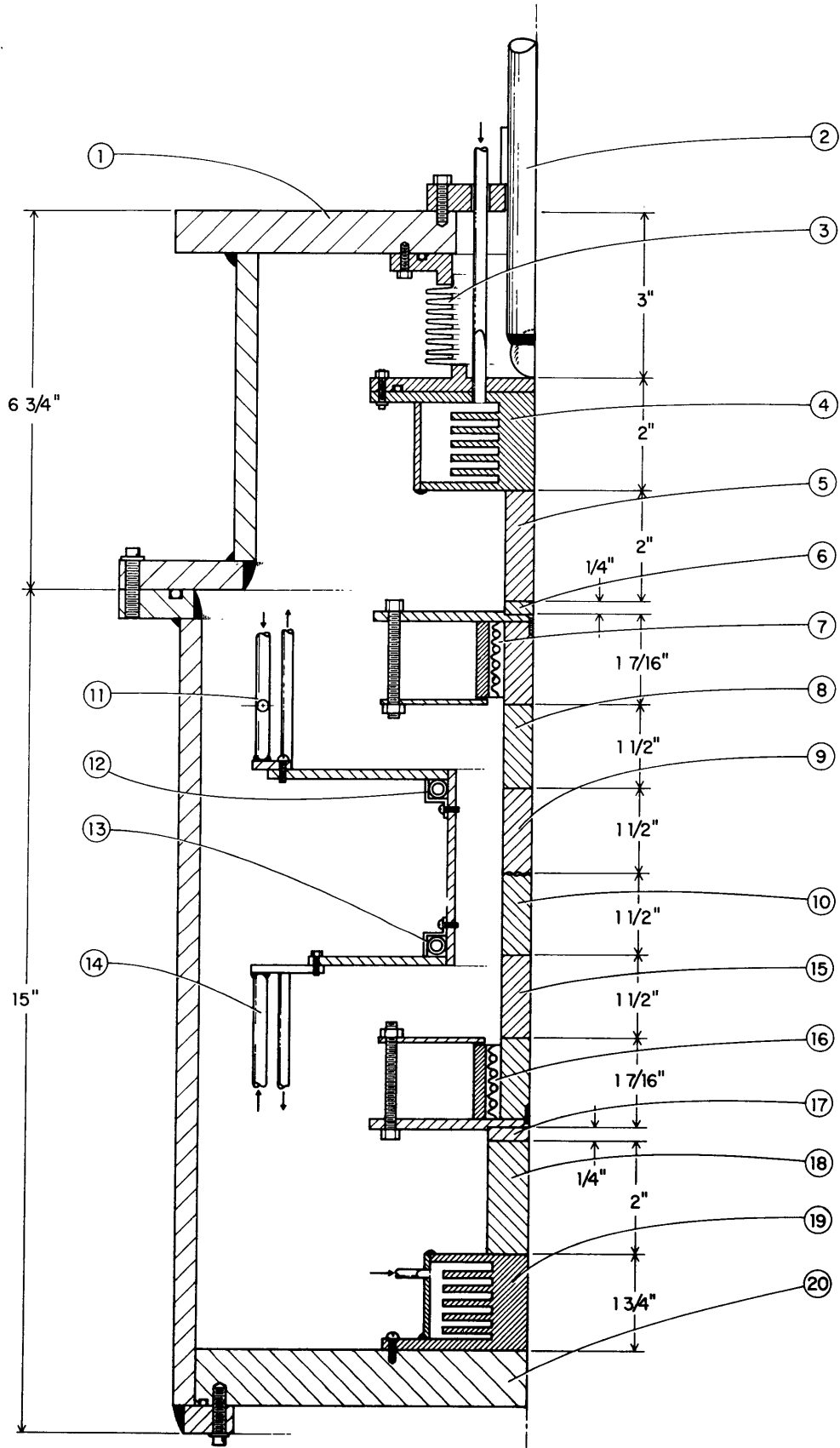
FIG. 22 TEST SECTION AND CHAMBER
