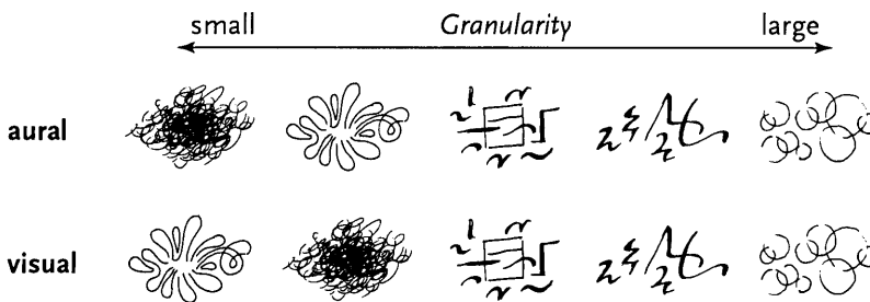
Figure 89. Granularity.
