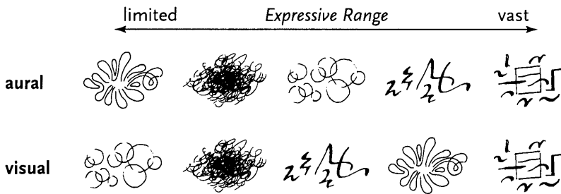
Figure 88. Expressive Range.
