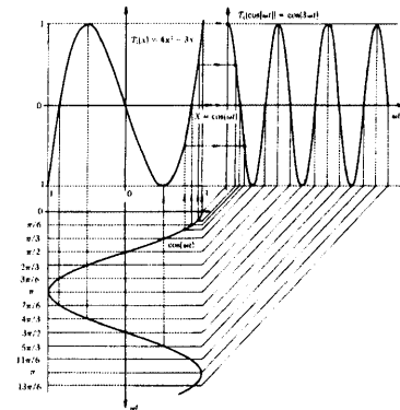
Figure 67. The waveshaping synthesis used in Warbo . A pure cosine source wave in the lower left is shaped by one of the Chebyshev shaping functions, 4x^3 - 3x , in the upper left. The final output wave is shown in the upper right.
