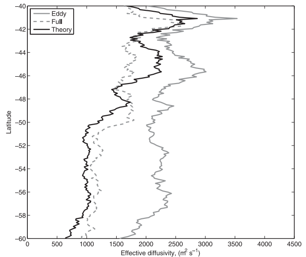
FIG. 7. Eddy diffusivity ( \text{m}^2 \text{s}^{-1} ) across mean streamlines from calculations for the full Southern Ocean: eddy diffusivity estimated from Nakamura's approach using only the geostrophic eddy velocity (solid gray) and using the full geostrophic velocity (dashed gray); theoretical prediction in (20) (solid black).
