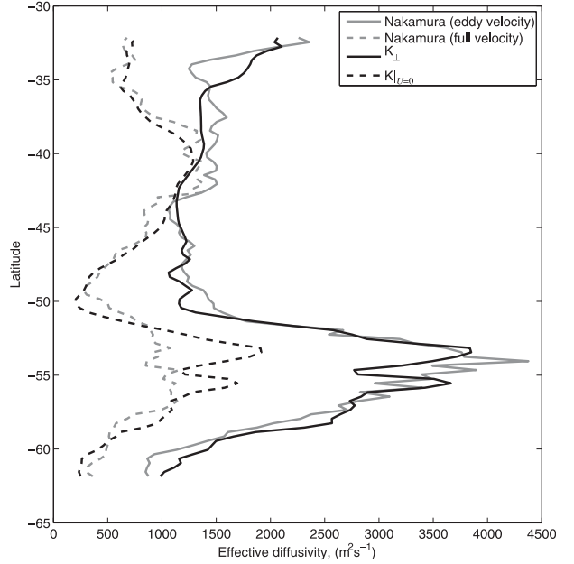
FIG. 8. Meridional eddy diffusivity ( m^2 s^{-1} ) for a path in the Pacific sector of the Southern Ocean between 125^{\circ} and 150^{\circ}W estimated directly from altimetric observations: eddy diffusivity estimated from Nakamura’s approach using only the geostrophic eddy velocity (solid gray) and using the full geostrophic velocity (dashed gray); theoretical prediction in (19) in the absence of mean flow (solid black) and with the mean flow (dashed black).
