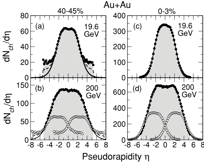
FIG. 22. Illustration of the methods used for estimating the total number of charged particles from the measured dN_{\text{ch}}/d\eta versus \eta (solid points) distributions. The solid curve represents a fit to the data within the region -y_{\text{beam}} < \eta < y_{\text{beam}} using the functional form of Eq. (14). The open circles and the shaded regions are explained in the text.
