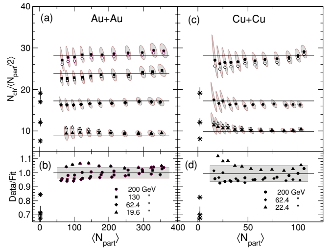
FIG. 27. (Color online) Two estimates of the total charged-particle multiplicity per participant pair, 2N_{\text{ch}}|_{|\eta| < 5.4} / \langle N_{\text{part}} \rangle (open points) and 2N_{\text{ch}}^p / \langle N_{\text{part}} \rangle (solid points), are shown as a function of centrality for each energy for Au + Au (a) and Cu + Cu (c) collisions. Horizontal lines represent centrality-independent levels predicted by Eq. (17). The lower panels show the ratio of data to the Eq. (17) prediction. The solid line is the average of all data points and the gray-shaded area the 1\sigma standard deviation. Corresponding data for p\bar{p}/pp collisions are shown as stars, see Figs. 24 and 25 for details.
