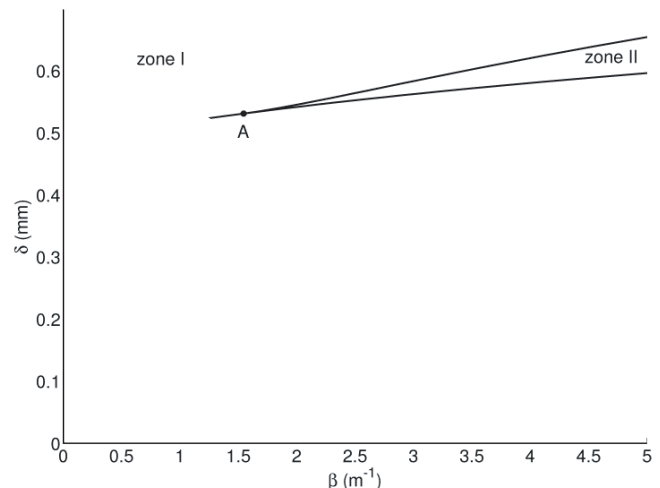
Fig. 7: Calculated stability diagram of wetting drops of volume \Omega = 3 \text{ mm}^3 in a trumpet-shaped tube of inner radius a(z) = \delta + \alpha z + \beta z^2 , with \alpha = 1.5^\circ , and inclined at 30^\circ relative to the horizontal. In zone III, the drop climbs. In zone I, it slides downwards. A stable-equilibrium position only arises in zone II. Note that the zone of stability is diminished relative to that evident in fig. 5 (obtained for \alpha = 0 ): to the left of point A, no stable-equilibrium height exists.
