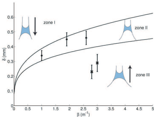
Fig. 5: (Colour on-line) Stability diagram of wetting drops of volume \Omega = 3 \text{ mm}^3 placed in a trumpet-shaped tube of inner radius a(z) = \delta + z^2 inclined at an angle 30^\circ relative to the horizontal. In zone III, the drop always climbs, propelled upwards by the capillary force arising from the large splay of the tube. In zone I, the drop slides downward: owing to relatively wide aperture \delta , the weight dominates the capillary force. A stable equilibrium is only possible in zone II. We include in the figure examples of our experimental parameters, and indicate whether drops stopped in the tube (dots), or rose to the top (crosses).
