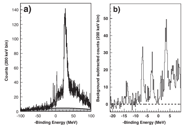
FIG. 2. The {}^{16}_{\Lambda}\text{N} binding-energy spectrum obtained after kaon selection with aerogel detectors and RICH. The electron-kaon random-coincidence contribution evaluated in a large timing window is superimposed on the spectrum in the left panel. The right panel shows the spectrum after this background has been subtracted.
