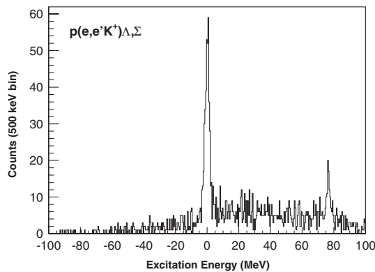
FIG. 1. Excitation energy spectrum of the p(e, e'K^+)\Lambda, \Sigma^0 on hydrogen, used for energy scale calibration. The fitted positions (not shown on the plot) for the peaks are -0.04 \pm 0.08 \text{ MeV} and 76.33 \pm 0.24 \text{ MeV} .
