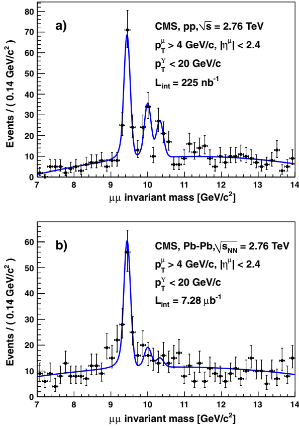
FIG. 1 (color online). Dimuon invariant-mass distributions from the pp (a) and Pb-Pb (b) data at \sqrt{s_{NN}} = 2.76 TeV. The same reconstruction algorithm and analysis criteria are applied to both data sets, including a transverse momentum requirement on single muons of p_T^\mu > 4 GeV/c. The solid lines show the result of the fit described in the text.
